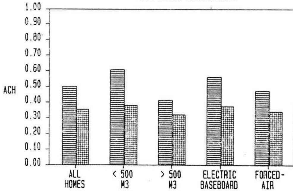
FIGURE 5. COMPARISON OF VENTILATION SYSTEM CAPACITY WITH ASHRAE REQUIREMENTS
