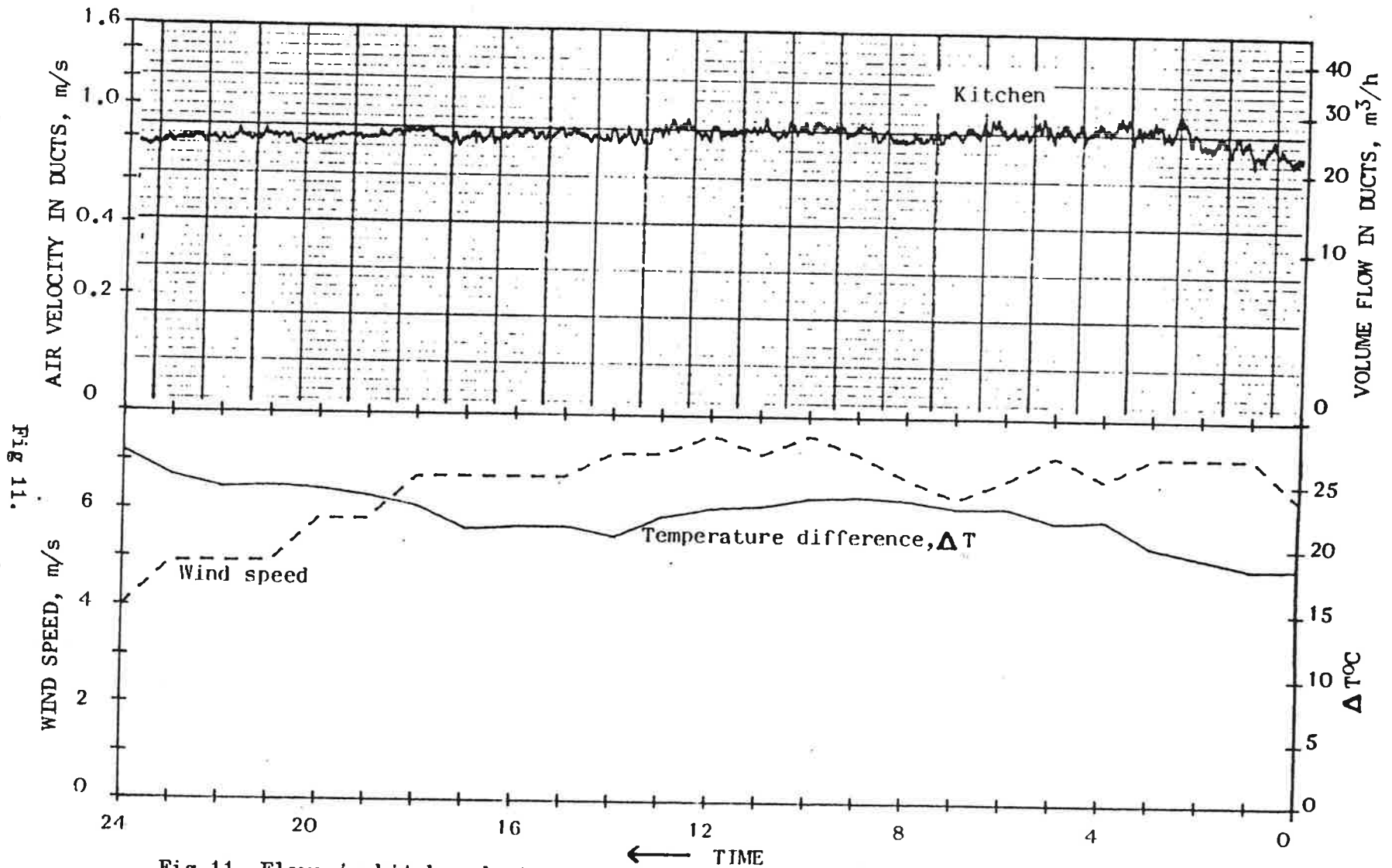
Fig 11. Flows in kitchen duct, wind speed and internal/external temperature difference ( \Delta T ), 15th February 1985.
