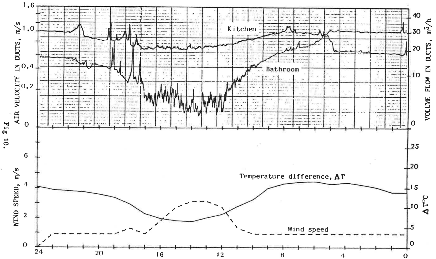
Fig 10. Flows in kitchen and bathroom ducts, wind speed and internal/external temperature difference ( \Delta T ), 12th March 1985.
