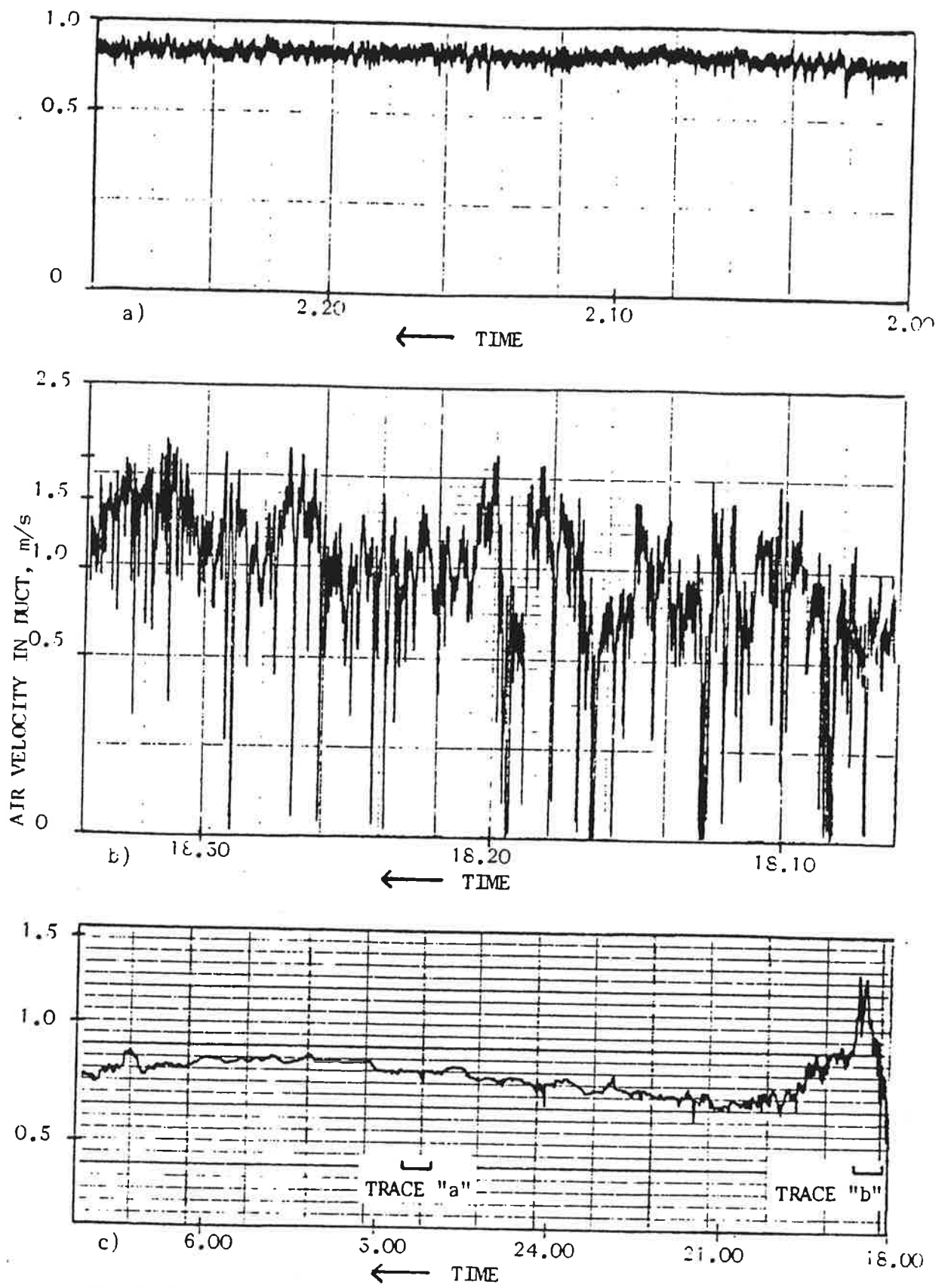
Fig 8. Typical air velocity traces (kitchen duct) a) undamped trace - steady flow b) undamped trace - irregular flow c) damped trace - including periods of traces 'a' and 'b'.
