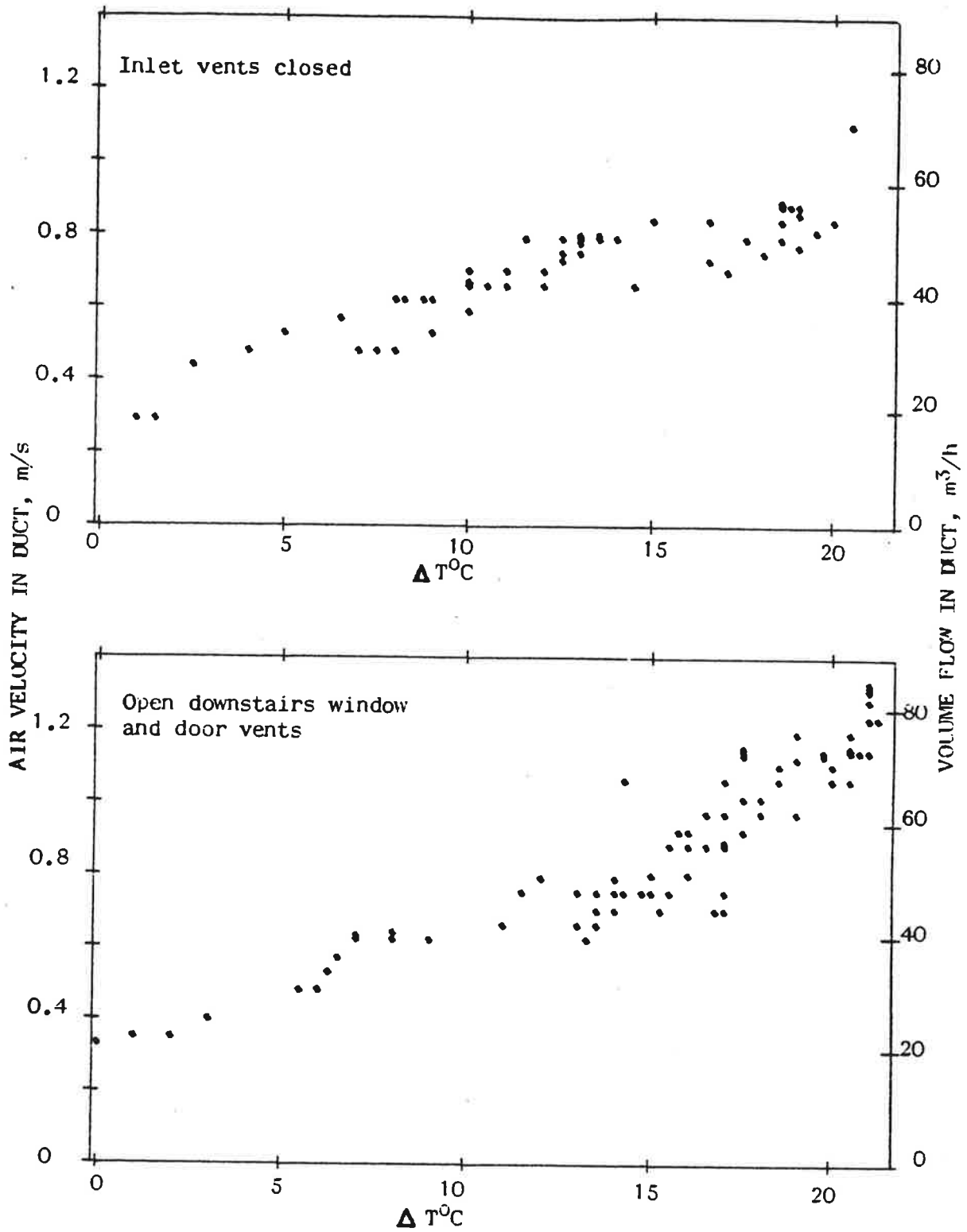
Fig 1. Flows in TRADA house kitchen duct. (House - 240m 3 ; kitchen - 20m 3 )
