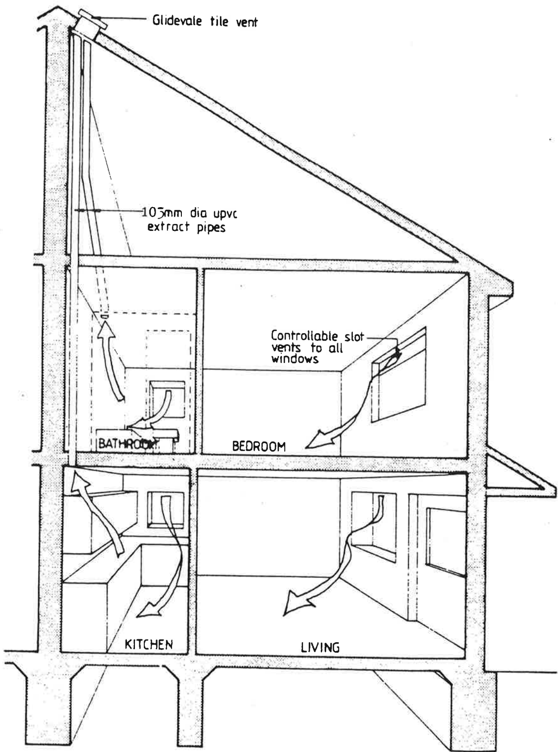
Fig 7. The ventilation system fitted in the 'Richmond' house.
