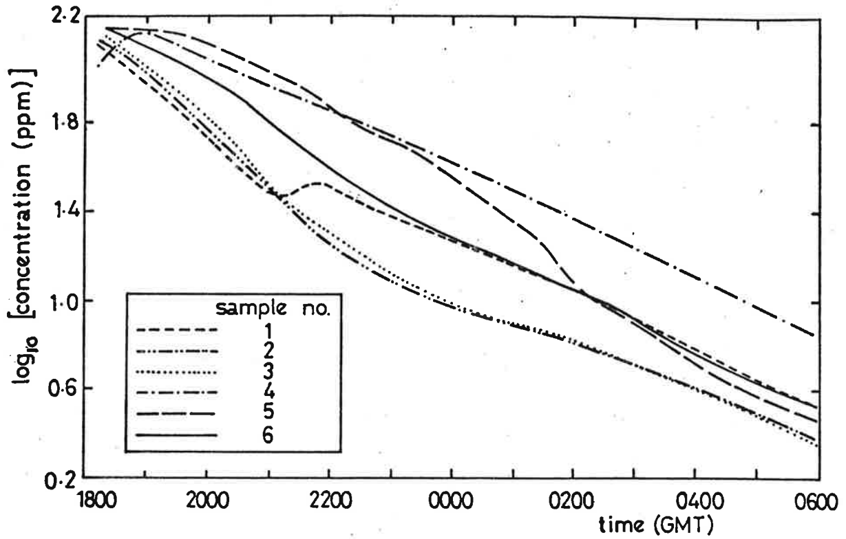
Figure 12 Concentration profiles from Test B1 in building B
