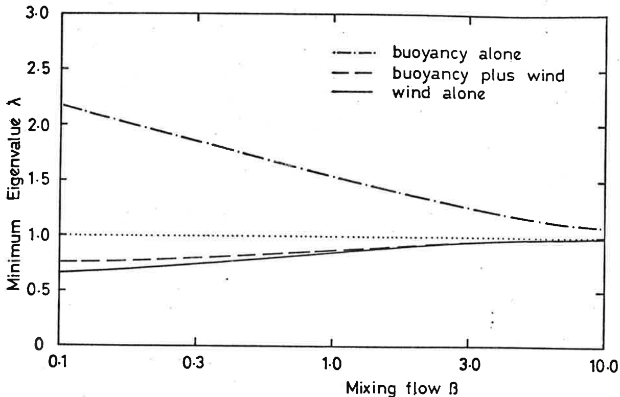
Figure 2 Variation of the dominant eigenvalue with enhanced mixing
