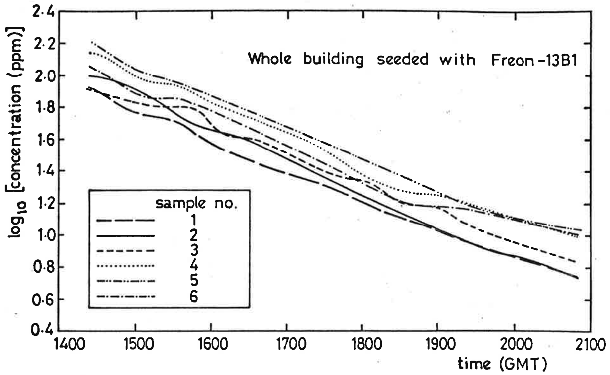
Figure 9.a Freon-13B1 concentration profiles from Test A1
