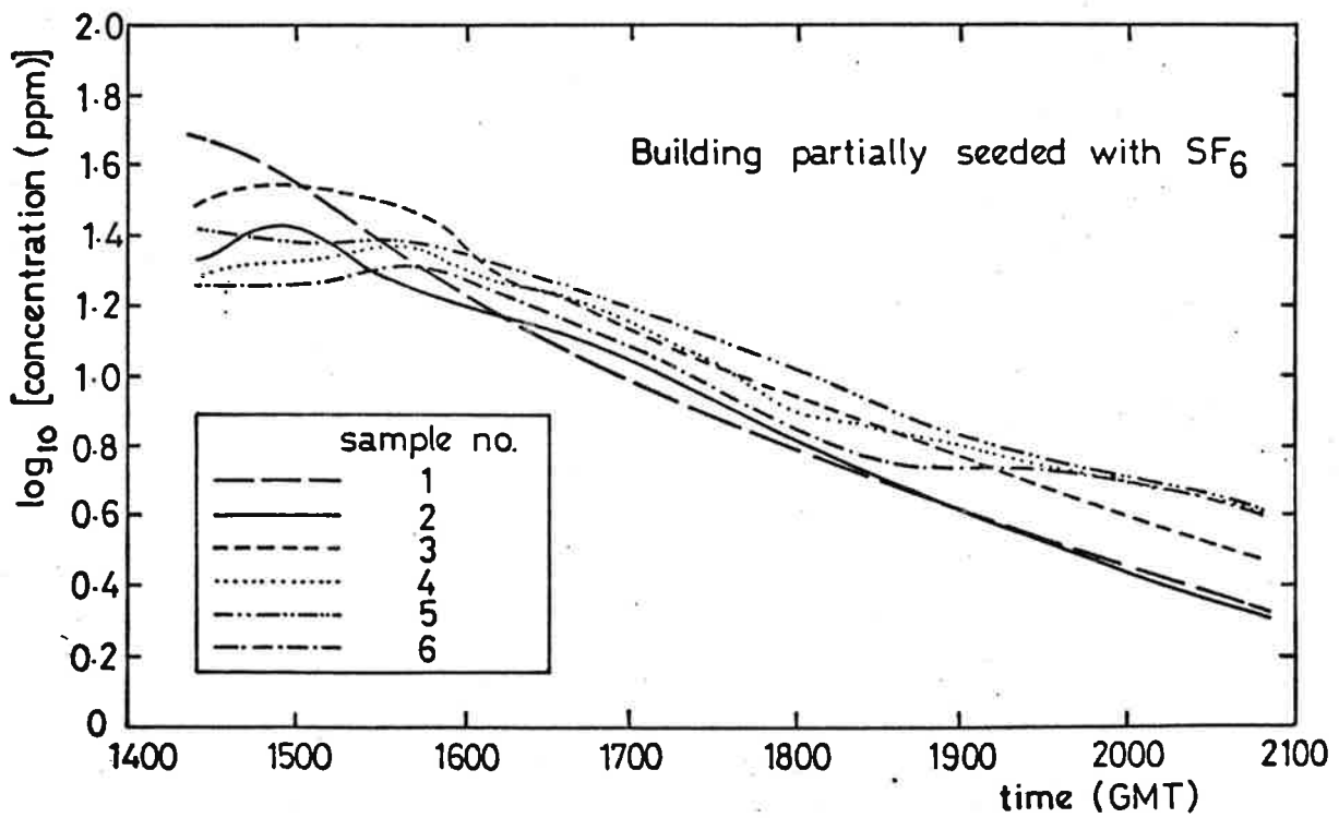
Figure 9.b SF6 concentration profiles from Test A1
