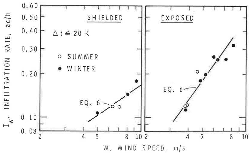
Figure 4. Wind induced air infiltration rates [2]
