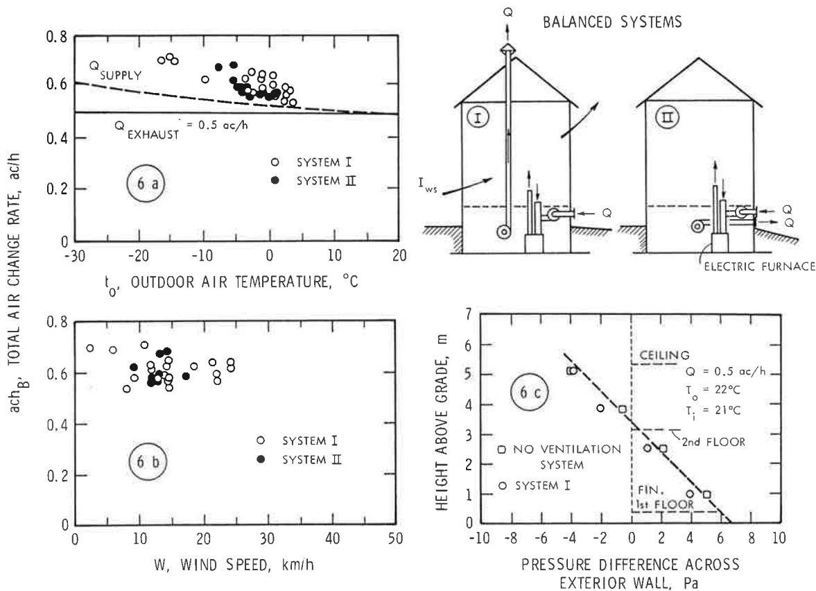
Figure 6. Total air change rate and pressure difference profile of balanced systems [4]
