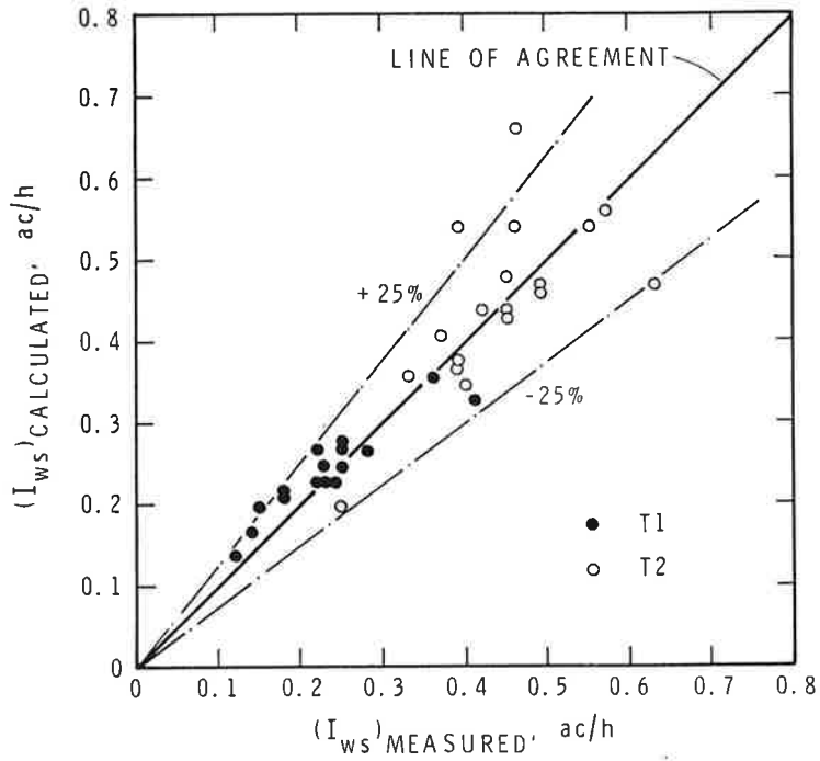
Figure 11. Comparison of calculated and measured air infiltration rates for houses T1 and T2
