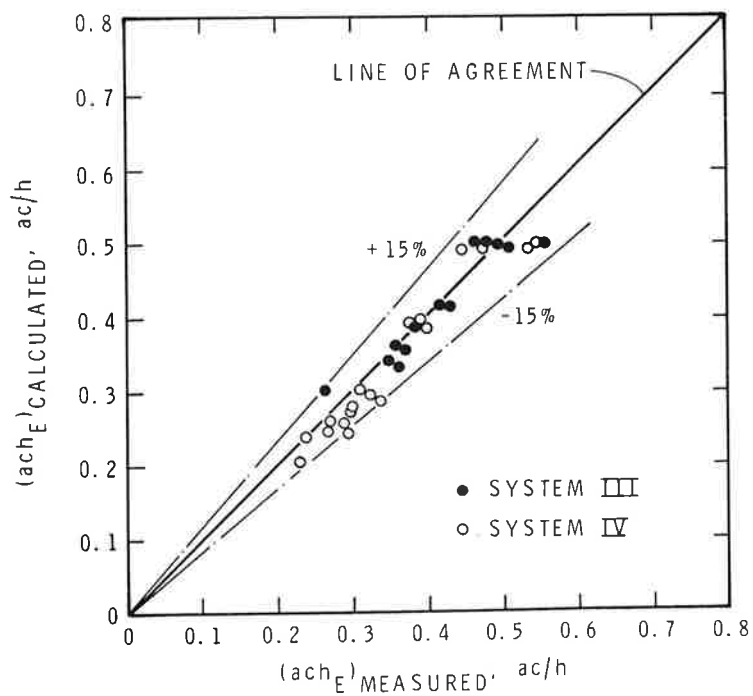
Figure 14. Comparison of calculated and measured air change rates for systems III and IV
