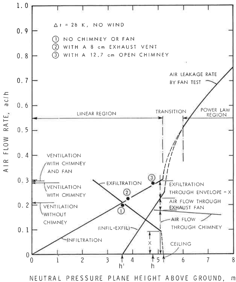
Figure 1. Supply and exhaust air flow rates versus height above ground level for a two-storey house
