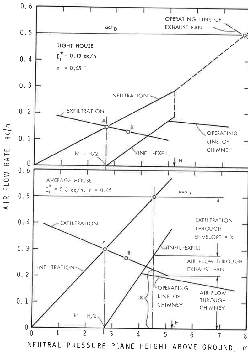
Figure 10. Air flow versus neutral pressure level diagram for selecting ventilation systems
