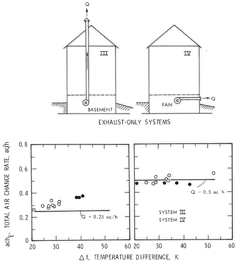
Figure 7. Total air change rate versus temperature difference for exhaust-only systems [4]
