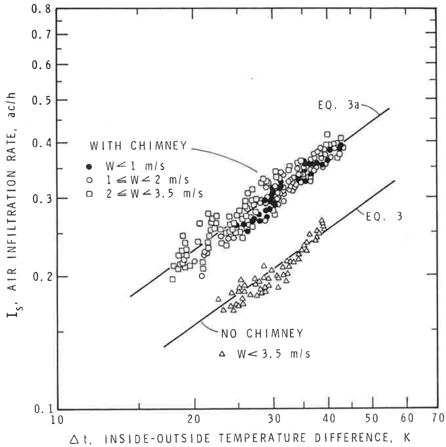
Figure 2. Air infiltration rates with and without chimney as determined by tracer gas decay method [3]
