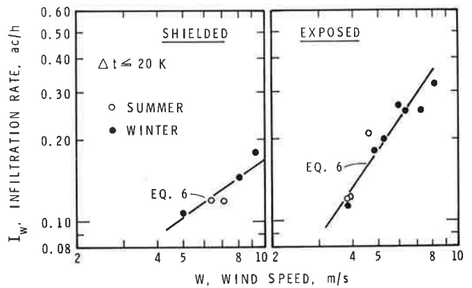
Figure 4. Wind induced air infiltration rates
