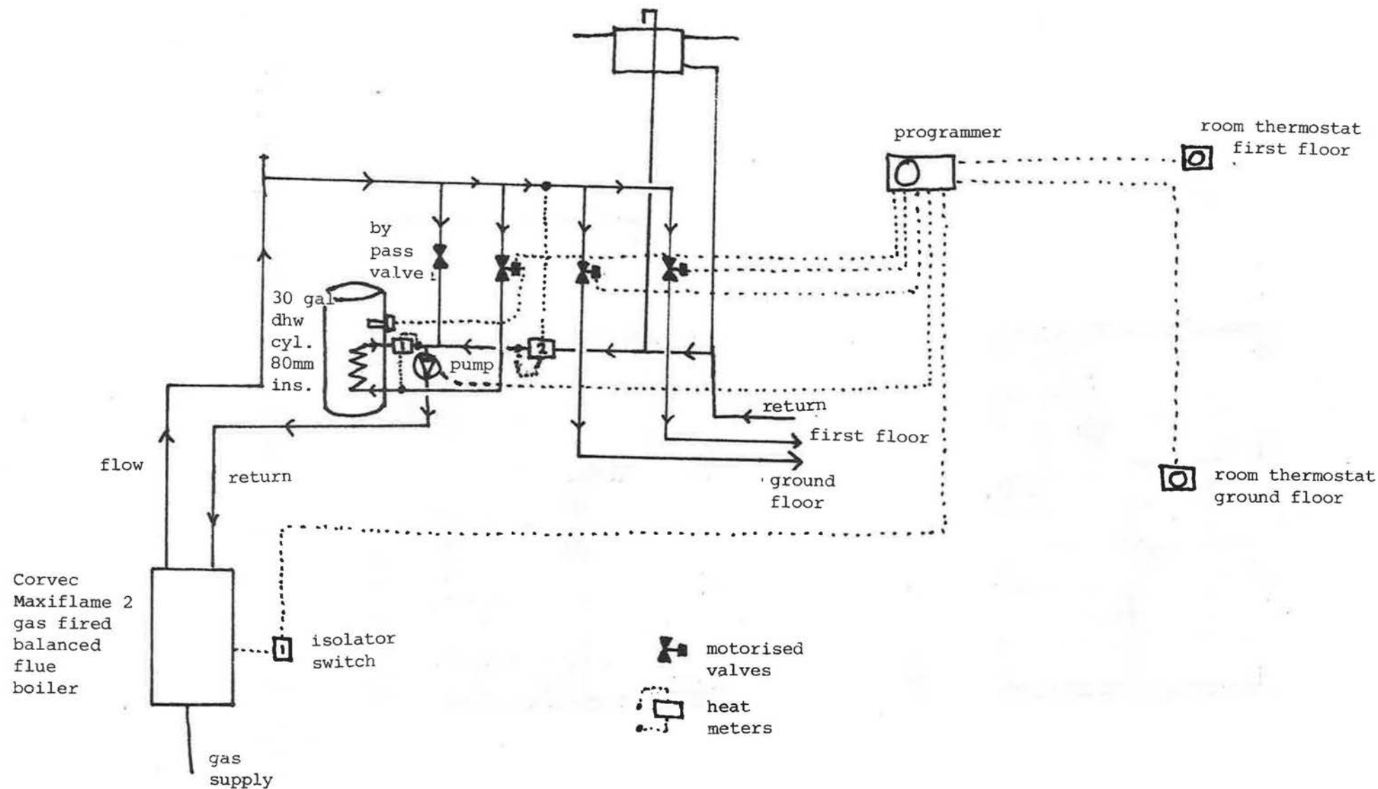
Figure 14.1 Heating system - diagrammatic
