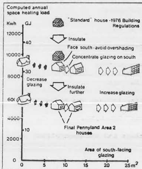
Figure S3. Pre-design modelling produced estimates of insulation and passive solar energy savings
