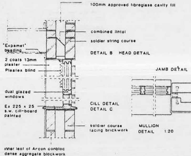
Figure S33 Insulation detailing
