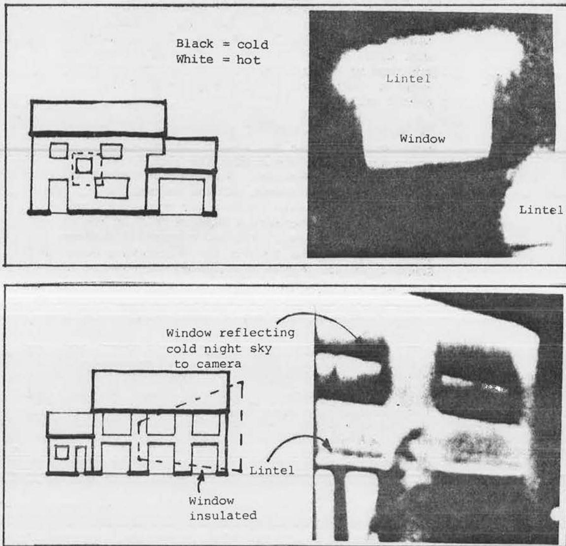
Figure S5. The thermographic survey helped to indentify specific areas of high heat loss such as the window lintels.
