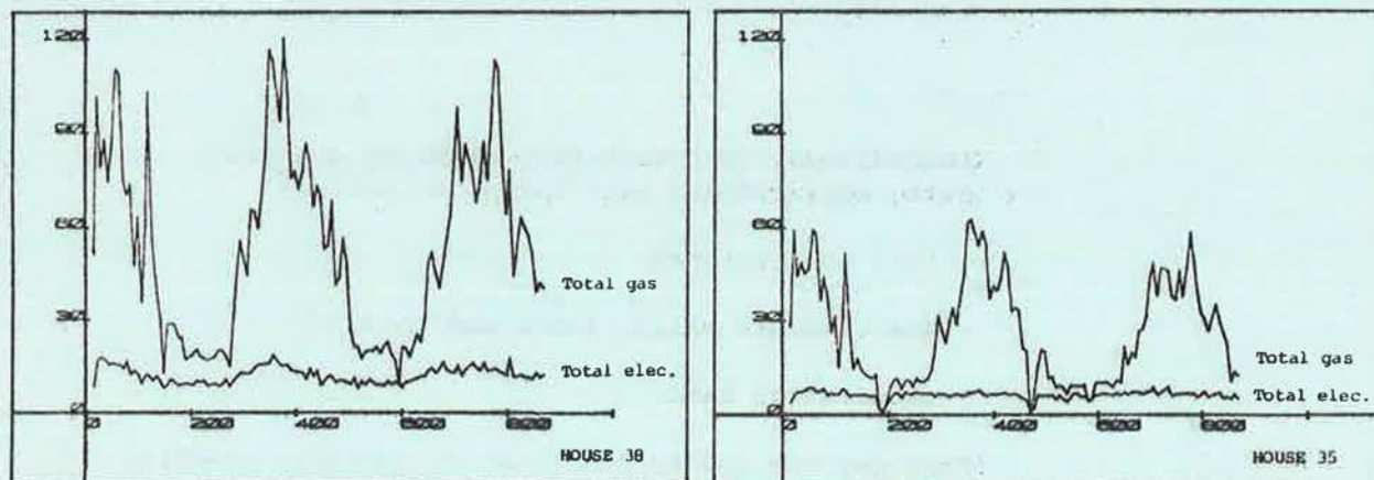
Figure S7. Gas and electricity consumption for two houses show a 2:1 difference in usage
