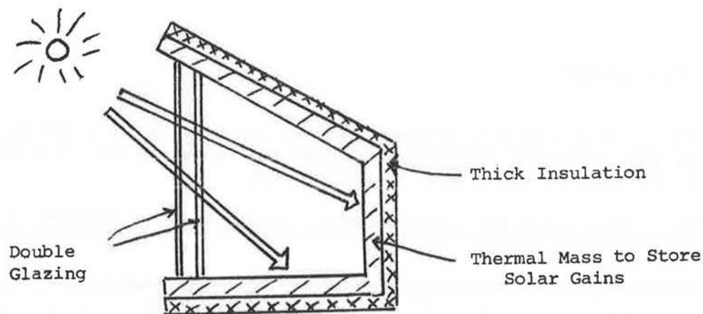
Figure 10.1 Notional Direct Gain Passive Solar House
