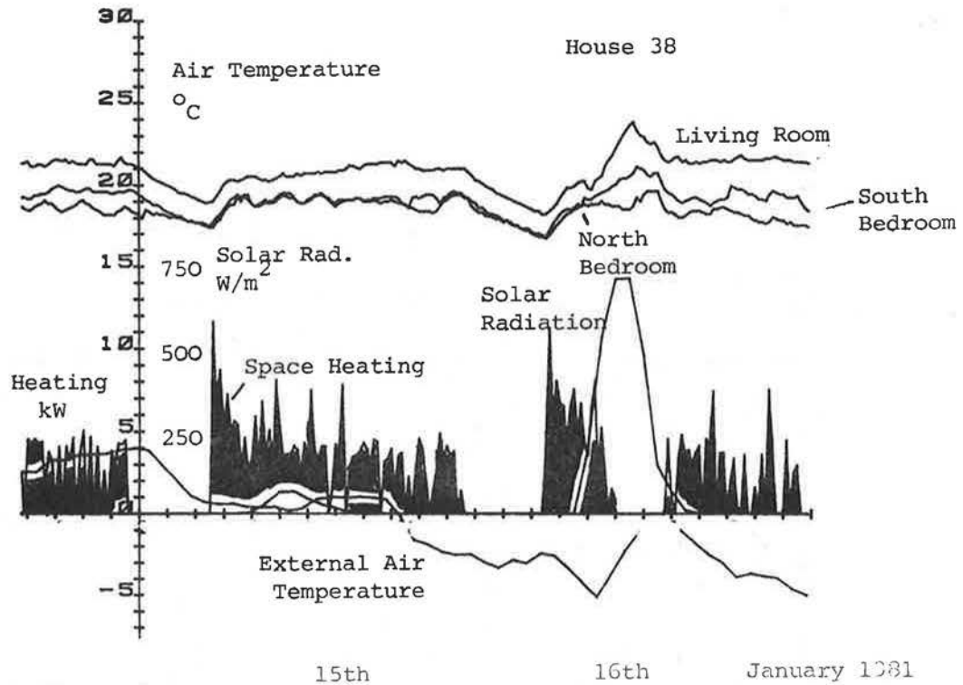
Figure 10.10 Solar Radiation and Space Heating
