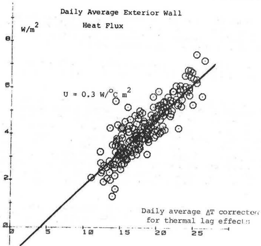
Figure 8.2. Wall U-value
