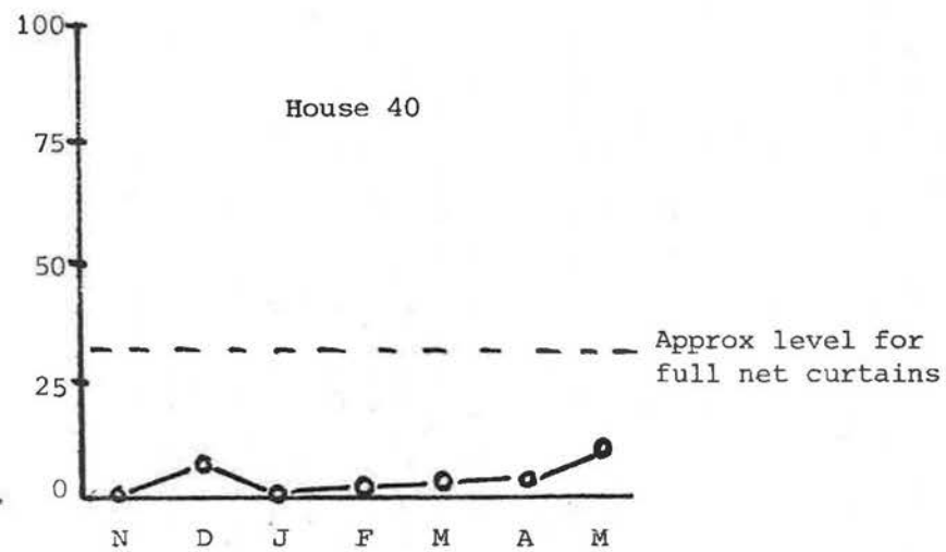
Figure 10.15 Average Percentage Obstruction of South-Facing Windows by Blinds and Curtains at 10 a.m.
