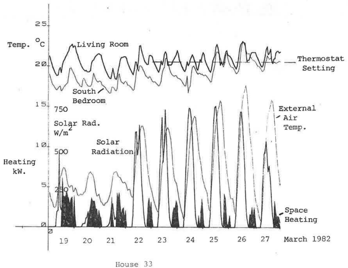
Figure 10.11 Solar Radiation and Space Heating
