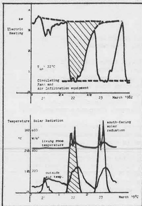
Figure S23. The effect of solar radiation on space heating and surface heat flux in the test house
