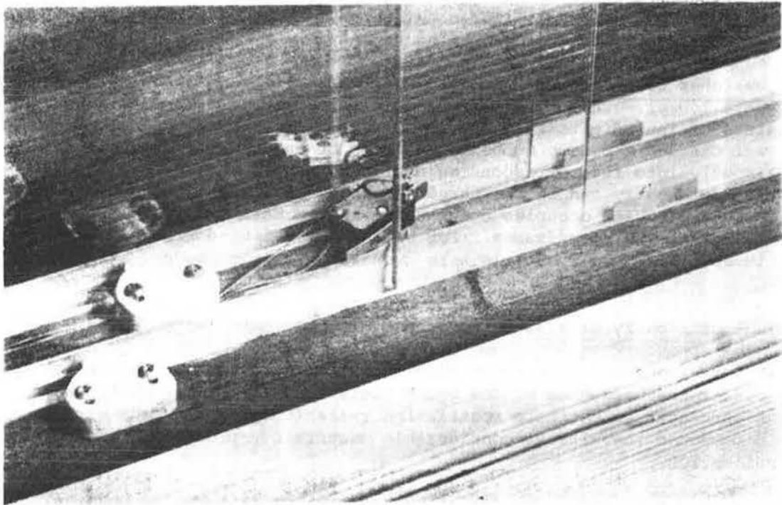
Figure 16.12 Lever action micro-switches were used to monitor window openings
