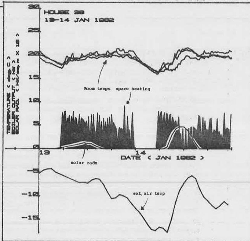
Figure S29. The radiator output was sufficient to give fast warm-up periods even in extreme outside conditions
