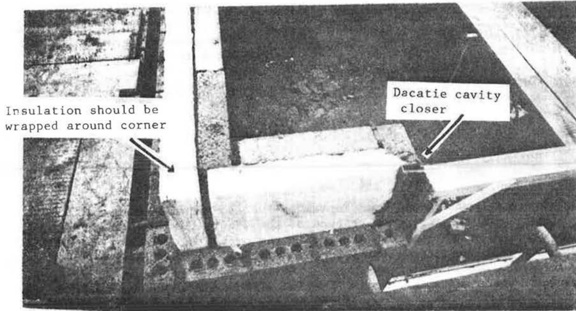
Figure 4.2 Wall insulation
