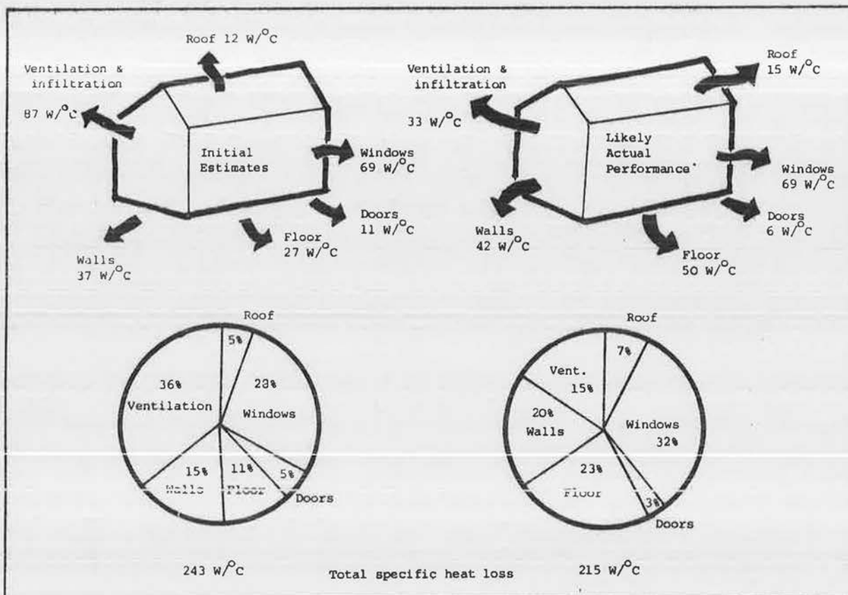
Figure S13. The total specific heat loss was as expected but the floor and ventilation components showed a considerable discrepancy
