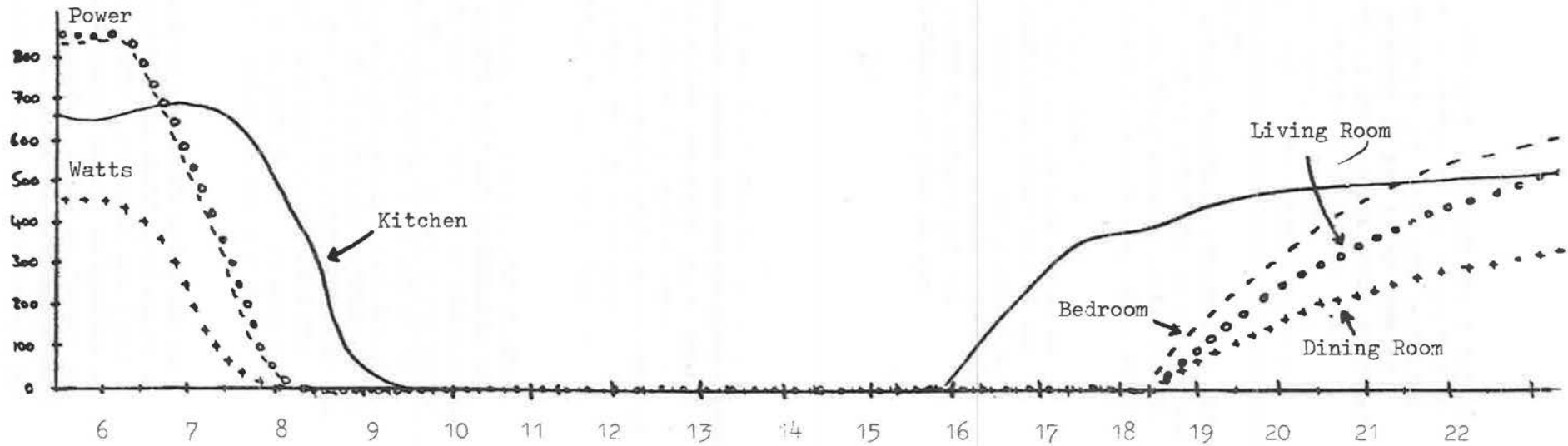
Figure 10.7 Heating Power Traces, 5th March 1982. CLEAR SKY SUNNY DAY
