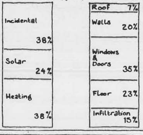
Figure S19 Heat gains balance heat losses
