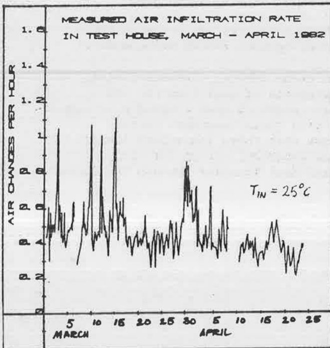
Figure S15. Infiltration rates were surprisingly low
