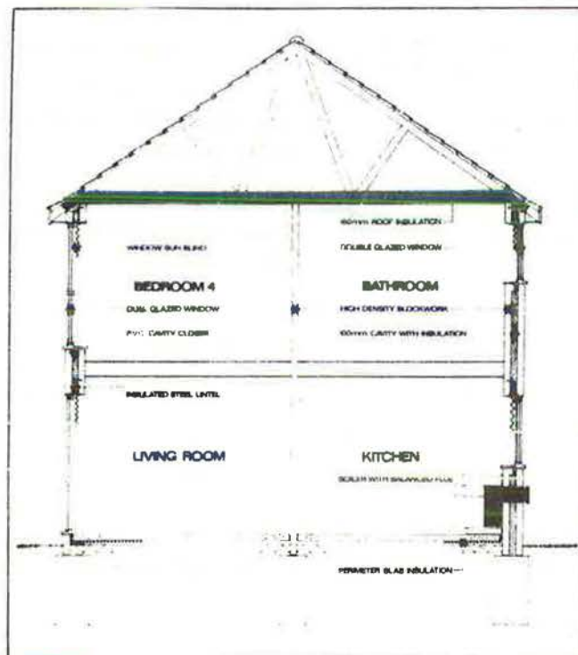
Figure 3.4 House section
