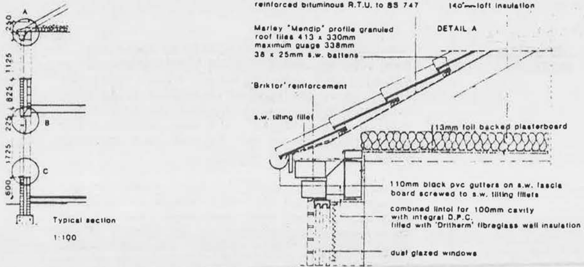
Figure S33 Insulation detailing
