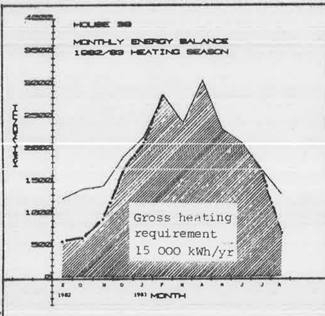
Figure S16. The gross heating requirement of 15,000 kWh/yr is about 10,000 kWh/yr less than house built to 1982 Building Regulations
