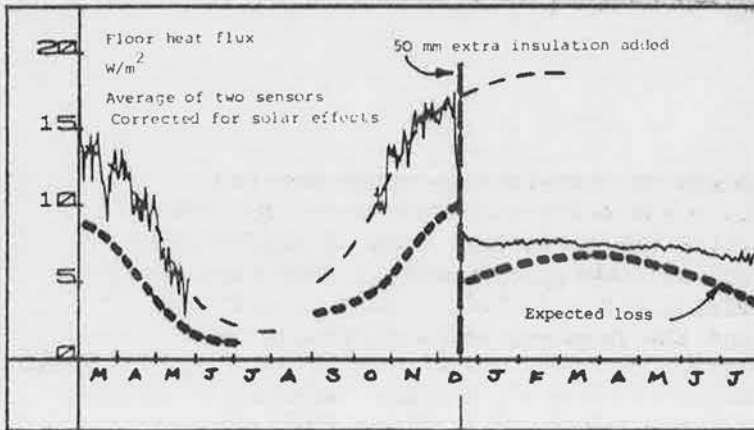
Figure S14. Floor heat losses twice as high as expected
