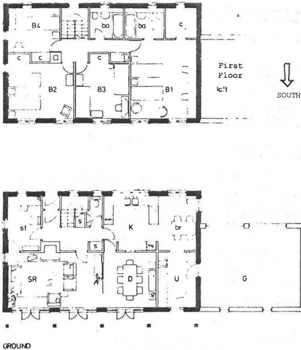
Figure 2.12 Woughton 'D' floor plans
