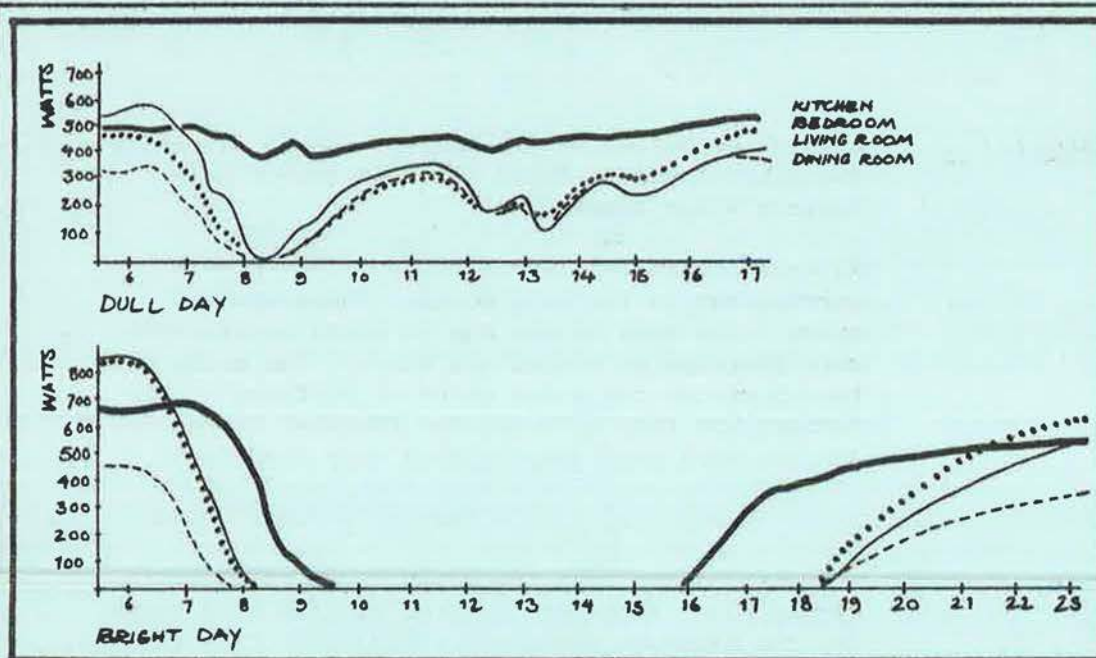
Figure S24. Power traces of room heaters during dull and sunny weather show solar gains displacing auxiliary heating
