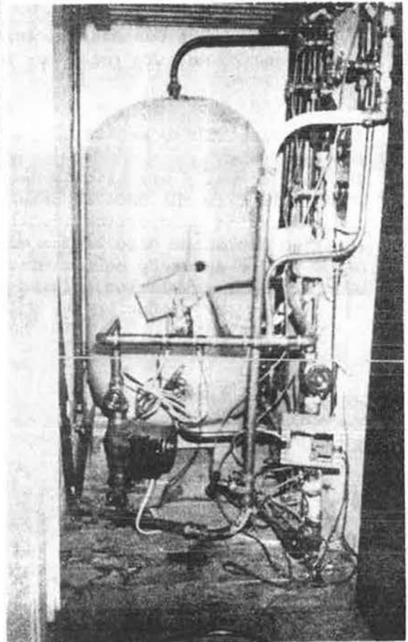
Figure 16.8 Two heat meters installed in an airing cupboard, one for space heating (right) and one for domestic hot water (in front of cylinder, angled).
