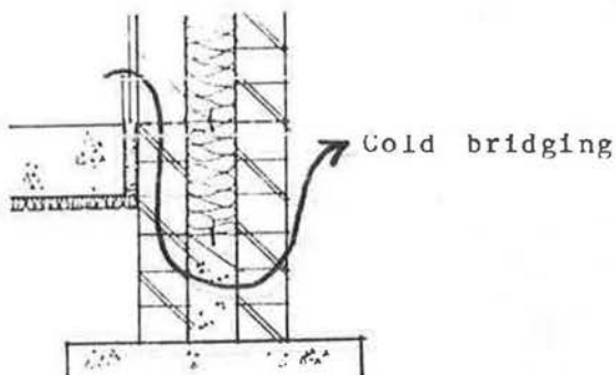
Figure 4.3 Wall insulation base detail
