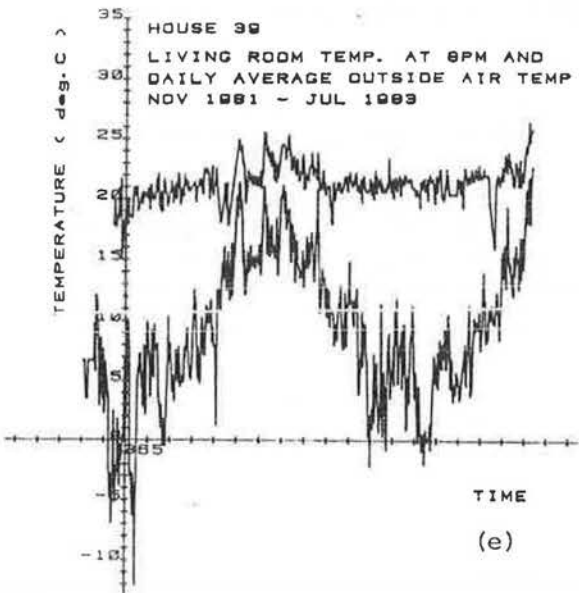
Figure 13.2 Living room temperatures at 8 p.m.
