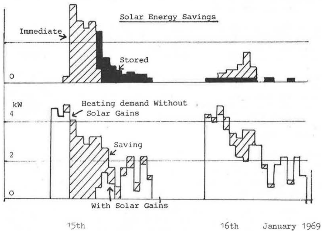
Figure 10.9 Effects of Solar Radiation on Occupied House Heating Demand
