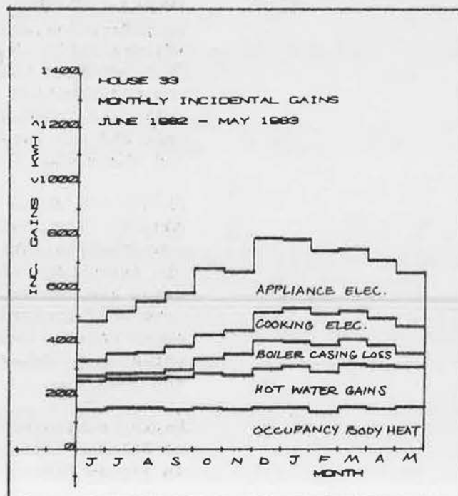
Figure S21. Incidental gains show a slight seasonal variation
