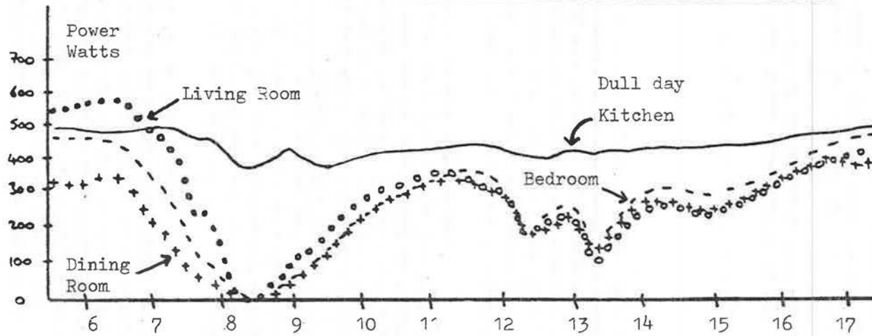
Figure 10.6 Heater Power Traces, 1st March 1982 DULL DAY
