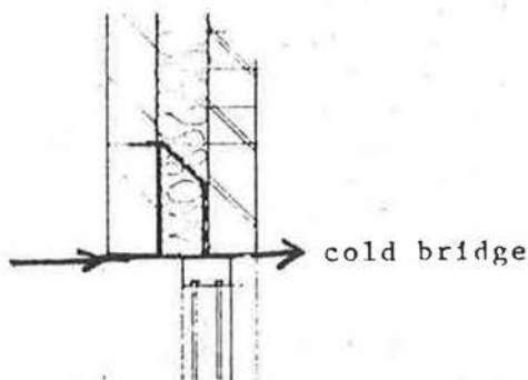
Figure 4.6 Lintel detail
