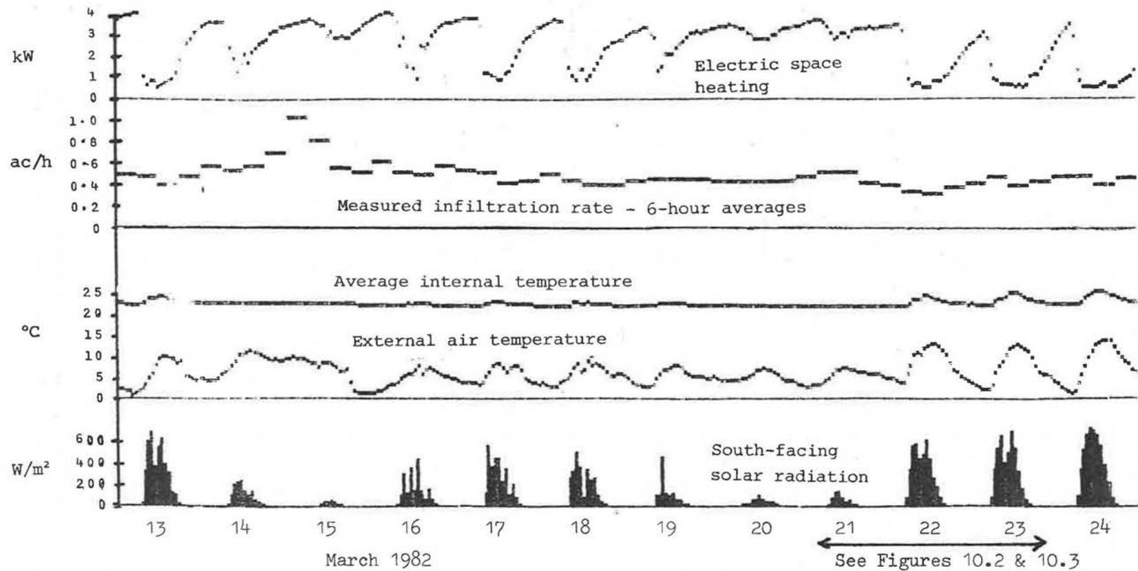
Figure 10.19 Space Heating, Infiltration, Temperatures and Solar Radiation 13.3.82 - 24.3.82
