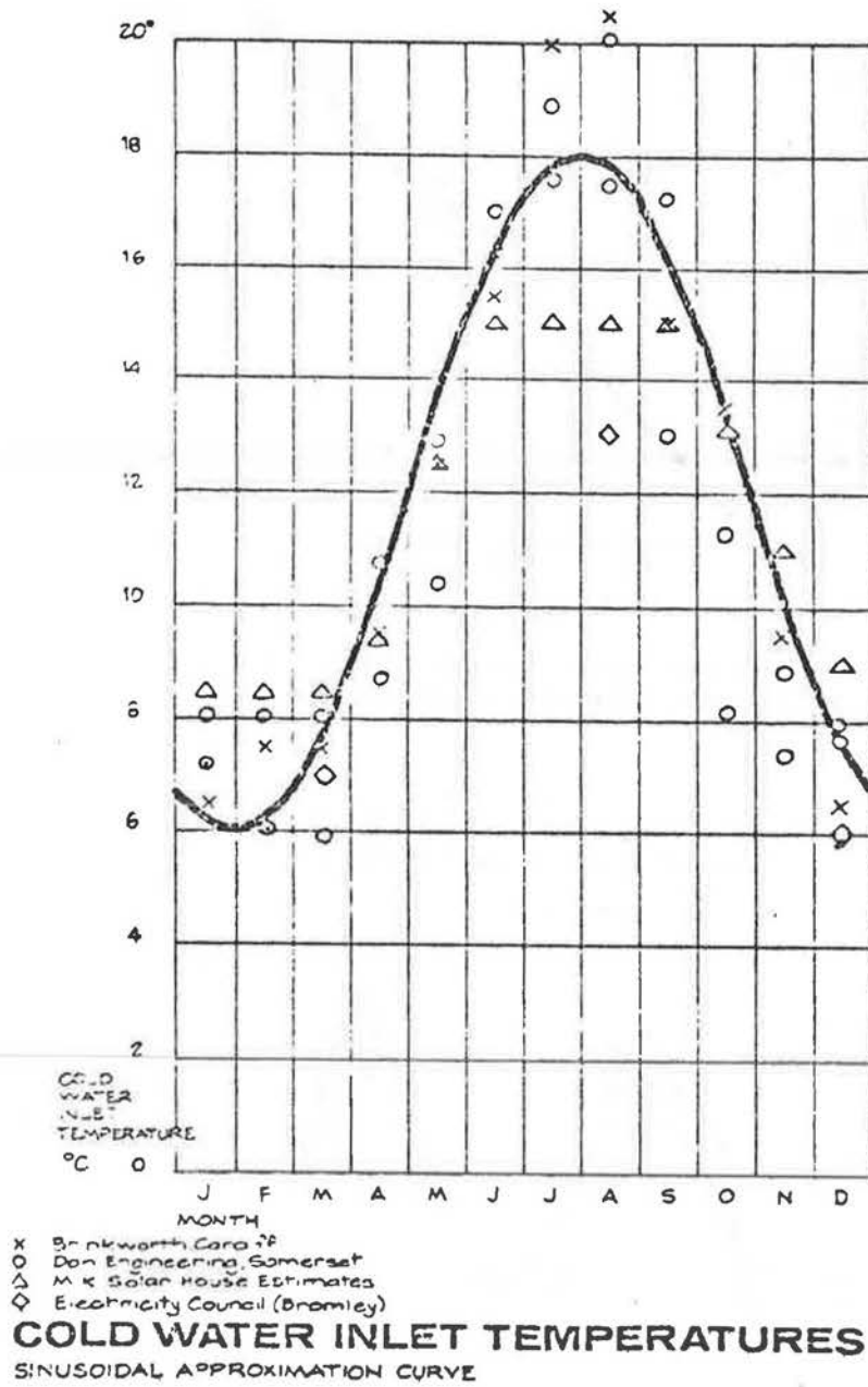
Figure 8.29 Assumed ground temperature curve used for floor loss calculations
