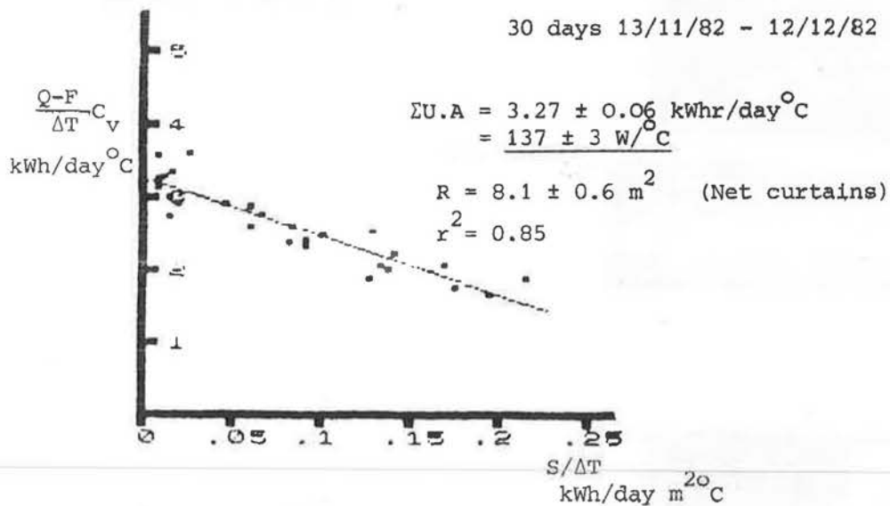
Figure 8.17 Test House Thermal Calibration
