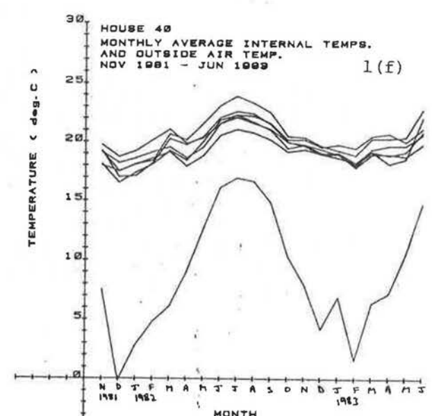
Figure 13.1 Monthly average internal room temperatures
