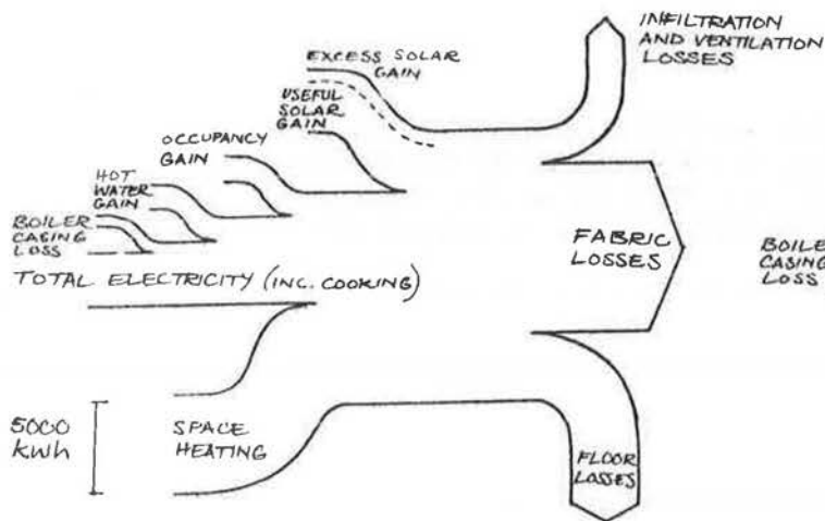
SANKEY DIAGRAM FOR HOUSE 33 SEPT - MAY
