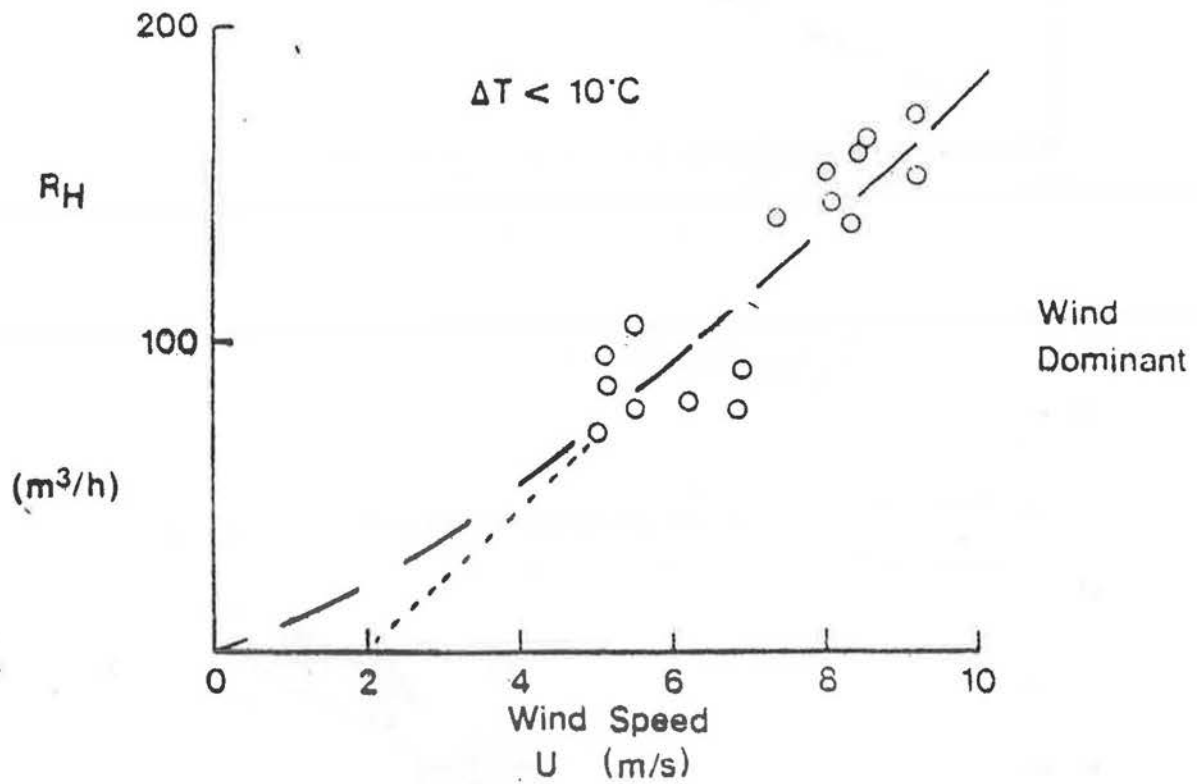
Figure A9.1.3 Determination of wind function f(u)
