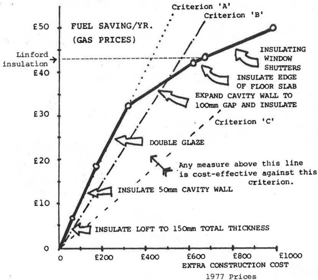
Figure 2.6 Original Design Ranking Of Insulation Measures - ref 2.12
