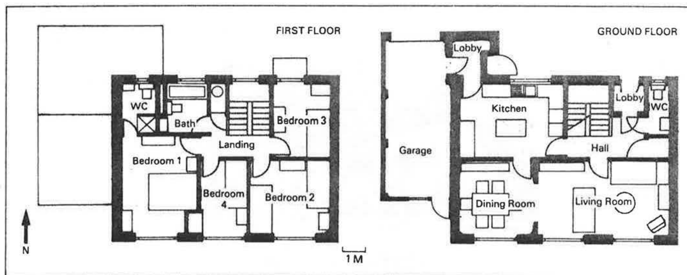
Figure 3.2 House plans
