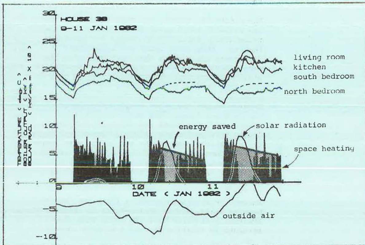
Figure S25. Solar gains clearly displace auxiliary heating in the occupied houses
