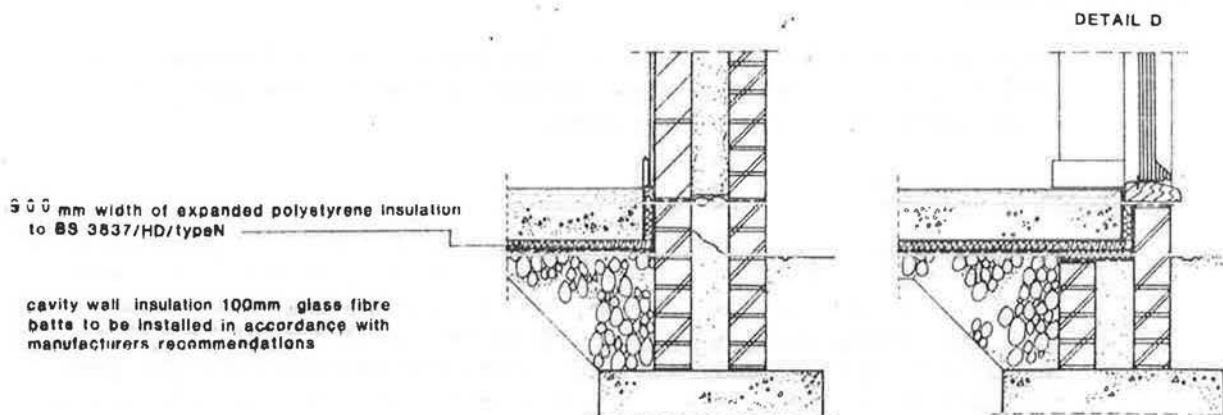
Fig. 3.5 ASSEMBLY DETAILS
