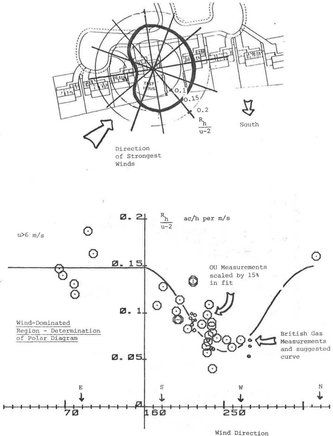
Figure A9.1.4 Sheltering effect of adjacent houses
