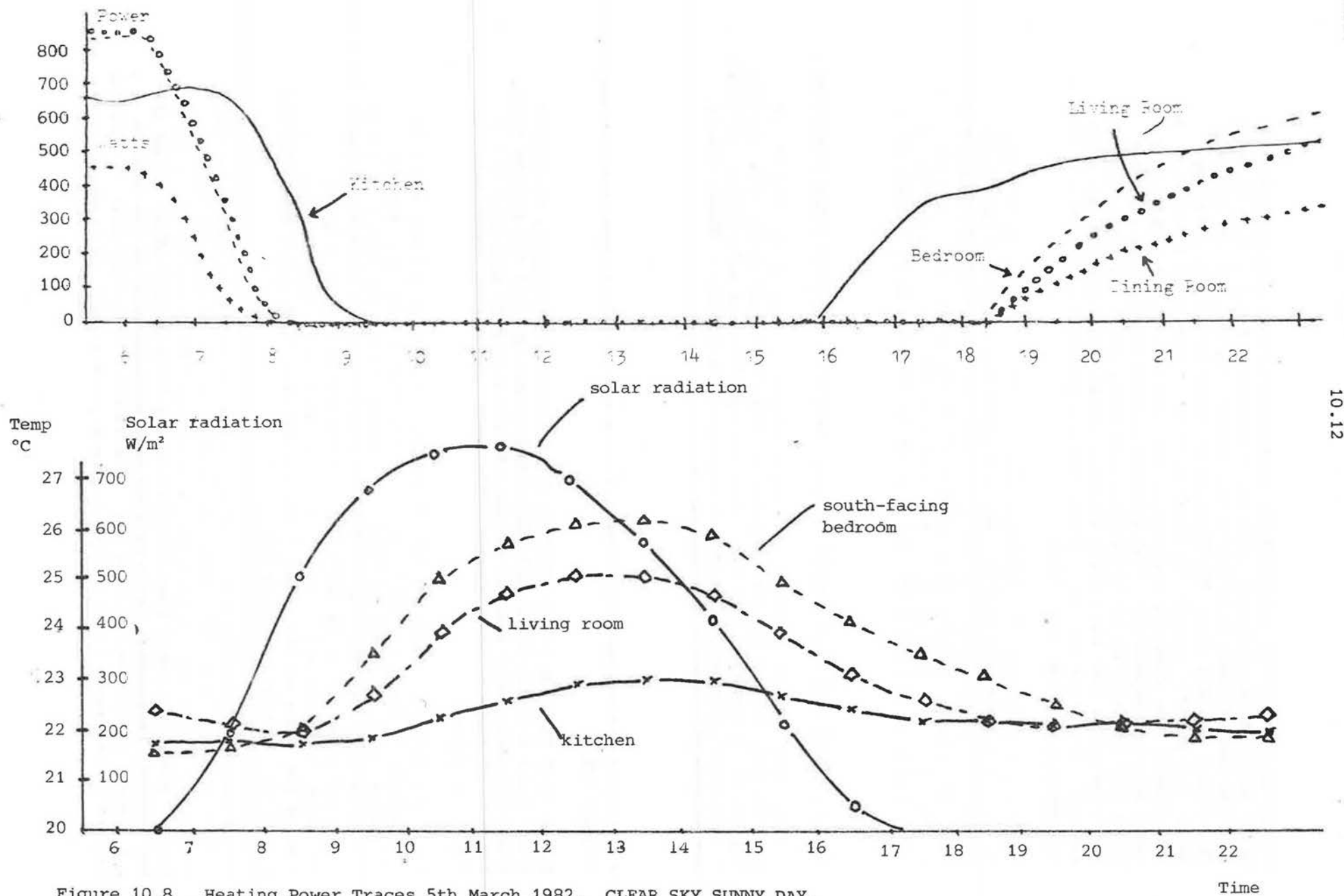
Figure 10.8 Heating Power Traces 5th March 1982. CLEAR SKY SUNNY DAY.
