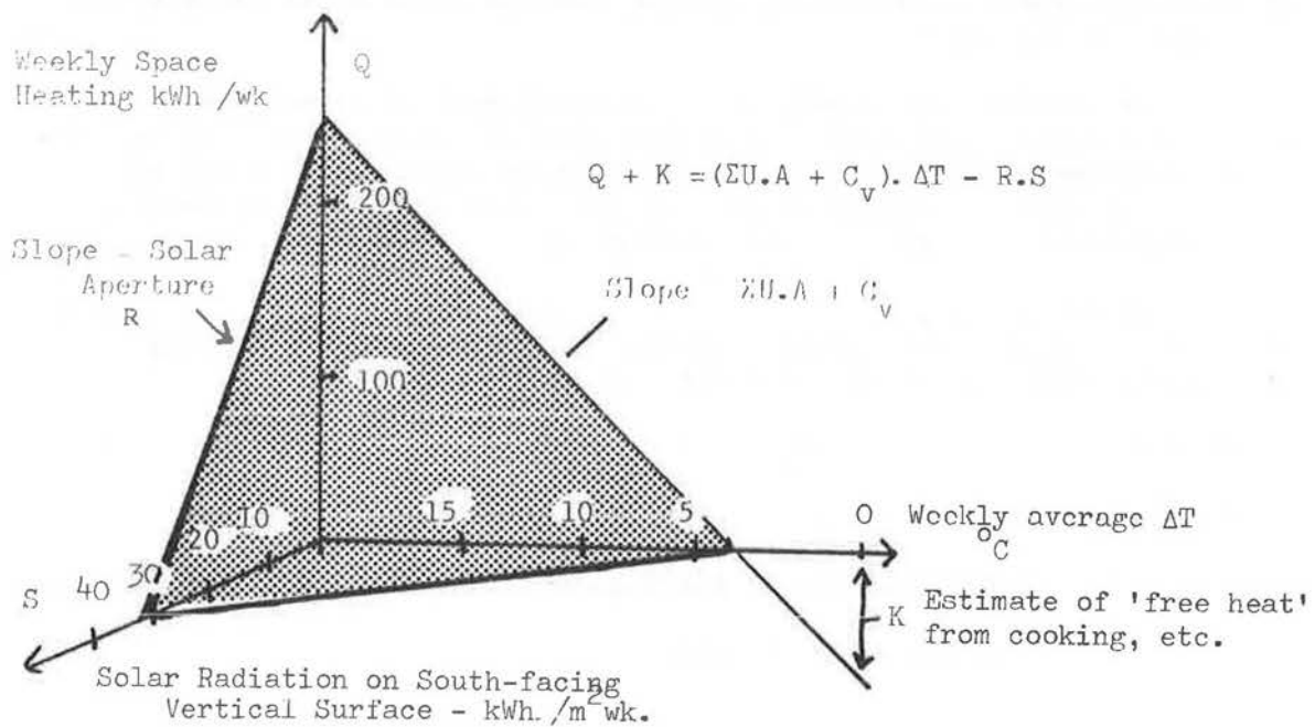
Figure 10.17 Triaxial Regression
