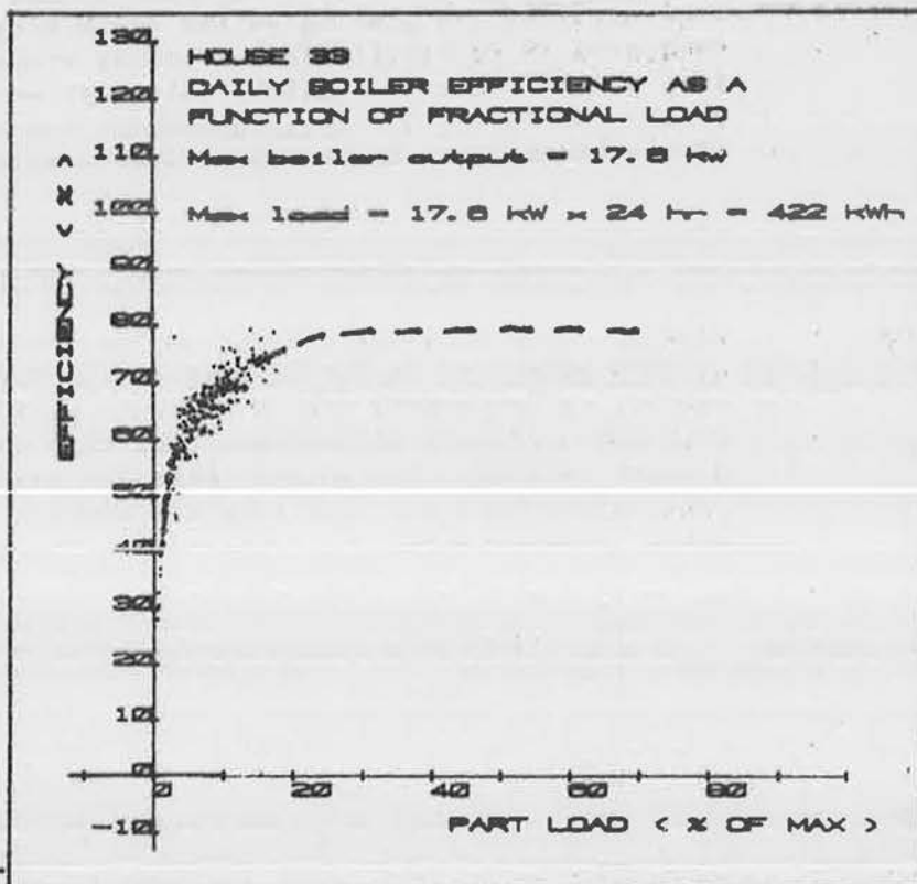
Figure S30. The boiler is always operating below 22% of absolute maximum load on a daily basis
