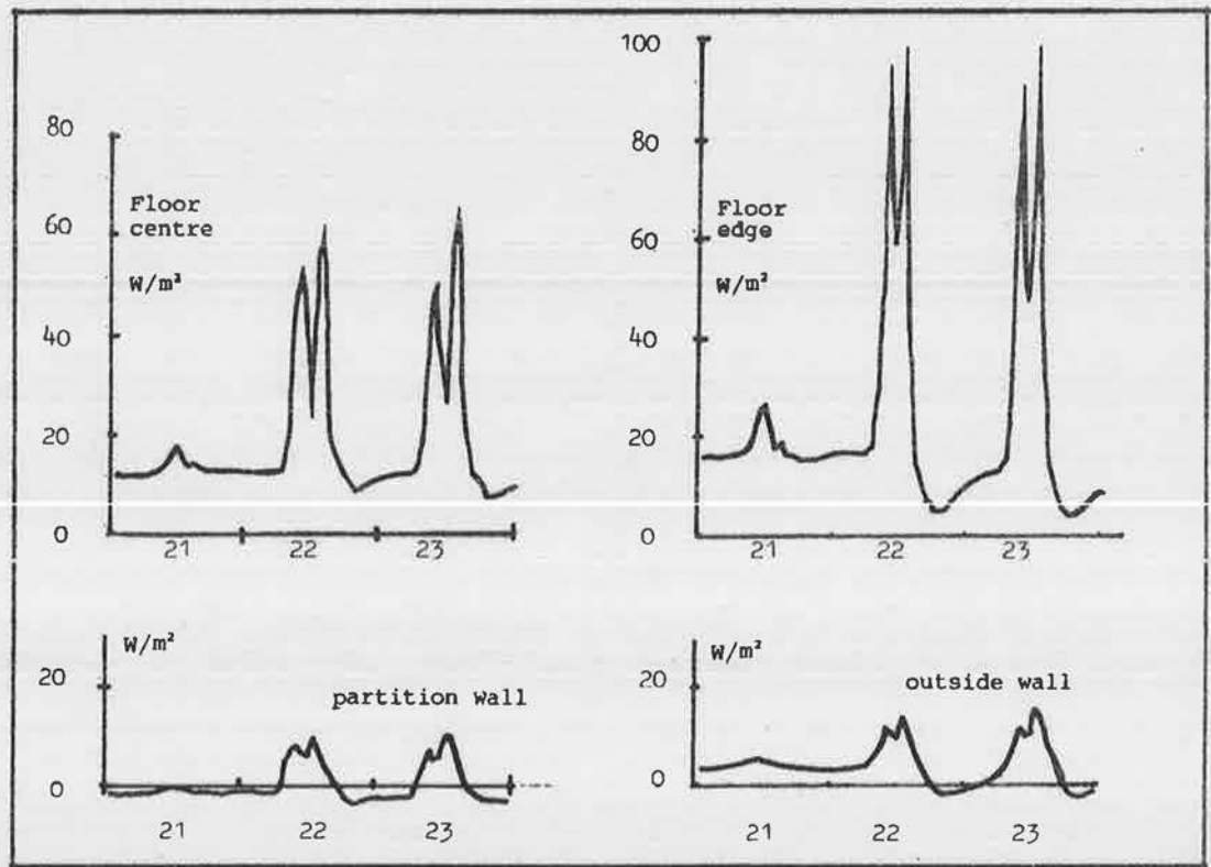
Figure S23. The effect of solar radiation on space heating and surface heat flux in the test house
