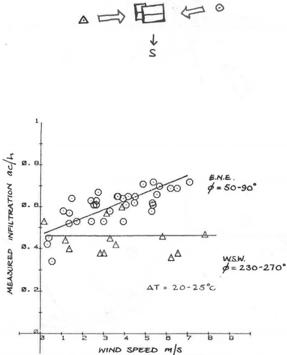
Figure A9.1.5 Measured infiltration rates at different wind speeds, for direction parallel to street. The house is sheltered to the west, but not to the east.
