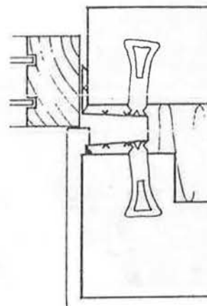
Figure 4.4 Dacatie cavity closure detail
