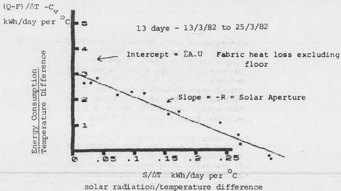
Figure S12. A typical example of the regression analysis used to estimate solar aperture and fabric heat losses
