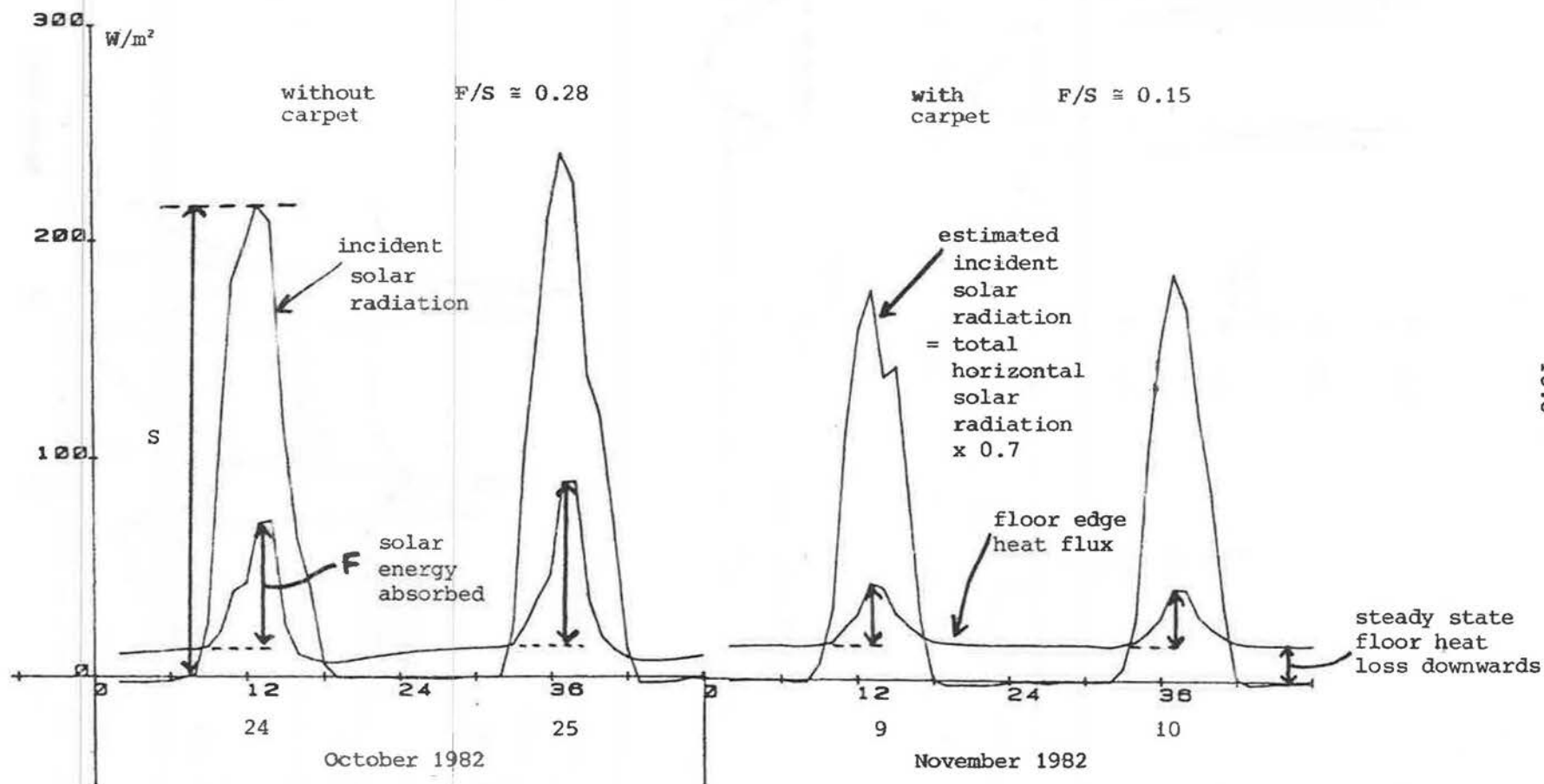
Figure 10.4 Effects of Carpet on Floor Heat Flux
