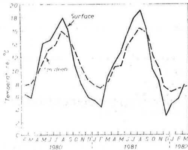
Figure 8.28 Relationship of average ground surface temperature and temperature at depth 1 metre.
