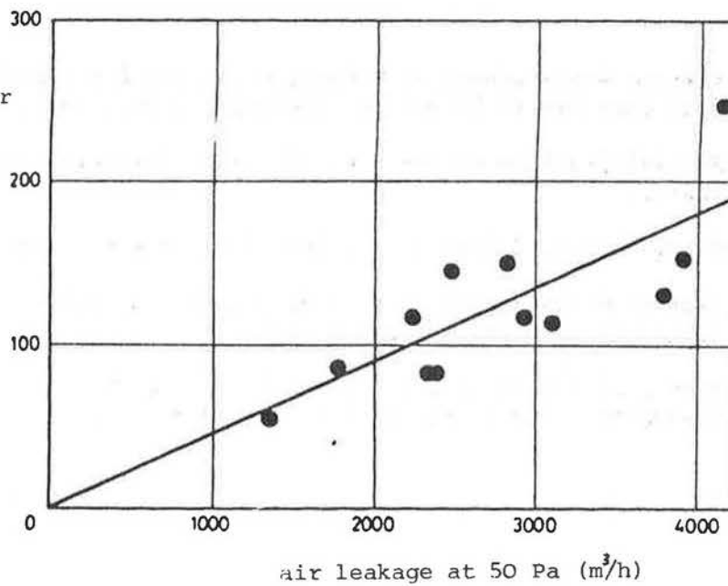
Figure A9.2.1 Variation of whole house infiltration rates with air leakage from BRE sample (reference 9.1)
