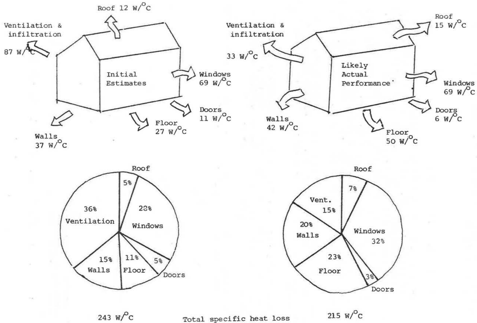
Figure 8.19 HOUSE HEAT LOSSES
