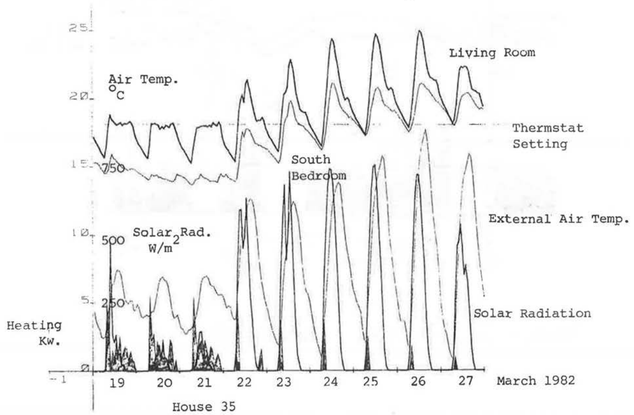
Figure 10.12 Solar Radiation and Space Heating
