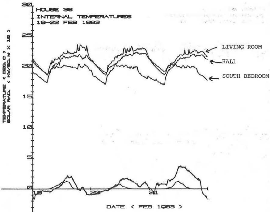
Figure 13.5 Temperature profiles during cold weather
