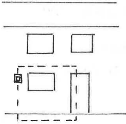
Figure 8.15 Pennyland Floor Edge Heat Losses
