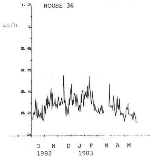
Figure 9.12 Estimated daily average air infiltration rates
