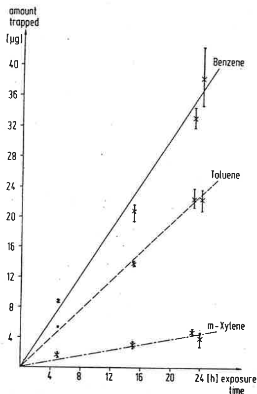
FIGURE 2 Relationship between exposure time and amounts of aromatic hydrocarbons trapped by the Gasbadge™ sampler.
