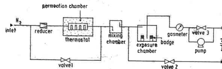
FIGURE 1 Device for generation of test gas atmospheres and exposure experiments.
