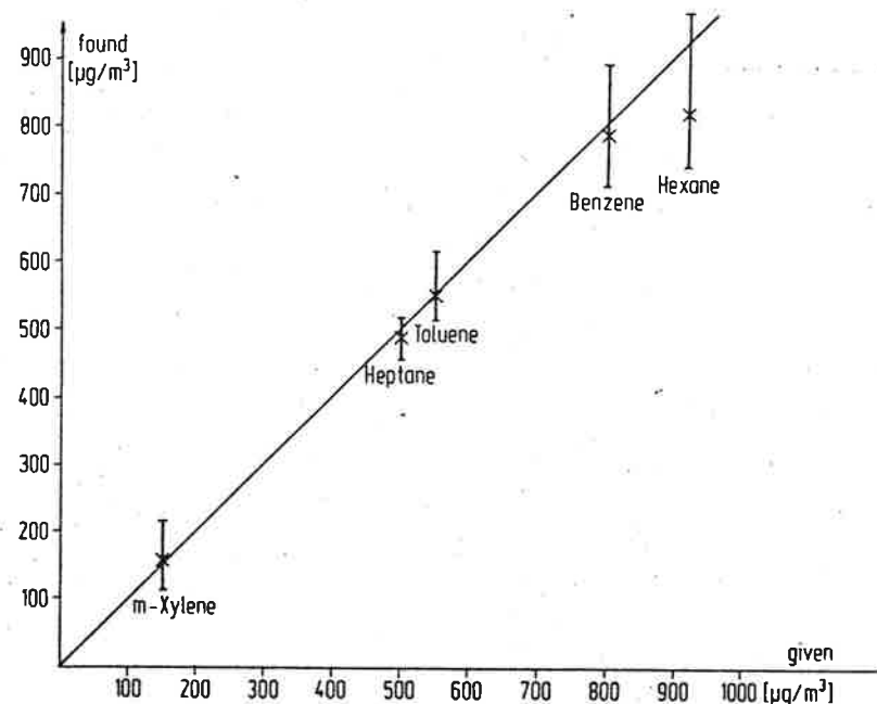
FIGURE 4 Determination of the hydrocarbon content of test gas atmosphere with Gasbadge™ samplers.
