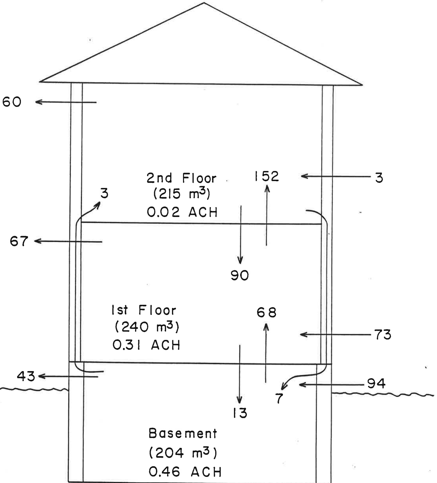
BROOKHAVEN HOUSE (All Flow Rates in m 3 /h)
