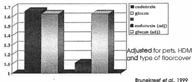
Fig. 3 \beta(1,3) -glucan and endotoxin in relation to PEF variability in children with respiratory symptoms (Brunekreef et al., 1999) PEF: Peak Expiratory Flow
