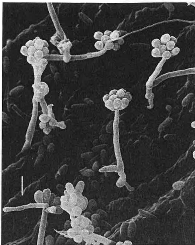
Fig. 4 SEM picture of Stachobotrys chartarum an important member of "the damp building associated fu ga". Magnification 2000 \times . Photo: Robert A. Samson (Gravesen et al., 1994)
