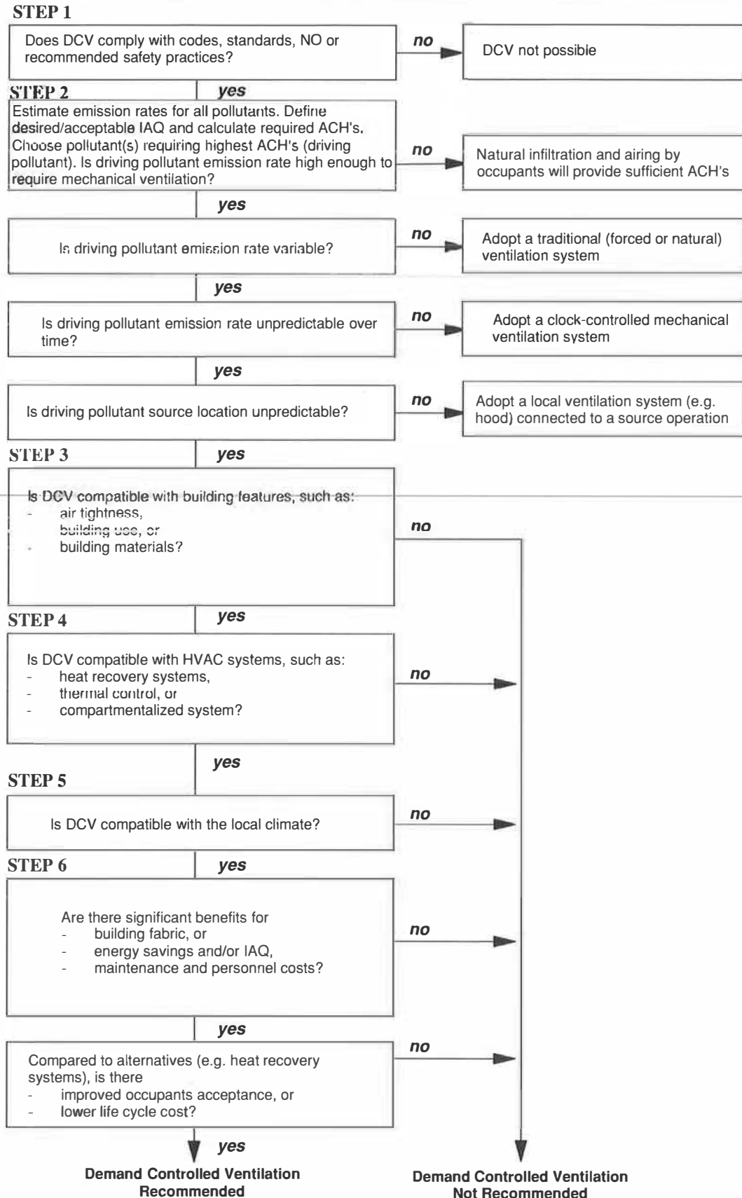
Figure 2.1 The most appropriate conditions for demand controlled ventilation
