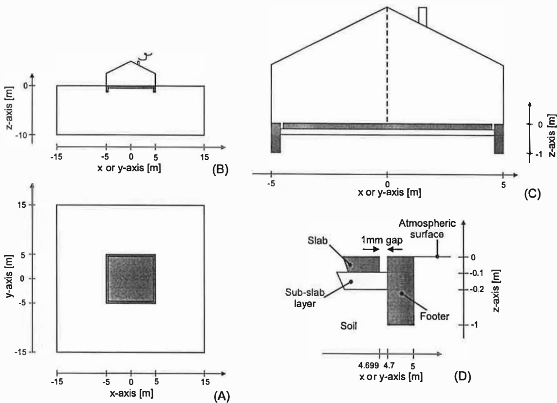
Figure 2. Case 2 geometry (not drawn to scale). (A) is the house viewed from the top, and (B) to (D) are different side views of the house.
