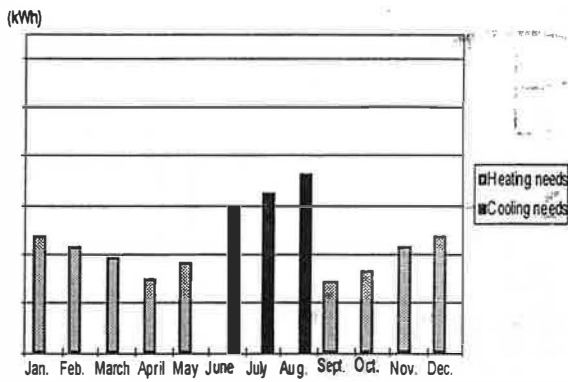
figure 3 : Lille, heating and cooling needs ; figure 4 : Madrid, heating and cooling needs Collected solar energy
