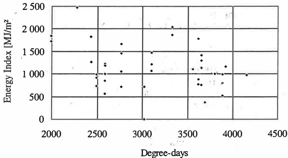
Figure 2: Total energy index 1 and degree-days in 56 European office buildings. The largest energy consumption is more than six times the smallest! [Roulet et al, 1995]
