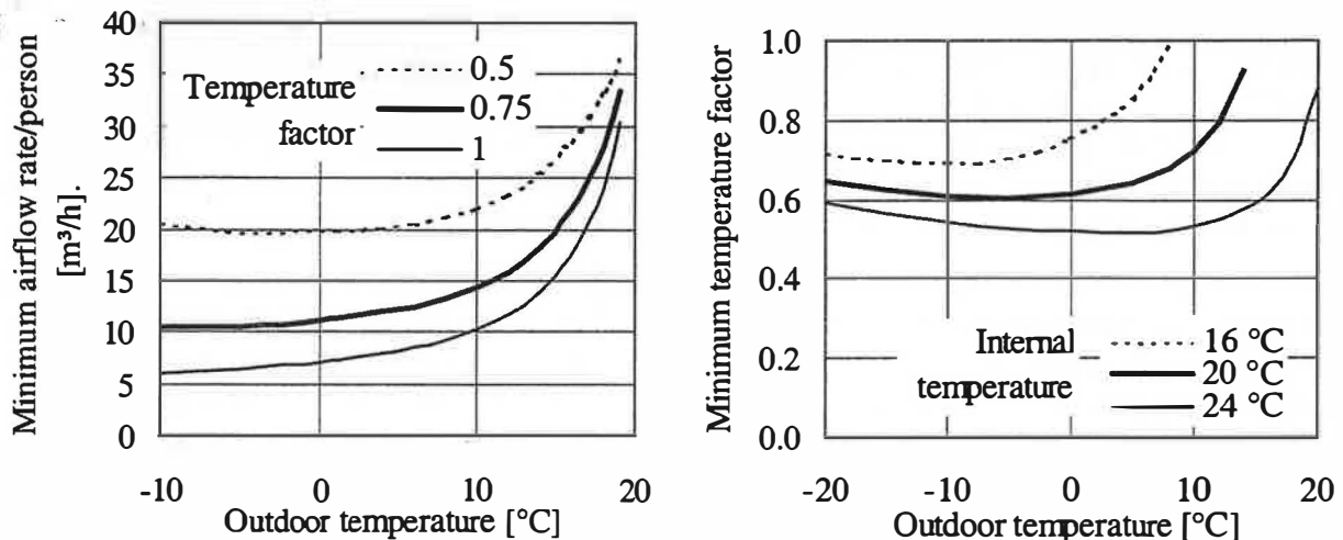
Figure 4: Conditions to avoid moisture growth on external walls 4 .
