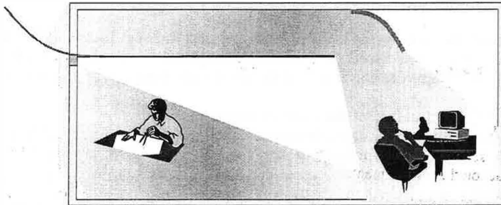
Figure 7: Principle of the anidolic ceiling. A part of the light is reflected by carefully shaped mirrors to the back of the room .
