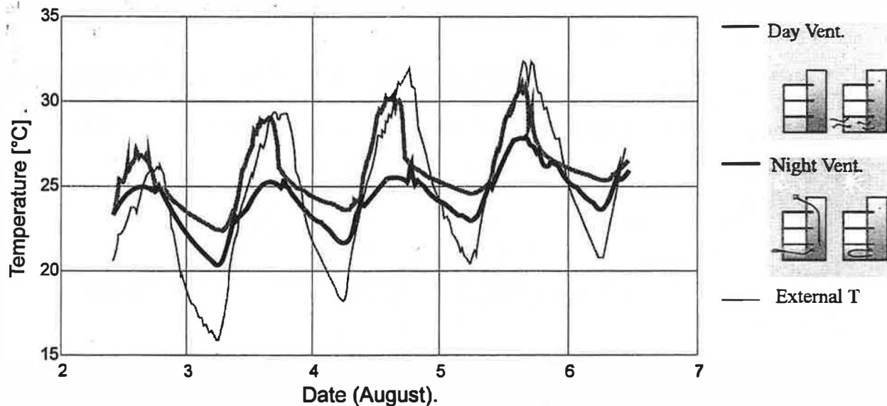
Figure 6: Effect of passive cooling through night ventilation on the LESO building.
