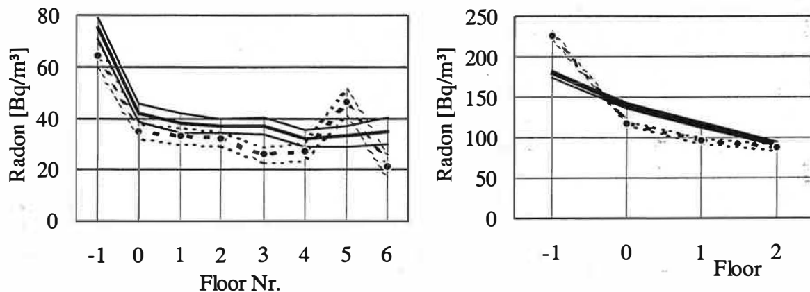
Figure 5: Geometric average \pm 95% confidence interval of radon concentration in 25 multifamily dwellings (left) and 7 single family homes in Switzerland; before (full line) and after (dotted line) energy retrofit [Cramer et al. 1992].
