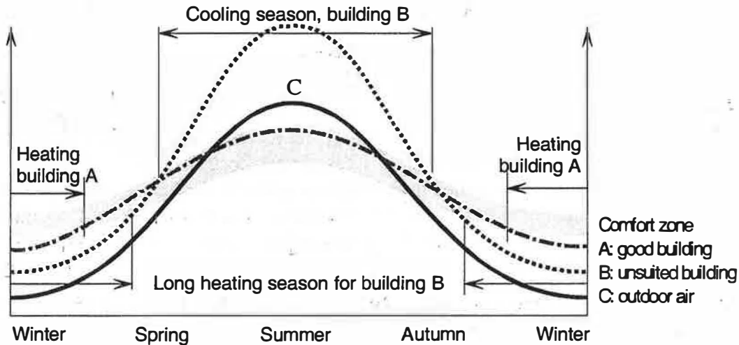
Figure 1: Evolution of temperatures in a free floating building and its environment throughout the year (Northern hemisphere).
