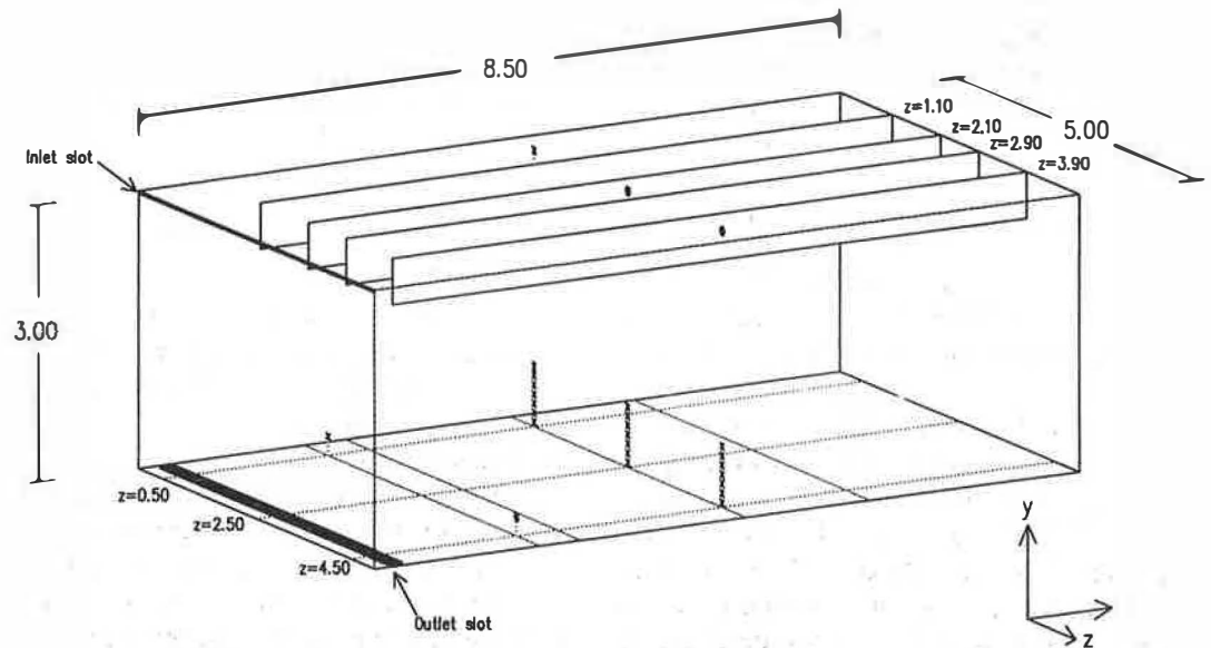
Figure 2 The Full scale test room with inlet slot, outlet slot and guiding plates.
