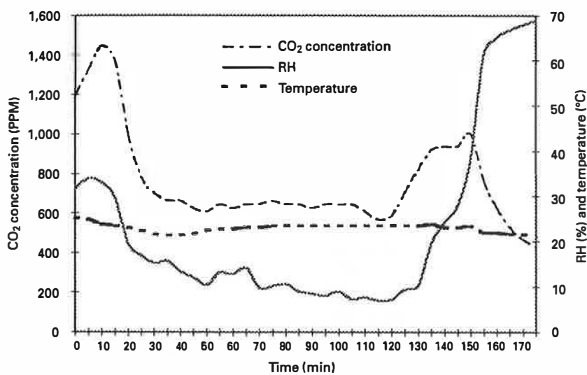
Fig. 3. CO 2 concentration, RH and temperature for the DC 9 (Flight 6/30B).
