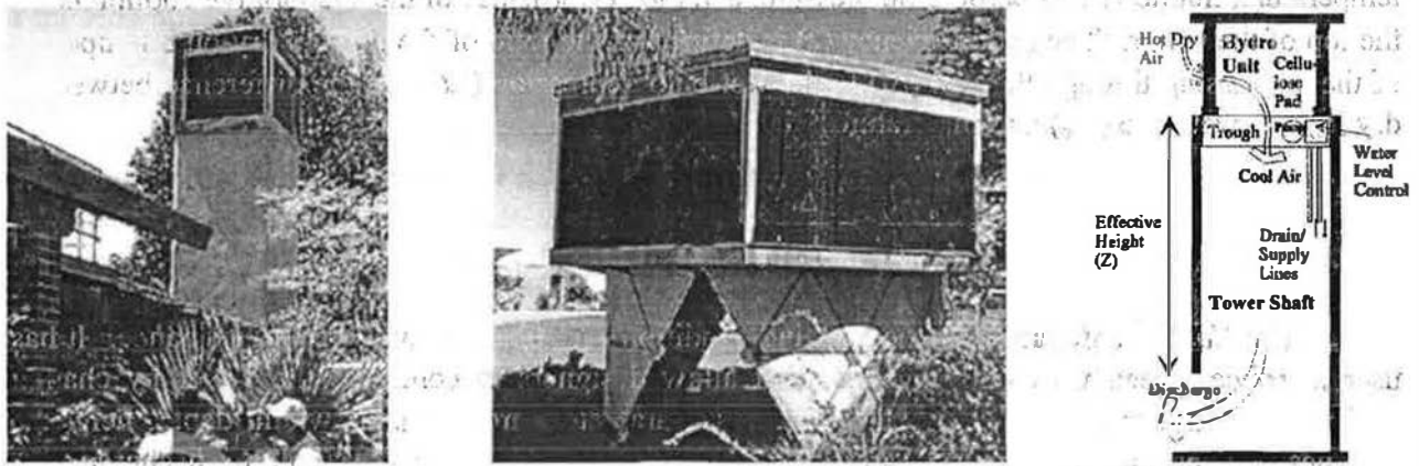
Figure 1. The Hodges Residential Cool Tower in Tucson(left), Hydro Unit Prototype at ERL (middle), and Cool Tower Schematic(right)
