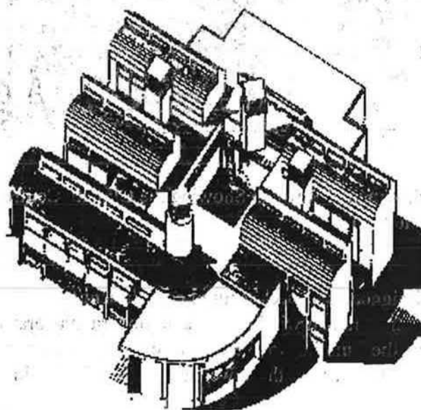
Figure 4. The BTC Building with Four Cool Towers
