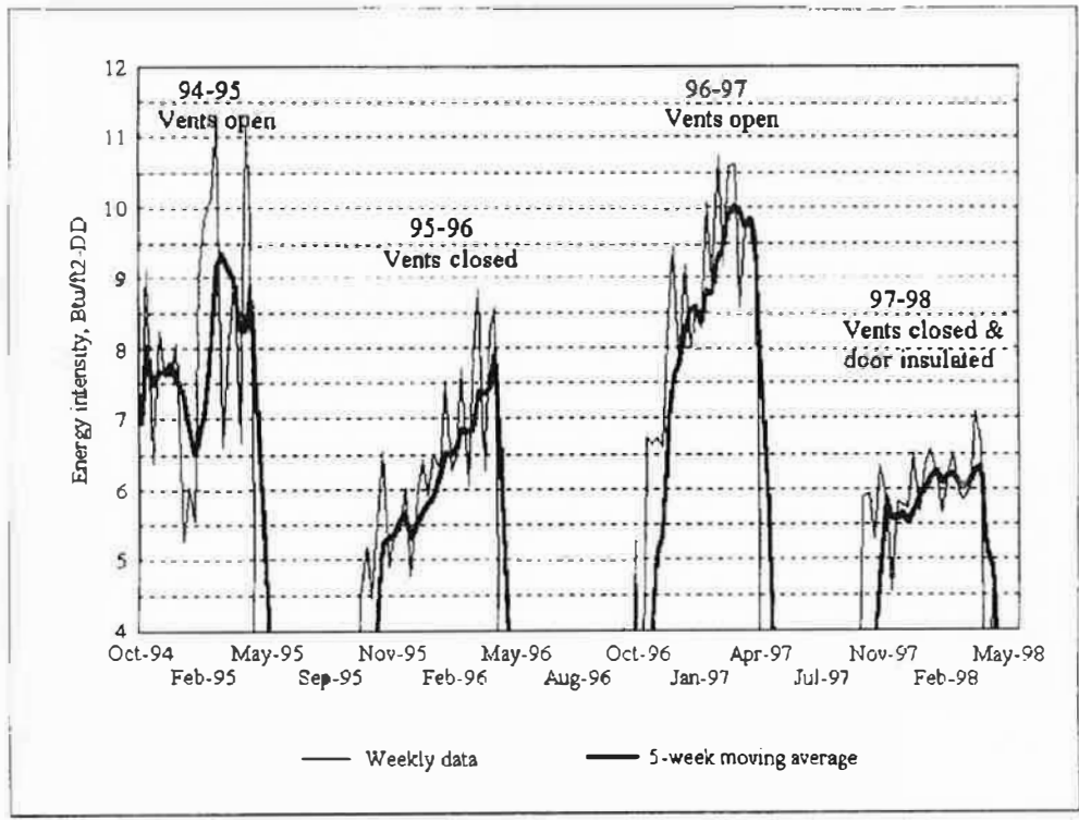
Figure 4. Weekly energy intensities of case study house over four heating seasons, showing the effect of open crawl space vents on energy consumption. Vents were open in the winters of 94-95 and 96-97, closed in 95-96. In 97-98 the crawl space access door was also insulated and air-sealed.
