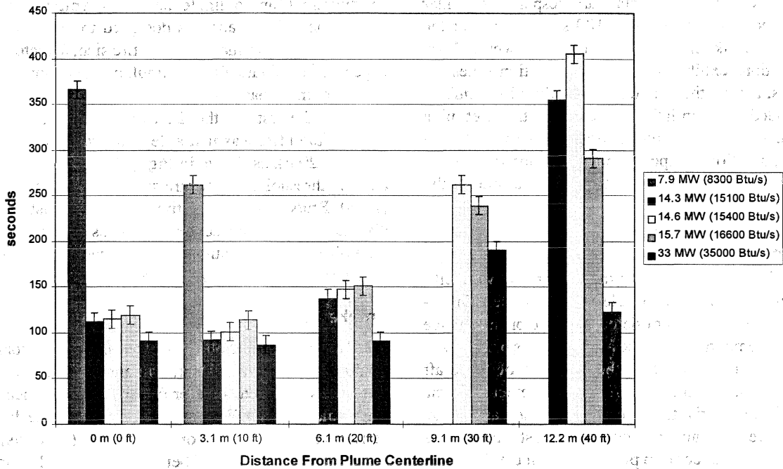
Figure 5 Earliest activation time of 79°C (175°F) sprinkler bulbs in the 22 m (73 ft) hangar as a function of distance and fire size. The fires are identified by total heat release rate. Uncertainties in these heat release rates are given in Table 4.
