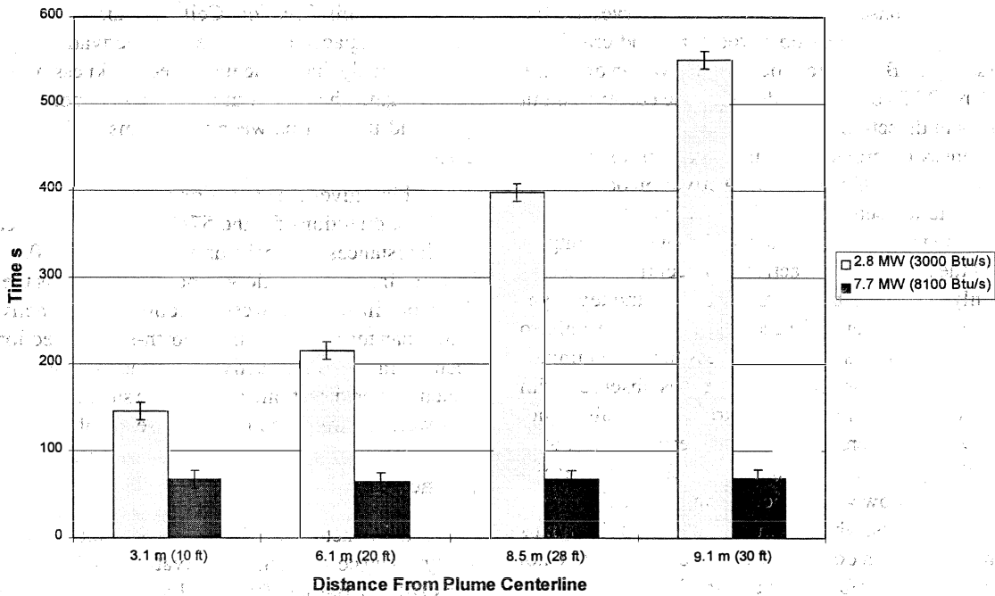
Figure 8 Earliest activation times as a function of distance for 57°C (135°F) heat detectors in the 15 m (50 ft) hangar for two tests that have draft curtains.
