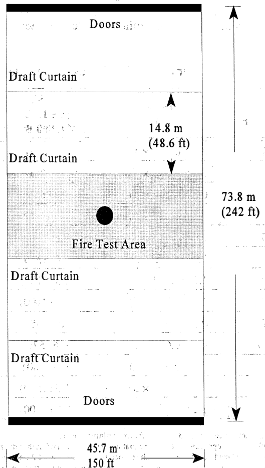
Figure 2 Plan view of 22 m (73 ft) hangar.
