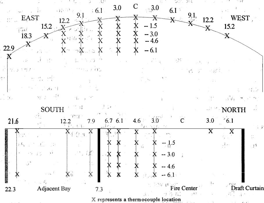
Figure 3 Thermocouple locations (m) for the 22 m (73 ft) hangar.
