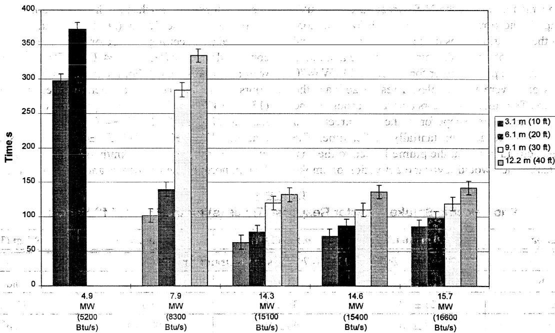
Figure 9 Earliest activation times as a function of distance for 57°C (135°F) heat detectors in the 22 m (73 ft) hangar. Distances from fire center are given in the side box in meters (feet).
