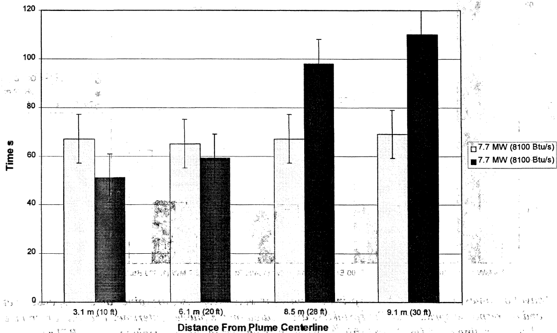
Figure 7 Earliest activation time for 57°C (135°F) heat detectors as a function of distance for the 2.5 m diameter JP-5 pan fires with and without a draft curtain in the 15 m hangar. The draft curtain tests are represented by the first bar at each position.
