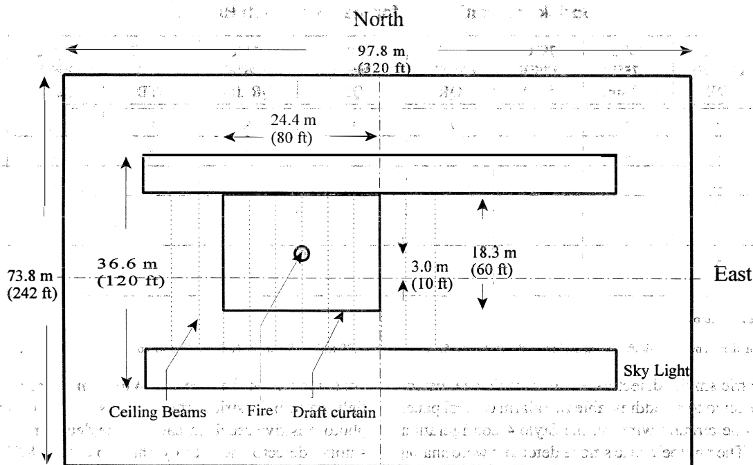
Figure 1 Plan view of 15 m (50 ft) hangar bay.
