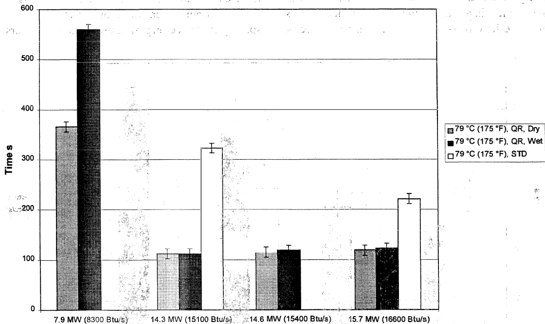
Figure 6 Activation times of 79°C (175°F) sprinkler bulbs for quick response, dry pipe, quick response, wet pipe, and standard response sprinklers. The sprinklers are located on the plume centerline. The quick response sprinklers had an RTI rating of 35 (m/s) 1/2 (63 [ft/s] 1/2 ), while the standard response sprinkler had an RTI rating of 188 (m/s) 1/2 (340 [ft/s] 1/2 ).
