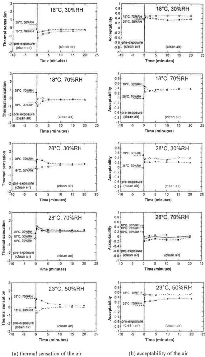
(a) thermal sensation of the air (b) acceptability of the air Fig. 4 Thermal sensation and acceptability of clean air at five different levels of temperature and humidity for 20-min exposures after step-changes from different temperatures and humidities of prior exposure clean air
