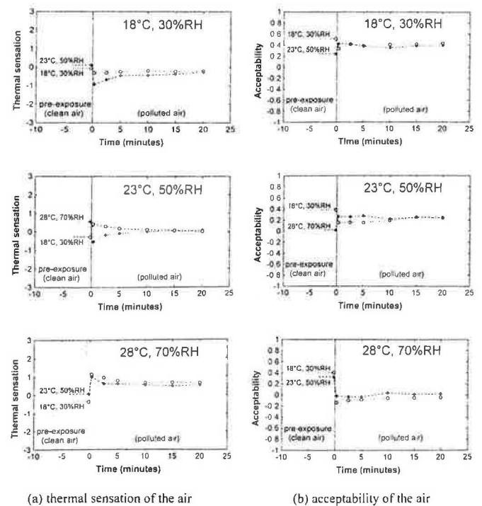
(a) thermal sensation of the air (b) acceptability of the air Fig. 5 Thermal sensation and acceptability of polluted air at three different levels of temperature and humidity during a 20-min exposure after step-change from different temperatures and humidities of prior exposure clean air
