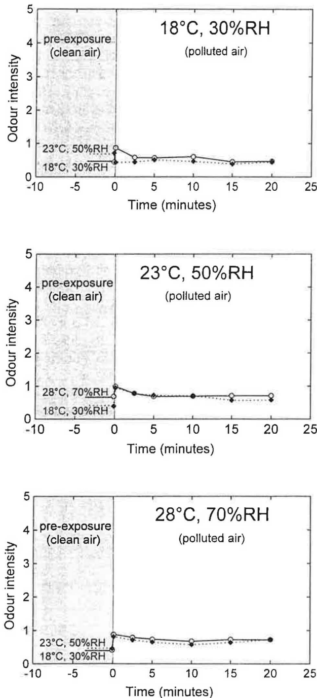
Fig. 10 Odour intensity of the polluted air at three different levels of temperature and humidity during a 20-min exposure after step-change from different temperatures and humidities of prior exposure clean air
