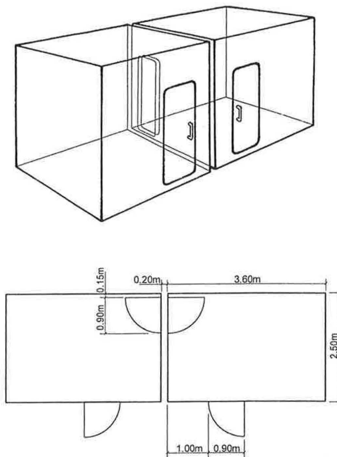
Fig. 2 Perspective view and plan of the two adjacent climate chambers
