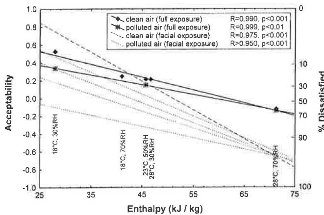
Fig. 8 The acceptability-enthalpy relations obtained from the experiment with whole-body exposure compared with the results from the experiment with facial exposure
