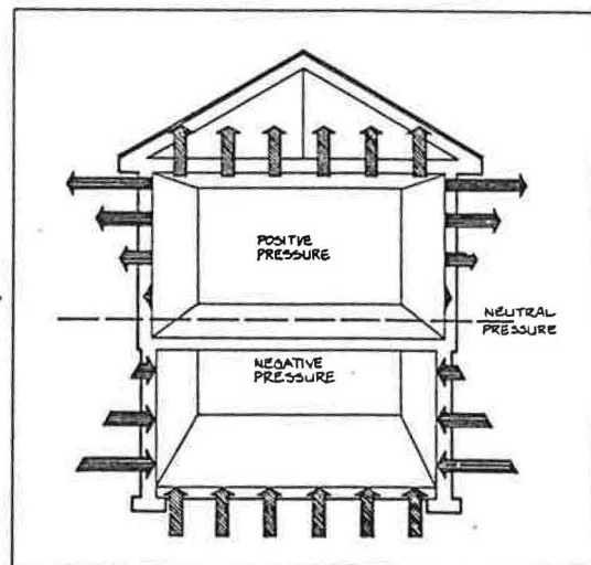
Figure 3: Pressure Distribution in a Typical House
