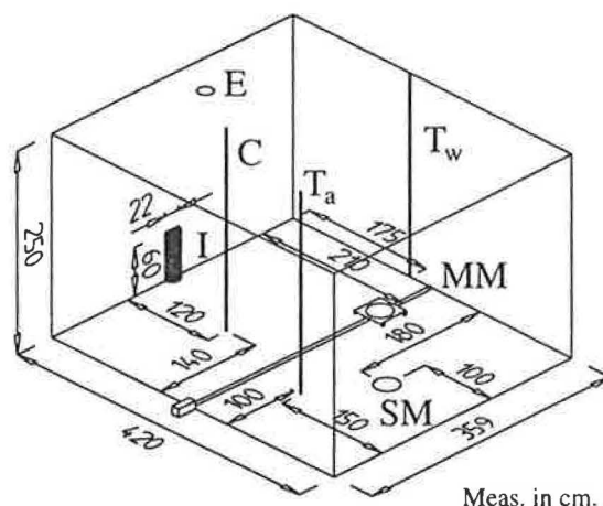
Figure 1: Test room with experimental setup. Location of inlet (I), exhaust (E), sitting manikin (SM), moving manikin (MM), measurement of concentrations (C), air temperatures ( T_a ), wall temperatures ( T_w ).
