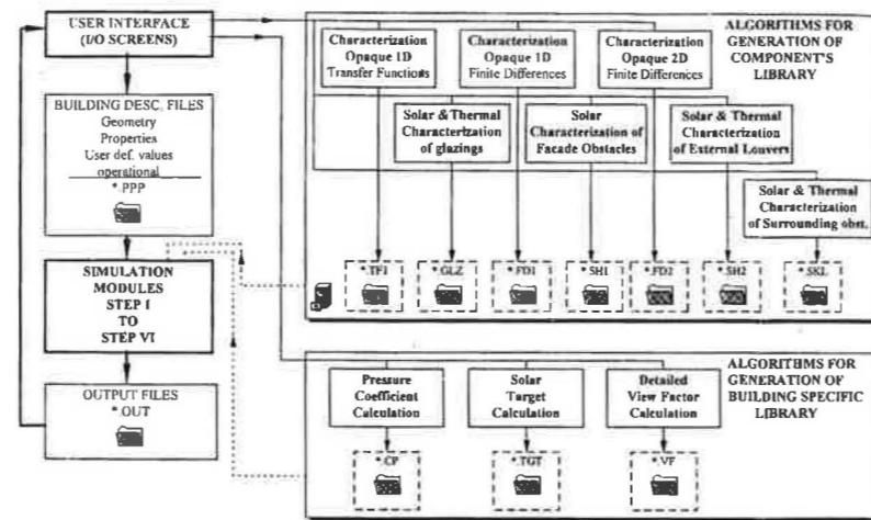
FIGURE 8 Information flow.
