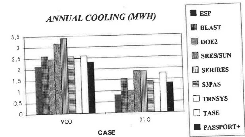
FIGURE 9 Annual cooling (cases 900 and 910).
