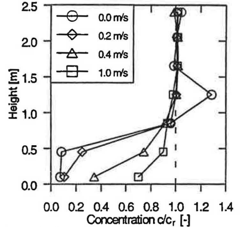
Figure 6: Contaminant added to exhalation (mouth). Concentration profiles for different speeds of moving manikin. Orientation of sitting manikin is 0°.
