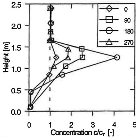
Figure 5: Contaminant added to exhalation (mouth). Concentration profiles for different orientations of sitting manikin. Moving manikin is standing still.
