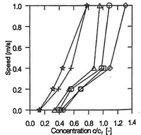
Figure 8: Personal exposure of sitting manikin in all experiments. Regarding nomenclature, see fig. 7.
