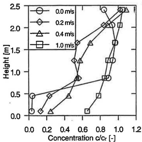
Figure 3: Contaminant added to heat plume above head of sitting manikin. Dimensionless concentration profiles for different speeds of moving manikin.
