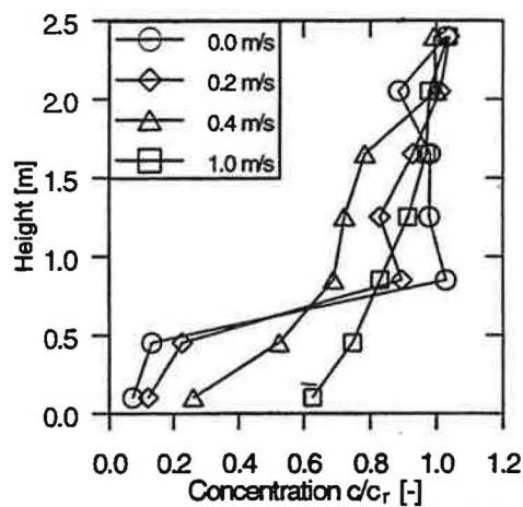
Figure 4: Contaminant added to exhalation (nose) of sitting manikin. Concentration profiles for different speeds of moving manikin.
