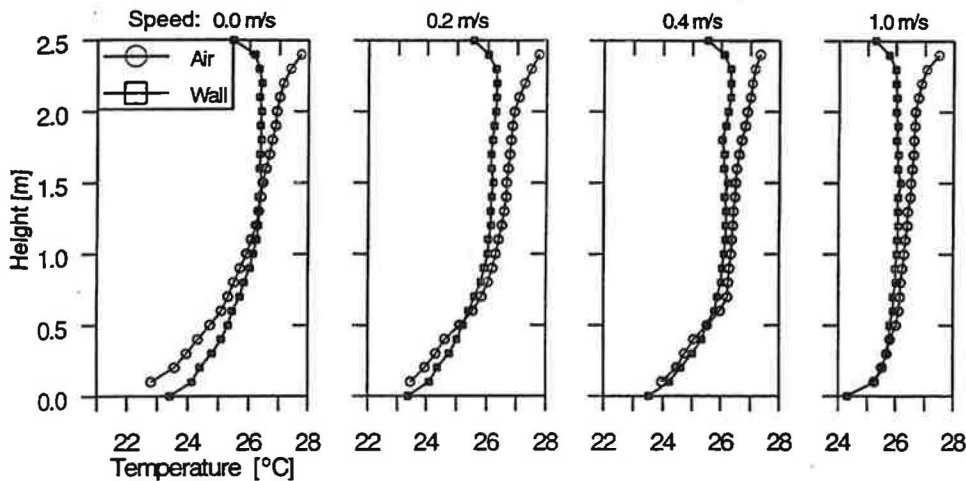
Figure 9: Typical vertical temperature profiles at different speeds of moving manikin, from experiments with exhalation through nose of sitting manikin. Inlet temperature was 16.7°C, exhaust temperature 27.3°C.
