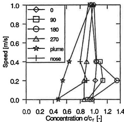
Figure 7: Personal exposure of moving manikin with different ways of adding contaminant: Mouth of sitting manikin at 4 different orientations, plume, and nose.
