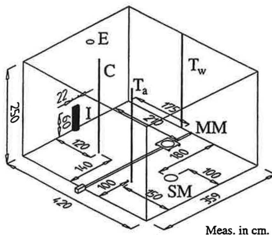
Figure 1: Test room with experimental setup. Location of inlet (I), exhaust (E), sitting manikin (SM), moving manikin (MM), measurement of concentrations (C), air temperatures ( T_a ), wall temperatures ( T_w ).
