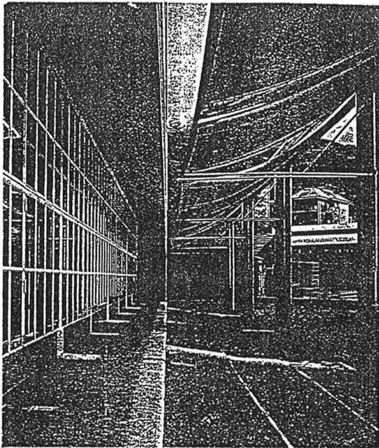
FIG. 15 Combination of fixed and movable shading at Asilo Sant'Elia (G.Terragni).
