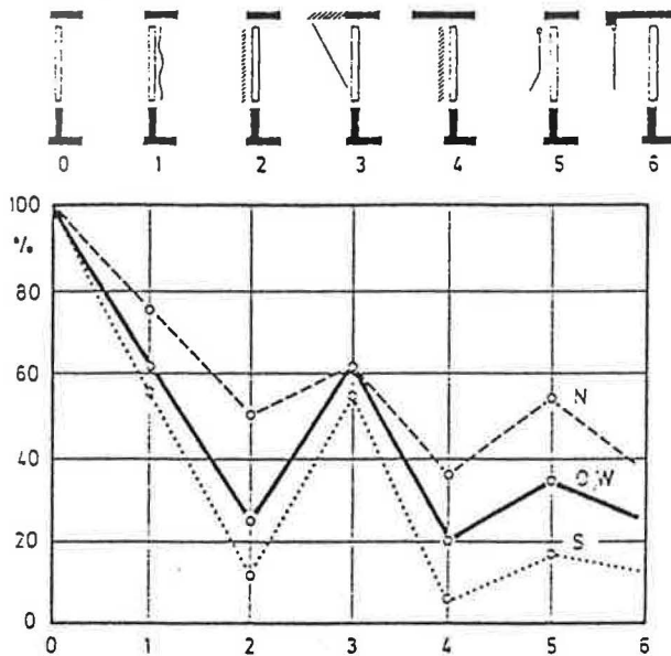
FIG. 23 Percentage reduction in shading coefficient as function of orientation and shade type [6]
