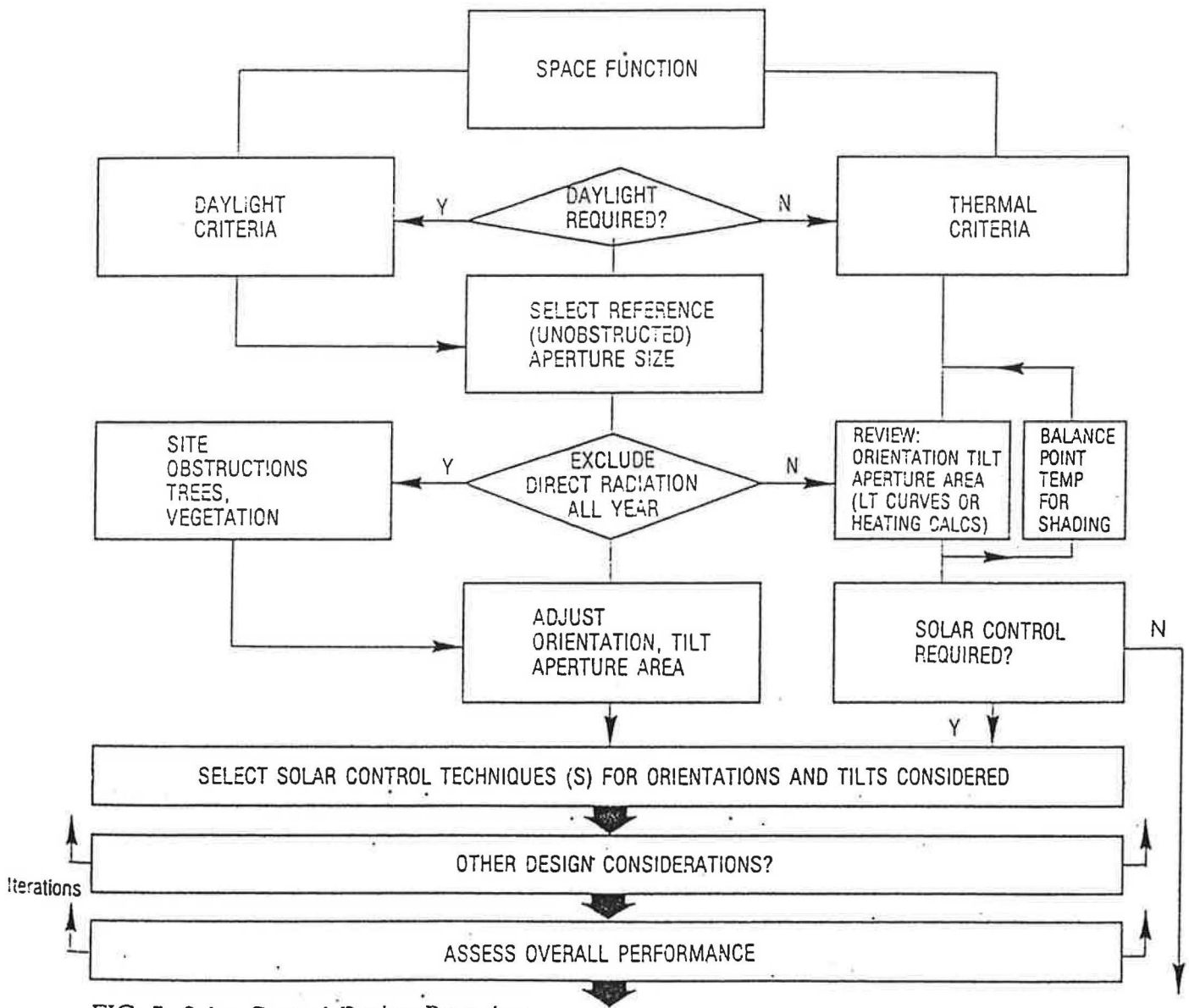
FIG. 7 Solar Control Design Procedure
