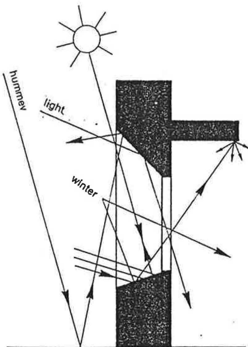
FIG. 18 Slanted openings
