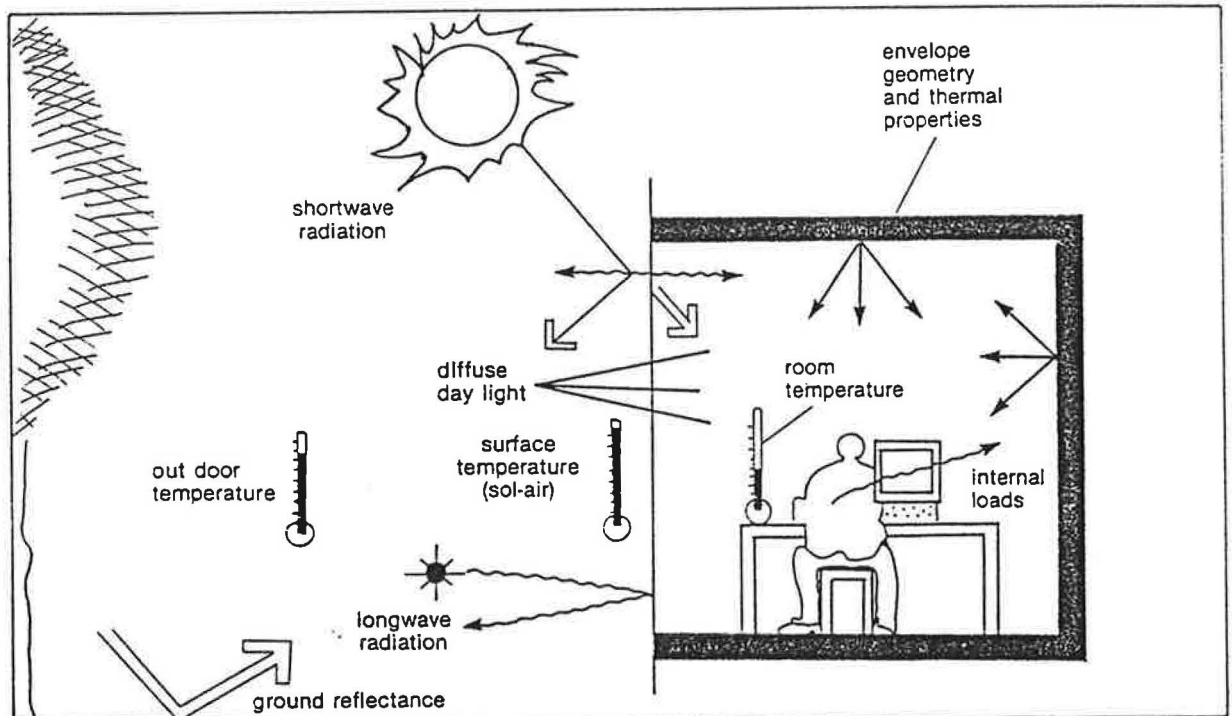
FIG. 2 Design considerations for solar control
