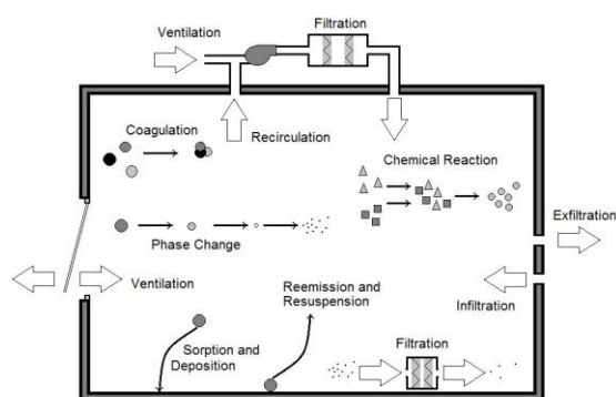
Figure 1: Ventilation Mechanisms and Pollutant Behaviours Indoors
