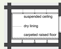
(c) Least effective thermal mass
