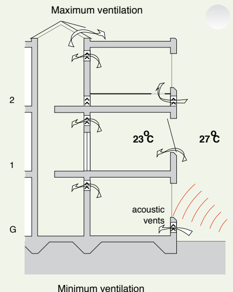
Minimum ventilation
