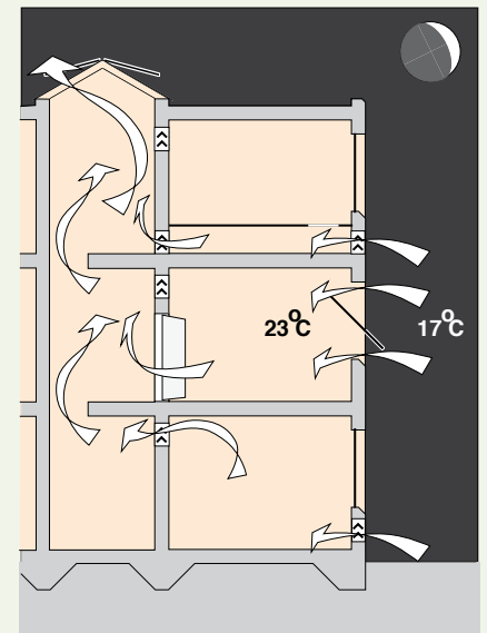
Maximum ventilation
