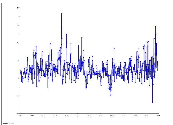
Figure 20: Measuring point 3, Differential pressure Pa, 14.10.2016, 3:00 to 4:00 p.m.
