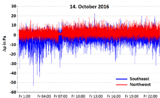
Figure 6: Pressure differences caused by wind 14 th October 2016
