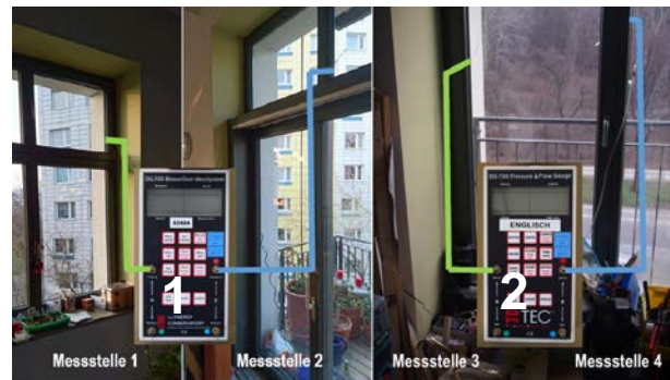
Figure 3: Measurement Configuration 1, pressure recording
