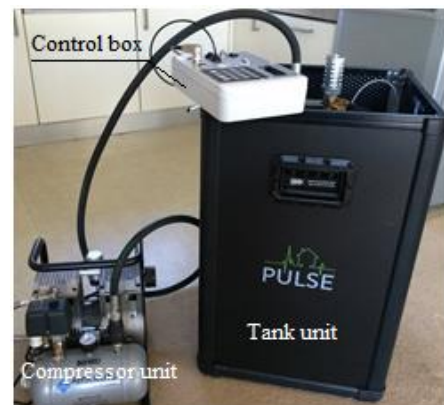
Figure 3 PULSE-60 and associated control box (SW test)
