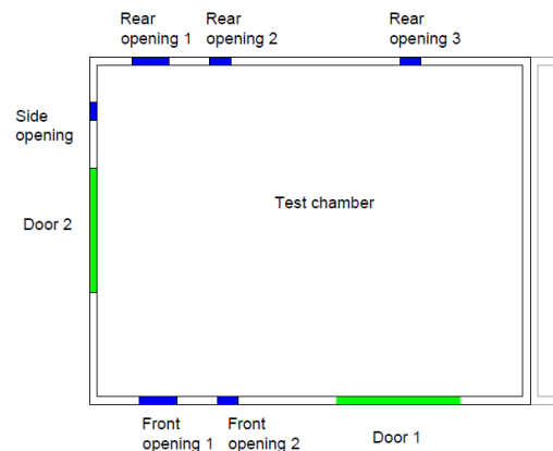
Figure 6 Plan of openings in the test chamber
