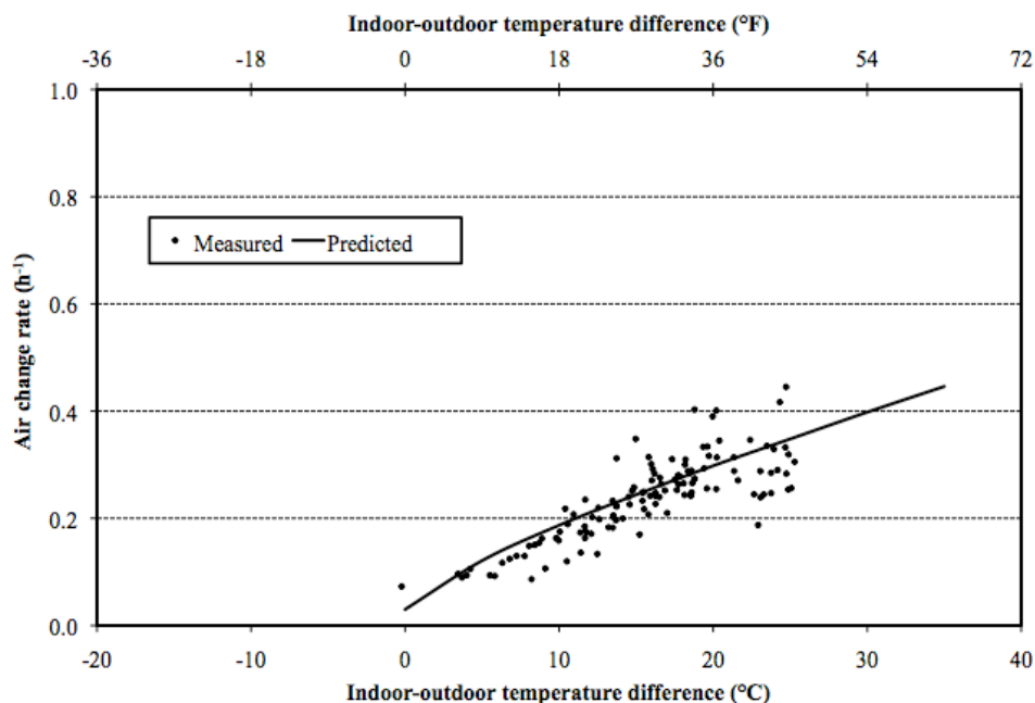
Figure 10. Measured and predicted post-retrofit air change rates as a function of temperature difference (low wind speed): Forced-air fan off (Condition 0).
