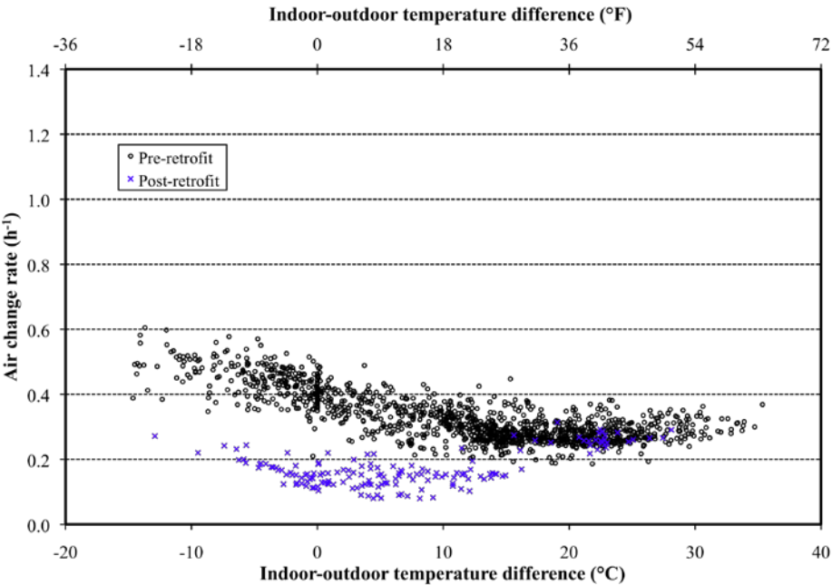
Figure 6. Pre- and Post-Retrofit measured air change rates as a function of temperature difference (low wind speed): forced-air fan on, outdoor air intake sealed (Condition 1a)
