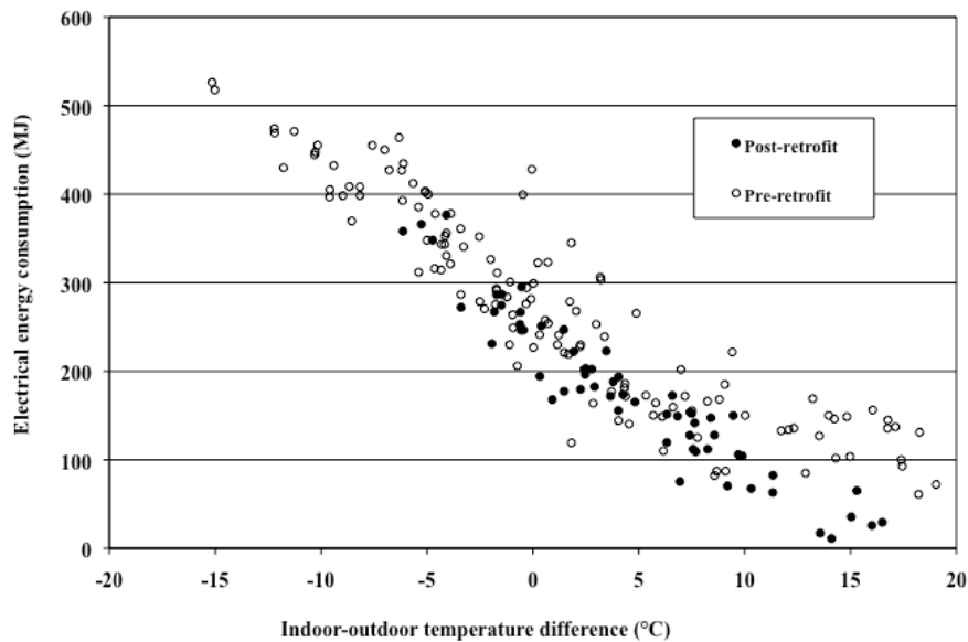
Figure 9. Pre-post electric cooling energy versus indoor-outdoor temperature difference
