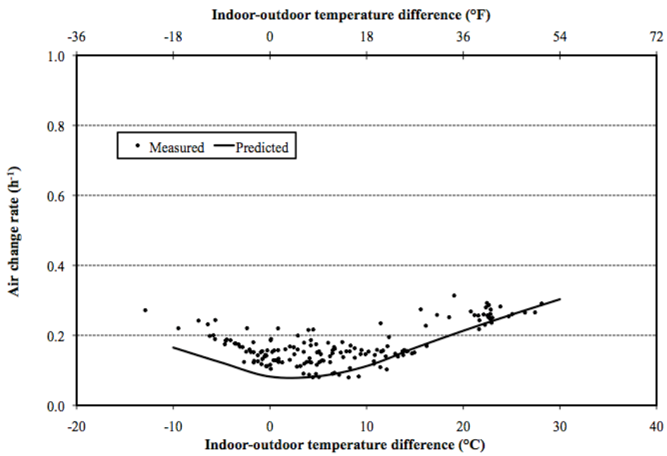
Figure 12. Measured and predicted post-retrofit air change rates as a function of temperature difference (low wind speed): Forced-air fan on, outdoor air intake sealed (Condition 1a).
