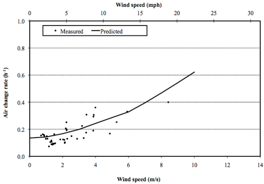
Figure 11. Measured and predicted post-retrofit air change rates as a function of wind speed (low temperature difference): Forced-air fan off (Condition 0).
