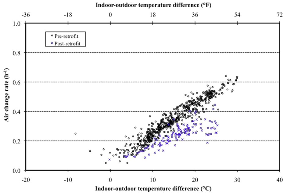
Figure 4. Pre- and Post-Retrofit measured air change rates as a function of temperature difference (low wind speed): forced-air fan off (Condition 0)
