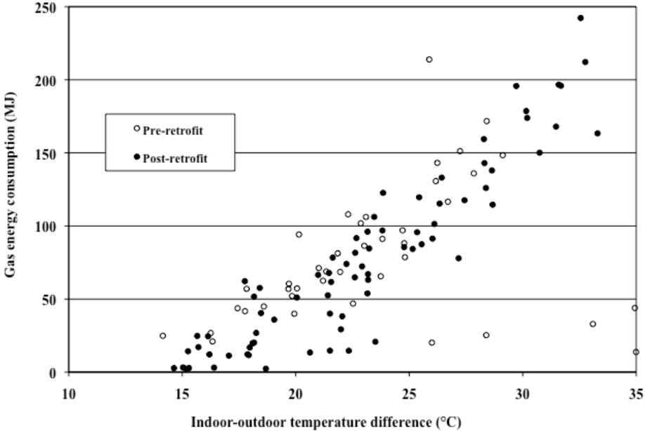
Figure 8. Pre-post gas heating energy versus indoor-outdoor temperature difference
