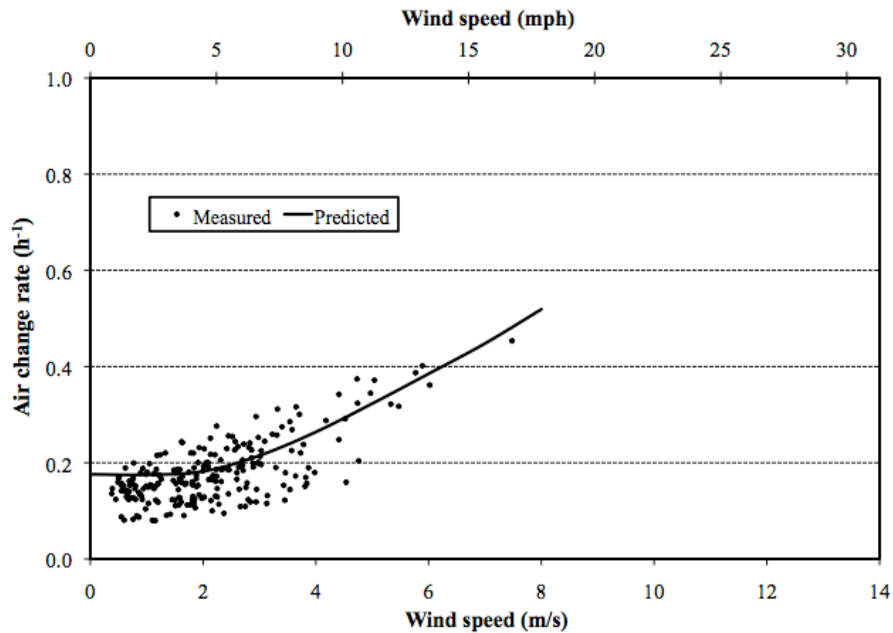
Figure 13. Measured and predicted post-retrofit air change rates as a function of wind speed (low temperature difference): Forced-air fan on, outdoor air intake sealed (Condition 1a).
