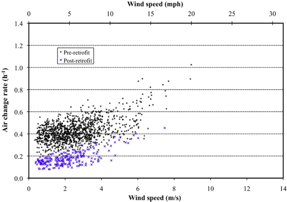
Figure 7. Pre- and Post-Retrofit measured air change rates as a function of wind speed (low \Delta T ): forced-air fan on, outdoor air intake sealed (Condition 1a)
