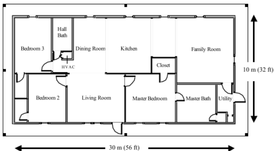
Figure 2. Schematic floor plan of manufactured house.
