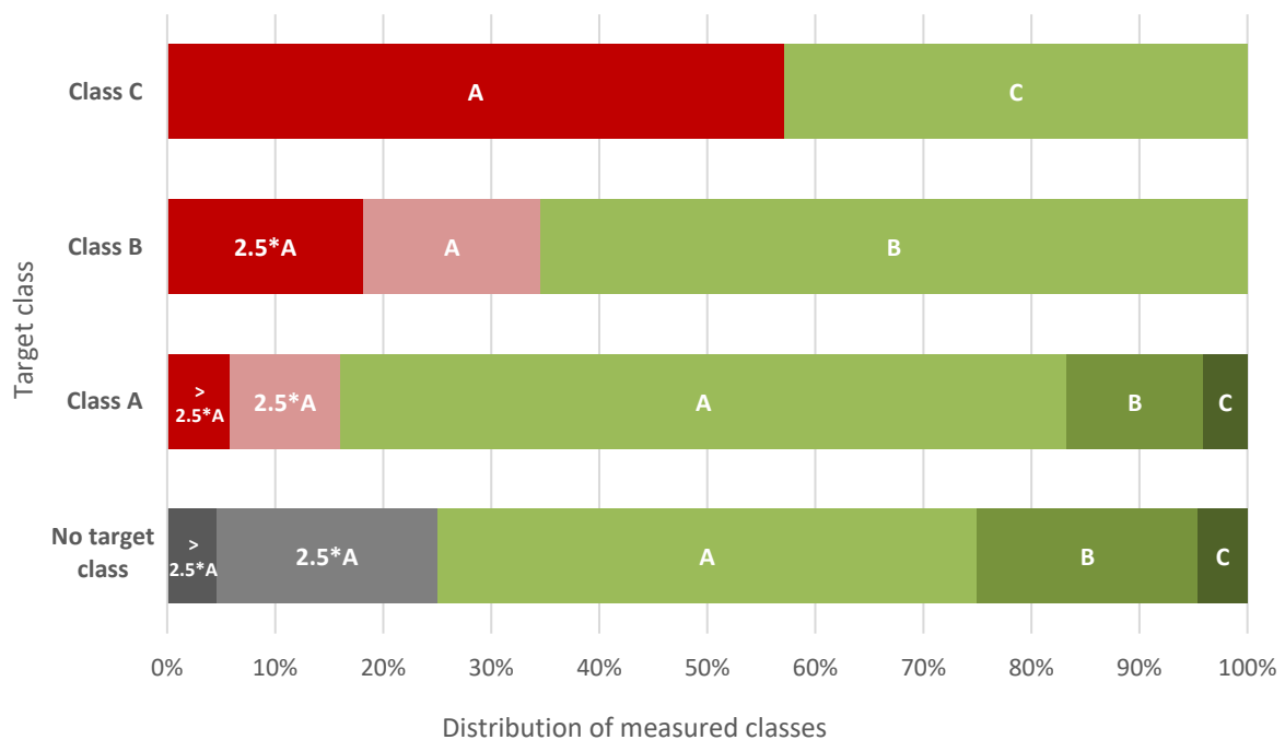
Figure 5: Specific ductwork airtightness measured class depending on target class
