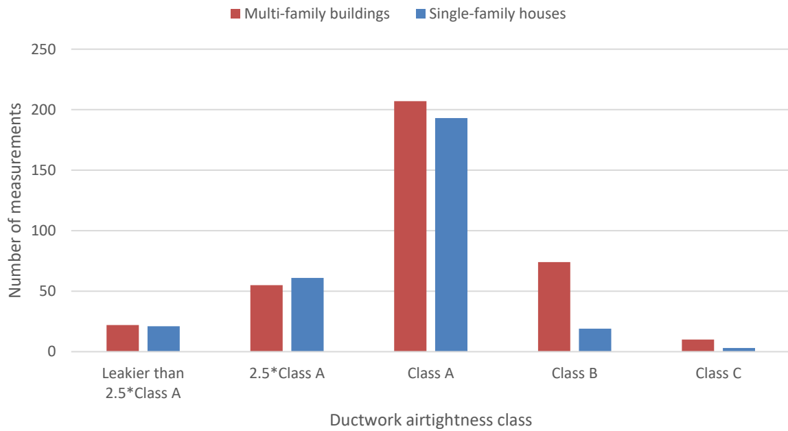
Figure 6: Specific ductwork airtightness measured class in residential buildings
