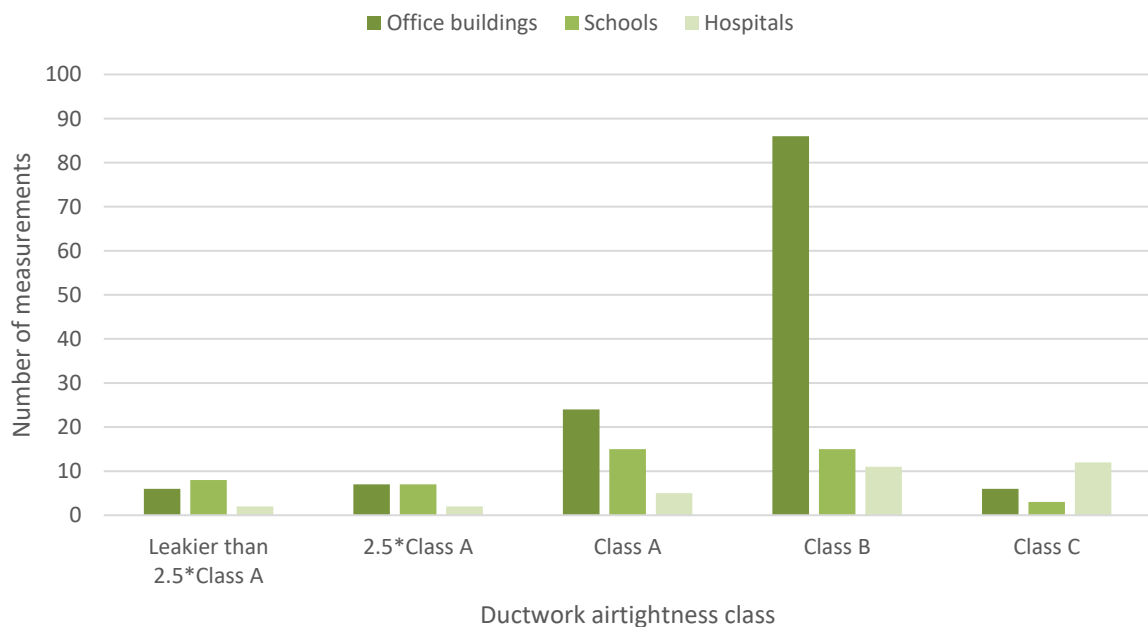
Figure 7: Specific ductwork airtightness measured class in non-residential buildings
