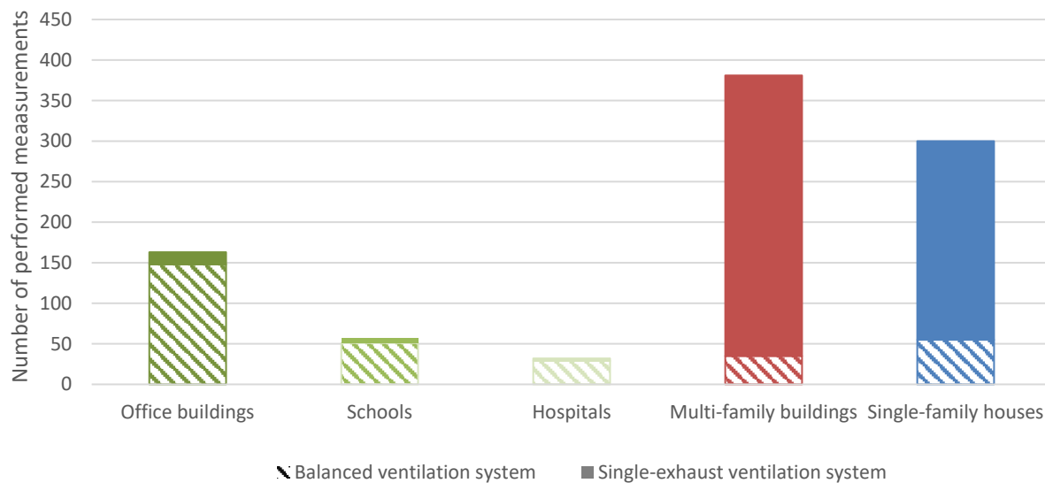
Figure 4: Type of ventilation system depending on buildings' use
