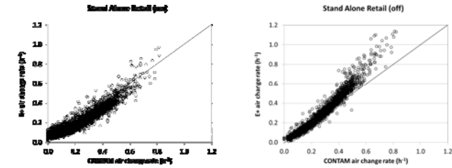
Figure 1: EnergyPlus vs. CONTAM infiltration rates for Stand Alone Retail (a) system-on and (b) system-off
