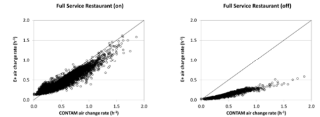
Figure 2: EnergyPlus vs. CONTAM infiltration rates for Full Service Restaurant (a) system-on and (b) system-off
