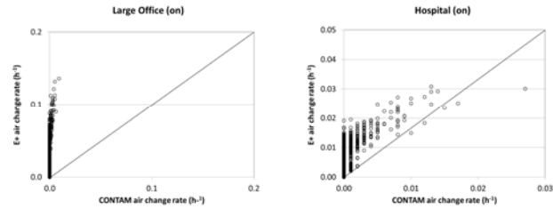
Figure 4: EnergyPlus vs. CONTAM infiltration rates for (a) Large Office system-on and (b) Hospital system-on, low I_{design} value ( 0.000304 \text{ m}^3/\text{s}/\text{m}^2 )
