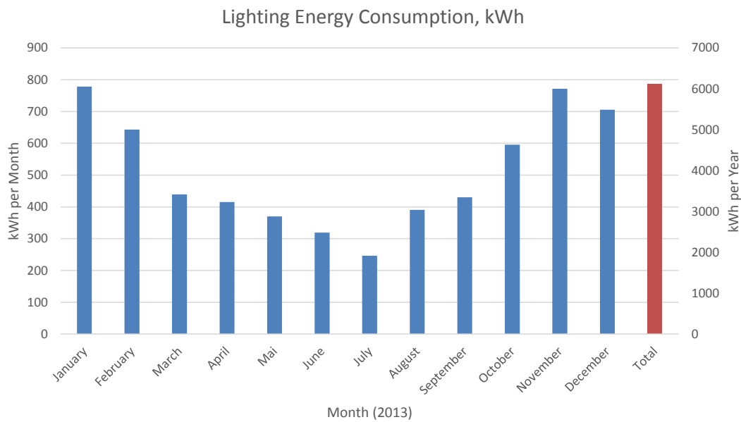
Figure 3. Monthly (blue) and total (red) lighting energy consumption (KNX_EM05_E) in kWh.
