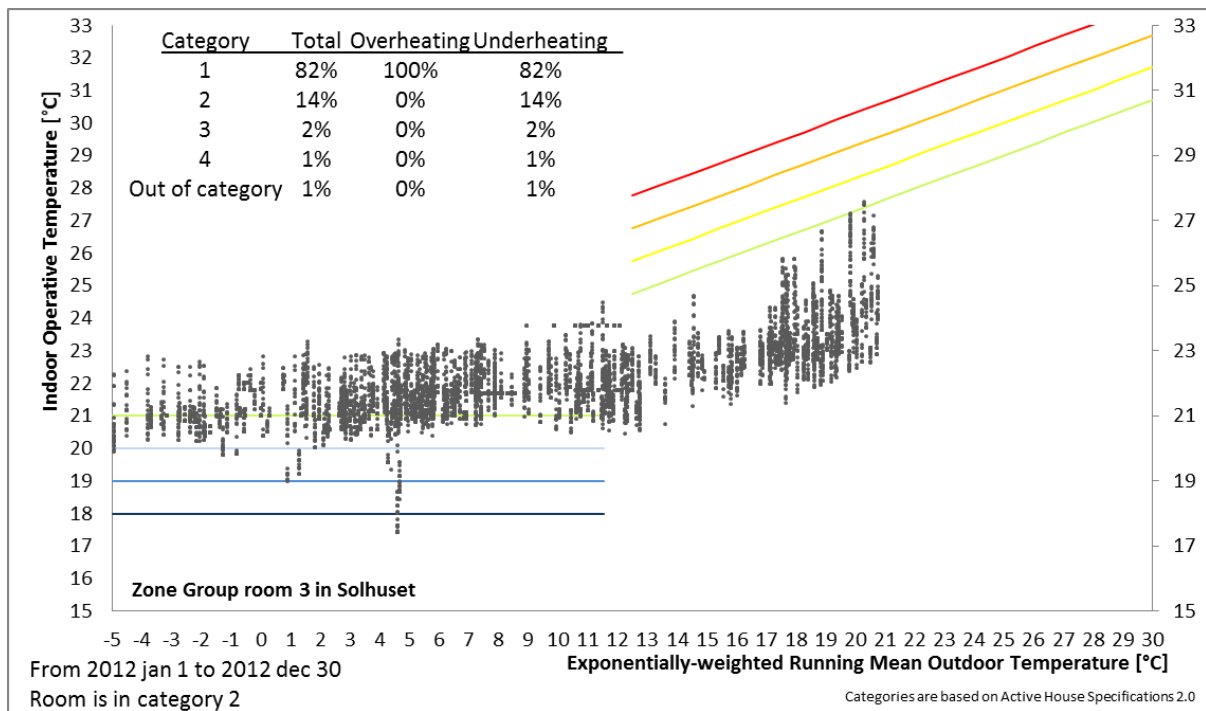
Figure 6. Measured indoor air temperature for Group room 3, plotted against the running mean outdoor temperature. Each dot represent the average temperature for an hour of the year.
