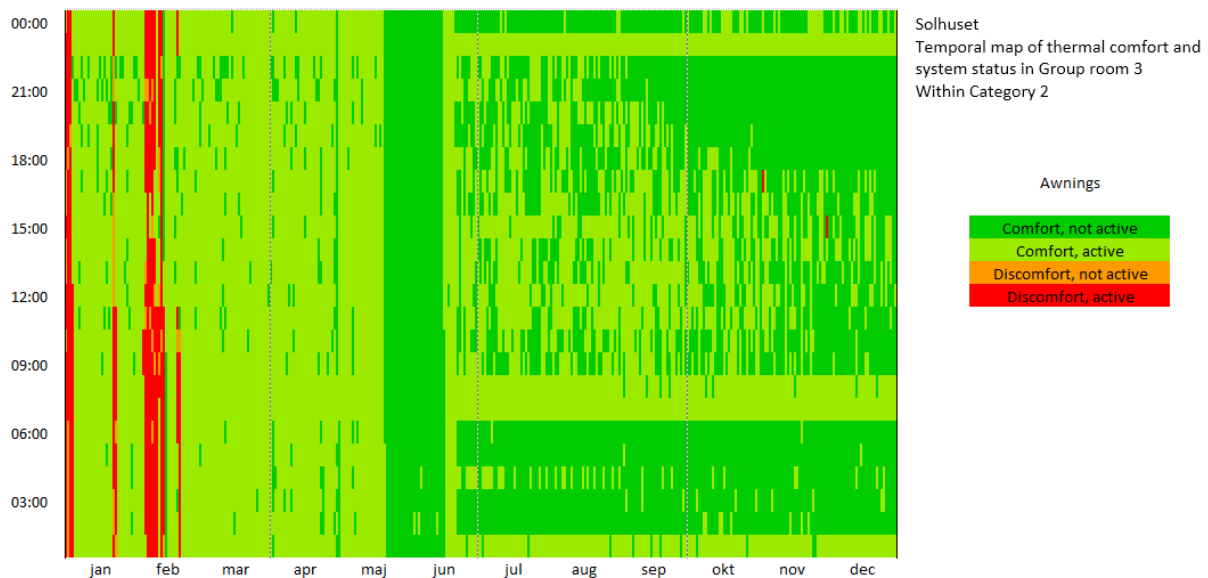
Figure 9 Temporal map for Group room 3 showing active or inactive awnings blinds in combination with thermal comfort category. Awning blinds are marked as active, if one or more awning blinds in the room are open. For the sake of the illustration, category 1 and 2 are called “comfort”, category 3 and 4 are “discomfort”.
