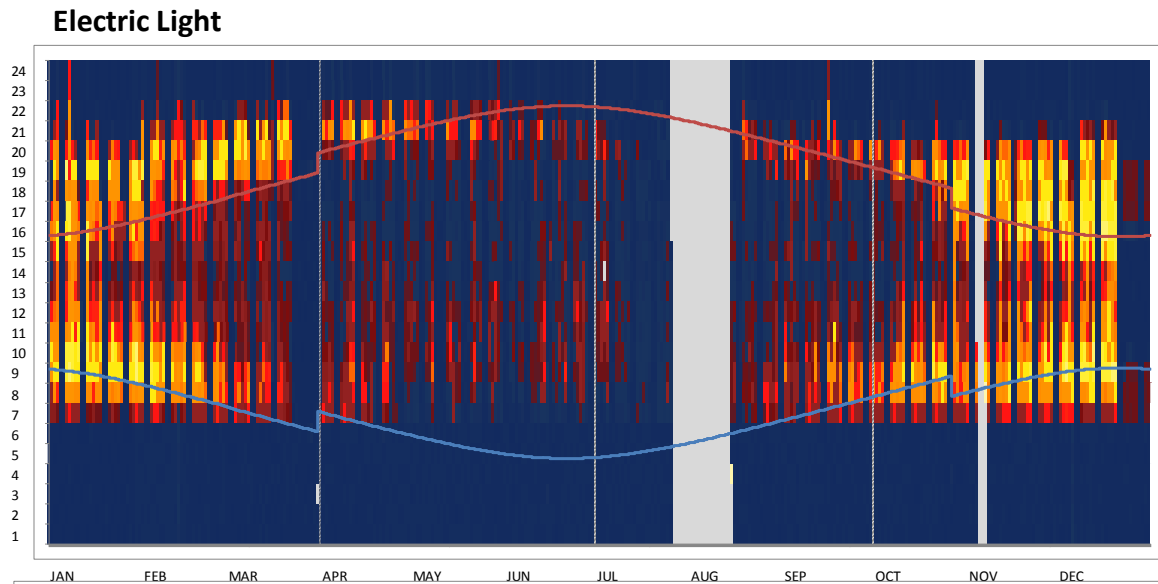
Figure 4. Temporal map of lighting use in Solhuset, 2013, including the sunrise (blue) and sunset (red). Lighting use and sunrise/sunset is according to local time, which account for Daylight Saving Time (DST). Measurements from August is missing.
