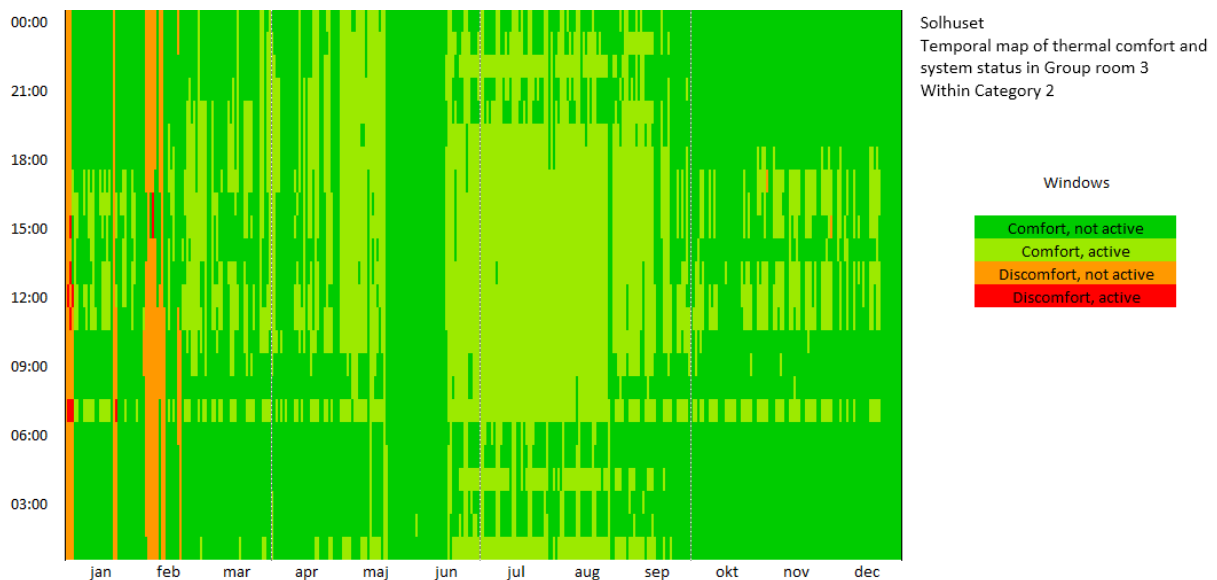
Figure 8 Temporal map for Group room 3 showing open or closed window in combination with thermal comfort category. Windows are marked as open, if one or more windows in the room are open For the sake of the illustration, category 1 and 2 are called “comfort”, category 3 and 4 are “discomfort”.
