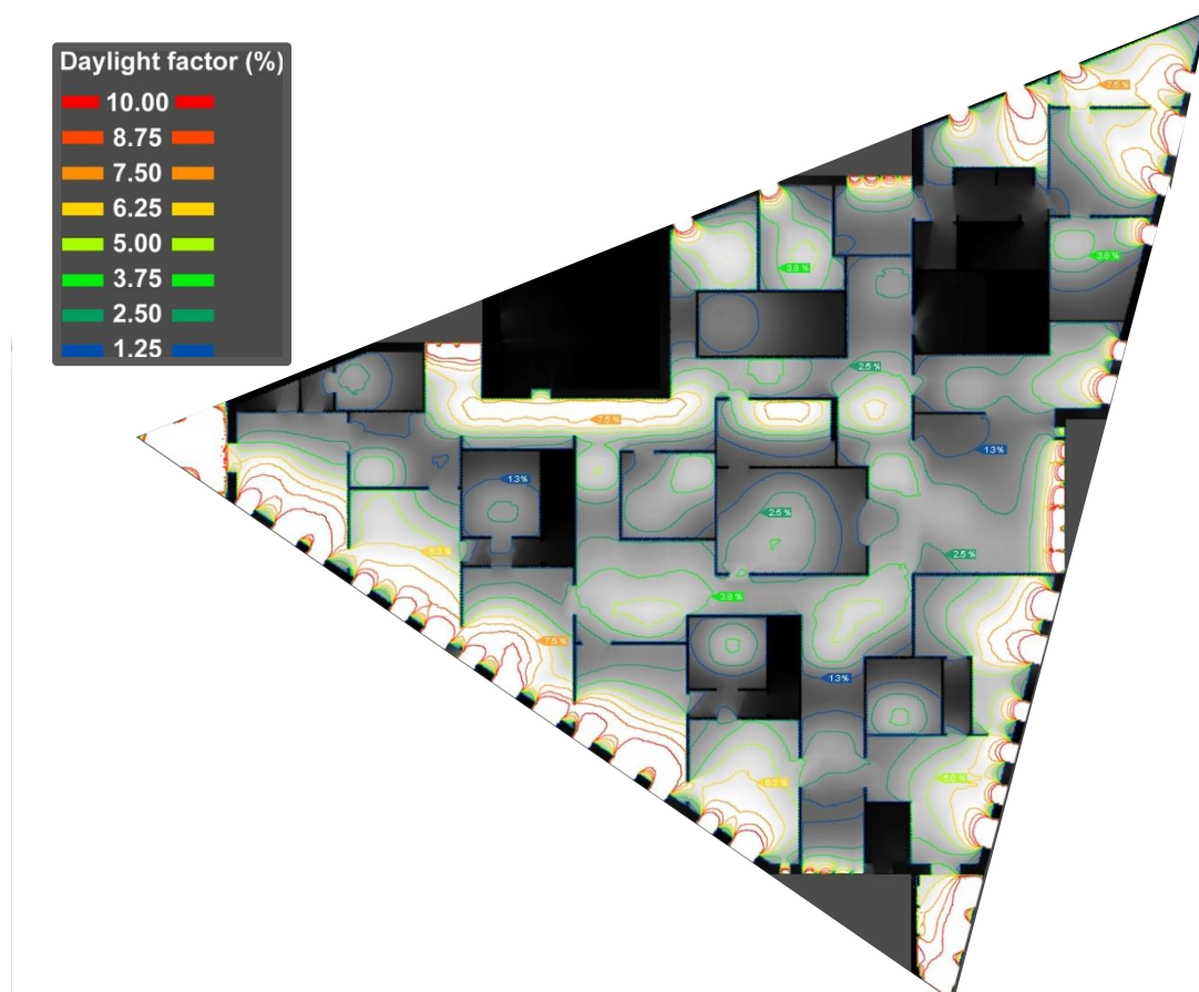
Figure 2. Calculated daylight factors in Solhuset.
