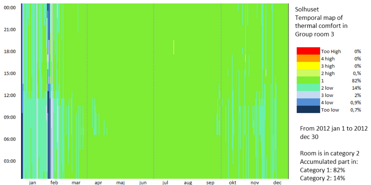
Figure 7. Group room 3. The comfort category of each hour of the year is plotted as a temporal map
