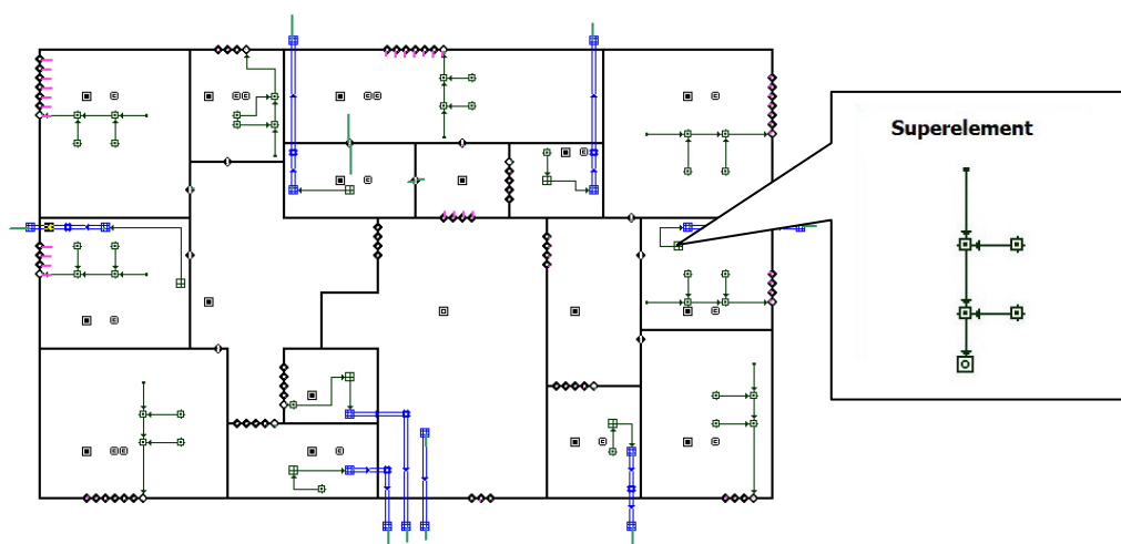
Fig. 3. Sketchpad (CONTAM) presenting 8 floor of analyzed building for analyzed variant.
