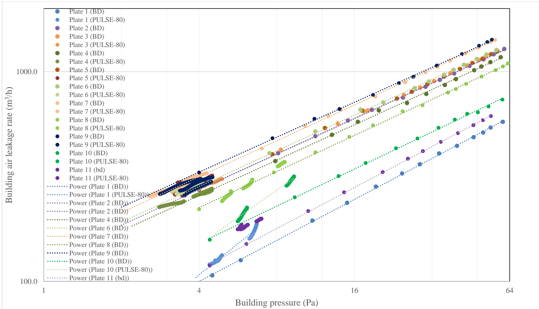
Figure 5 Log-log scale graph of leakage-pressure measured by DBB and PULSE-80
