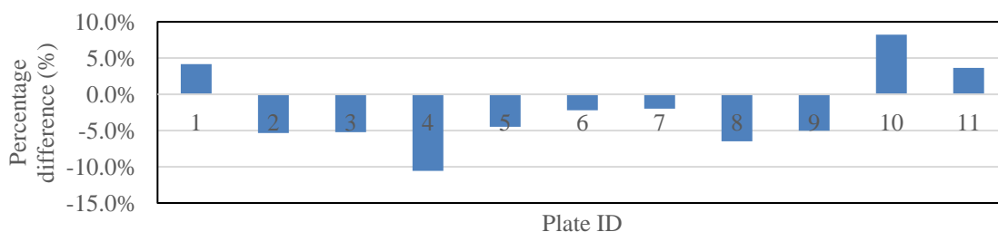
Figure 4 Percentage difference of Q 4 measured by DBB in Standard and Non-standard approach
