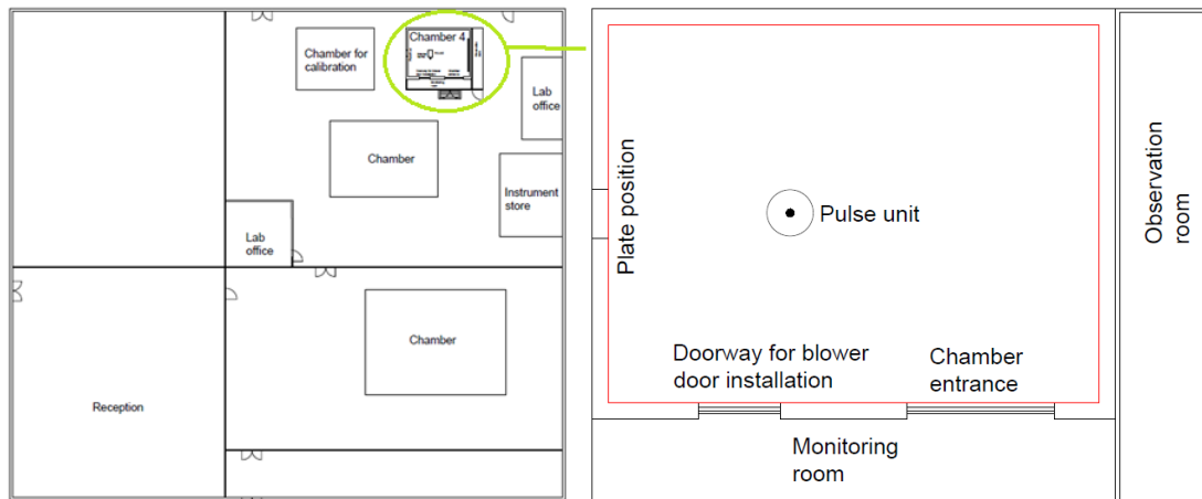
Figure 3 Environmental chamber for testing inside outer building (left) and test enclosure inside the chamber (right)
