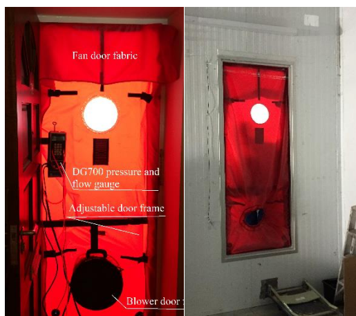
Figure 1 Energy Conservatory Duct blaster B (DBB)
