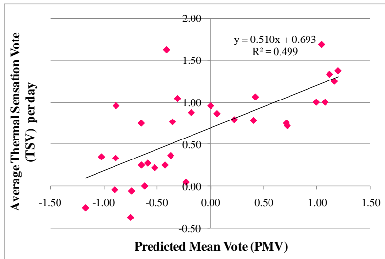
Figure 9: Scatter plot
