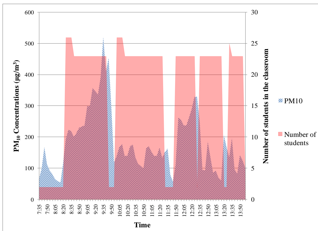
Figure 8: Diurnal variation of PM 10 concentrations in school 4 on April 15 th in relation to the number of students
