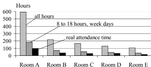
Figure 4: Frequencies for exceeding the maximum allowed room temperature of four passively cooled rooms (B to E) and one air-conditioned room (A) during the summer of 2003 (May 1 st to September 30 th ). The maximum allowed room temperature is 26°C for ambient temperatures up to 32°C, and above that 6 Kelvin below ambient temperature.
