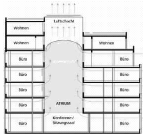
Figure 2: Section of the KfW building and air flow paths during night ventilation.
