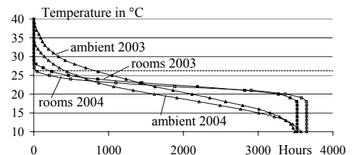
Figure 3: Cumulative frequency distributions for hourly averaged room (air) and ambient temperatures from May 1 st to September 30 th in 2003 and 2004. Due to the type and position of the temperature sensors, indoor air temperatures approximately represent an operative temperature. The room temperature is an average out of 4 office rooms which are exclusively cooled by passive means.
