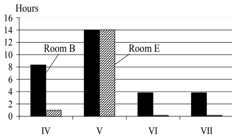
Figure 6: Frequencies of different sensations in room B (east) and E (west) during summer 2003 (May 1 st to September 30 th ) with only considering the hours when the temperature limit was exceeded during the attendance time: (IV) windows opened manually; (V) shading system opened; (VI) window and shading system opened; (VII) shading system closed at least 70% and window opened.
