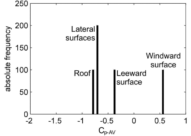
Figure 2: C_{p-AV} histogram for a cube, \theta = 0^\circ .
