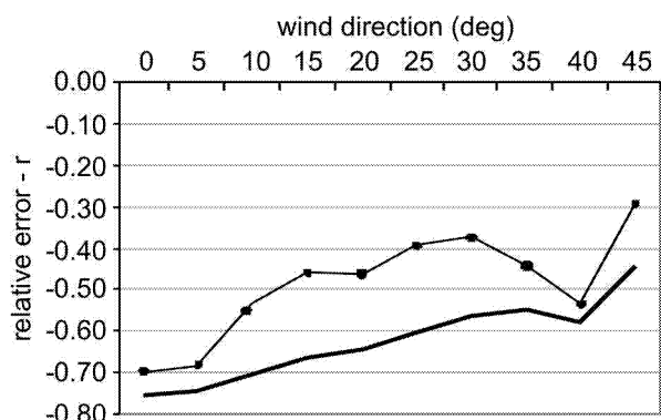
Figure 9: Lower bound values of r , CI = 95\% .
