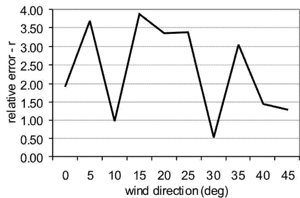
Figure 6: Upper bound values of r , CI = 95\% .
