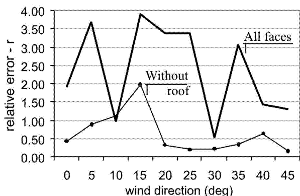
Figure 8: Upper bound values of r , CI = 95\% .
