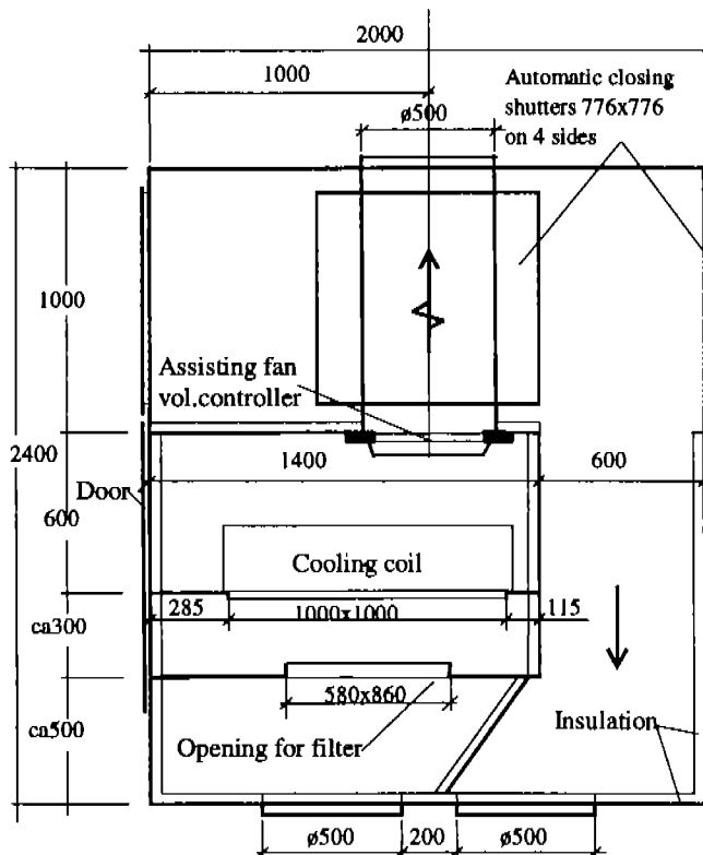
Fig. 2.2. Roof unit
