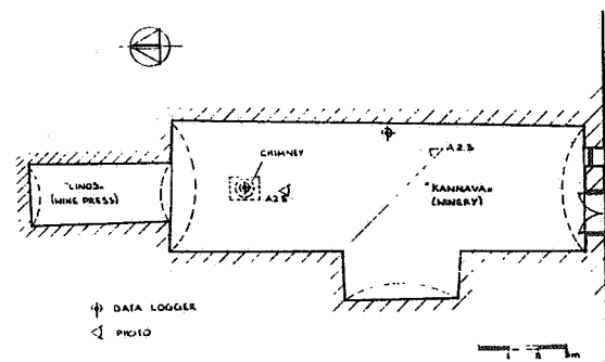
Fig. 2 Building 2: Floor Plan
