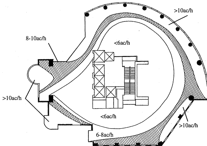
Figure 5: Approximate contours of air flow discharged through the ceiling in building F.
