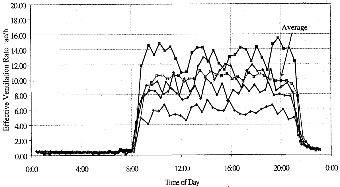
Figure 2: Effective ventilation rates in the breathing zones of building F.
