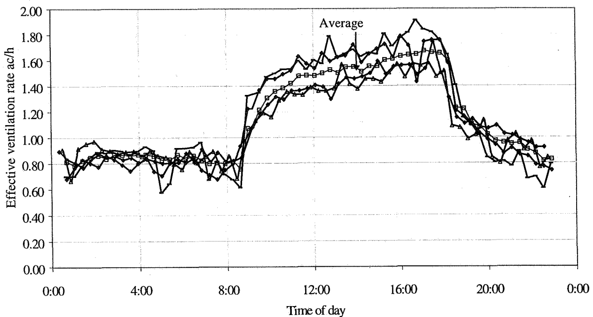
Figure 3: Effective ventilation rates in the breathing zones of building G.
