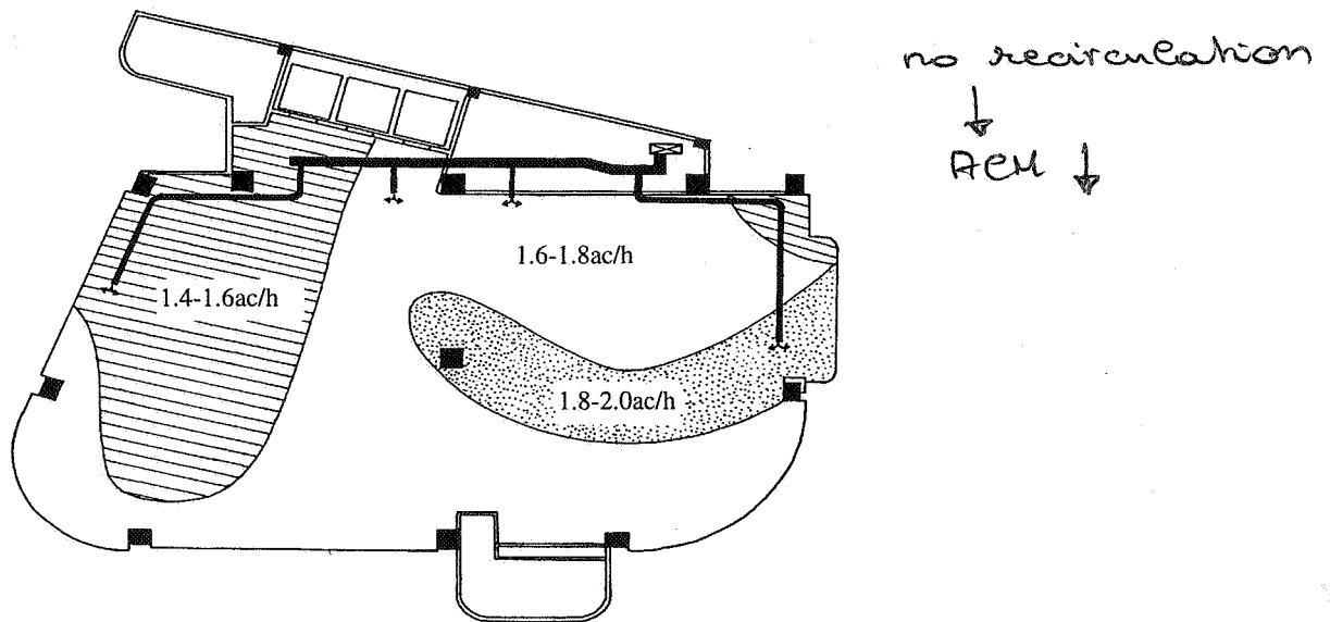
Figure 6: Approximate contours of effective ventilation rate in the breathing zones of building G.
