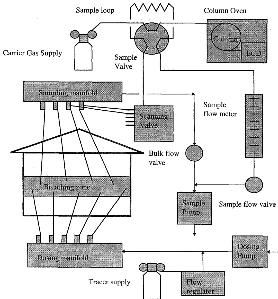
Figure 1: Outline of tracer dosing and sampling equipment for measuring ventilation performance.
