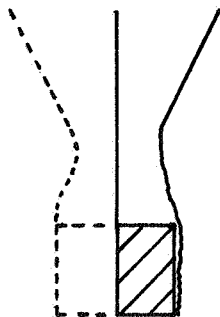
Figure 2. Symmetry considerations regarding vertical volume flux in thermal plumes are illustrated: free plume, two flows forming one plume, wall plume.
