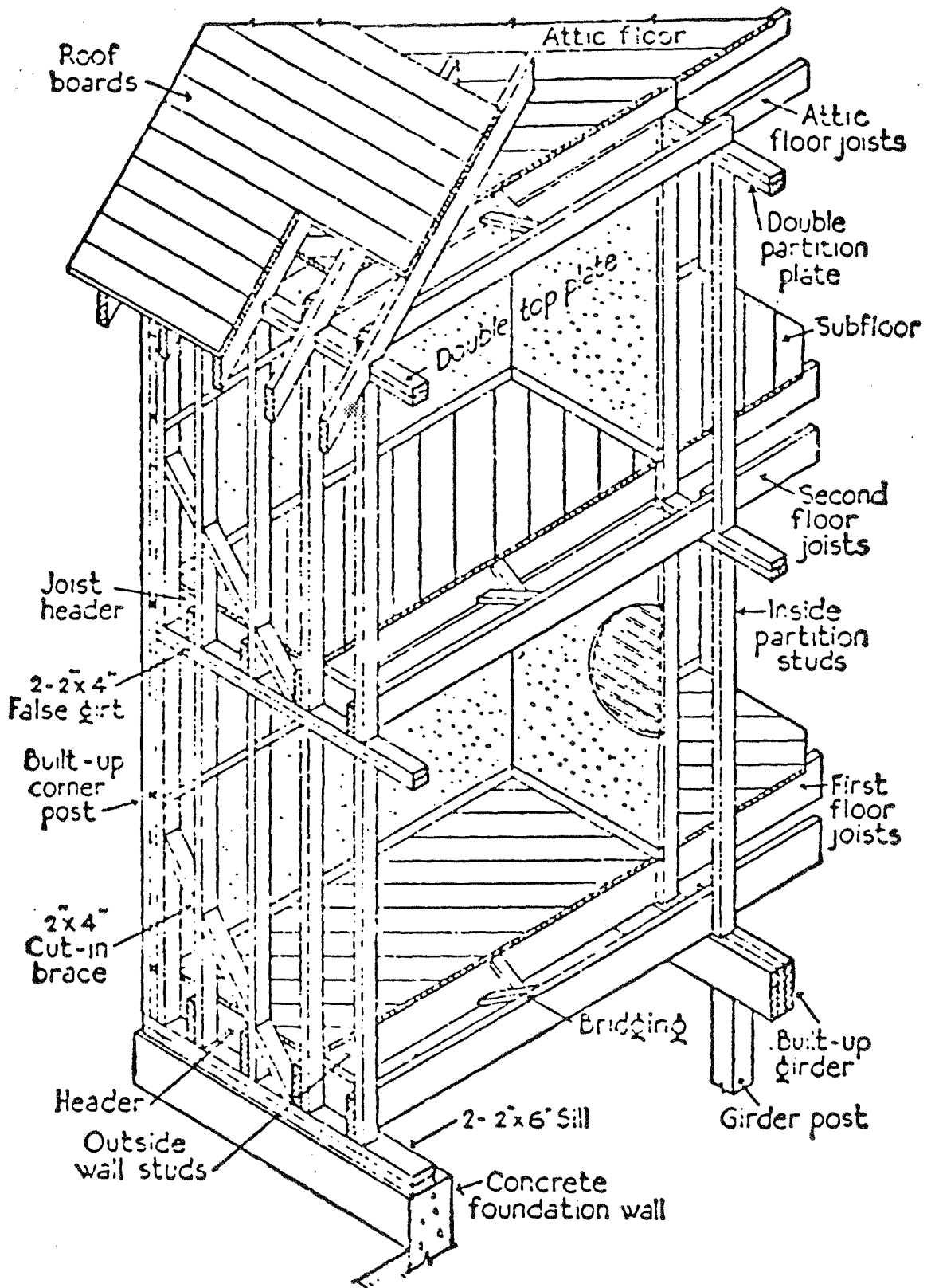
FIGURE 3. BRACED FRAME CONSTRUCTION 12
