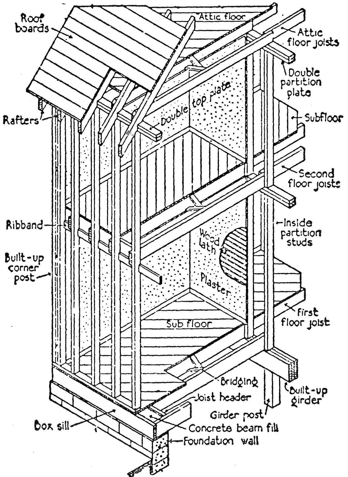
FIGURE 4. BALCONY FRAME CONSTRUCTION
