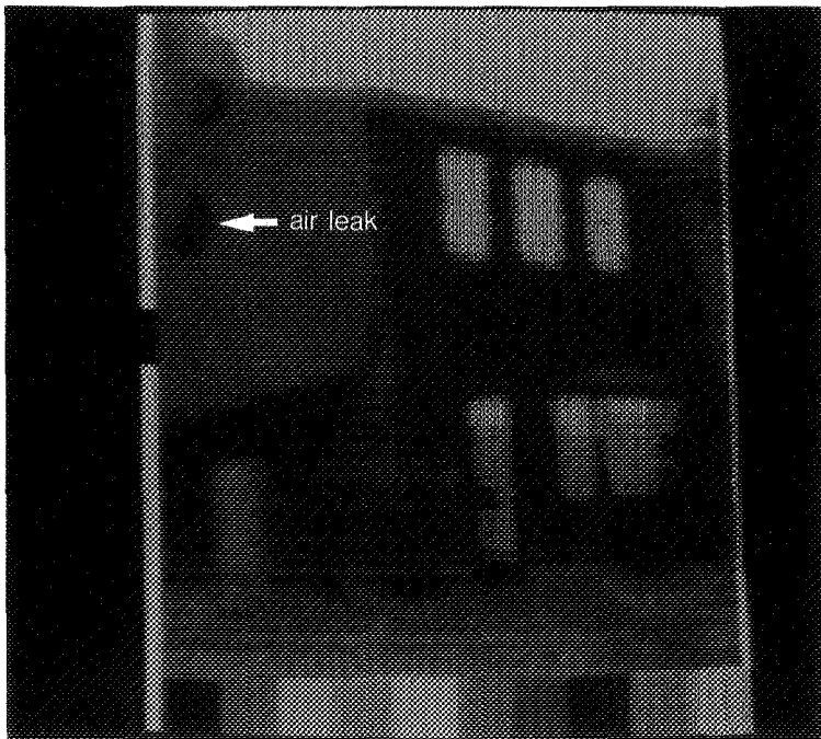
Figure 3b. Exterior thermographic scan while pressurized.
