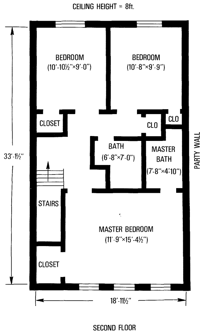
Figure 2. Floor plan of the test house.
