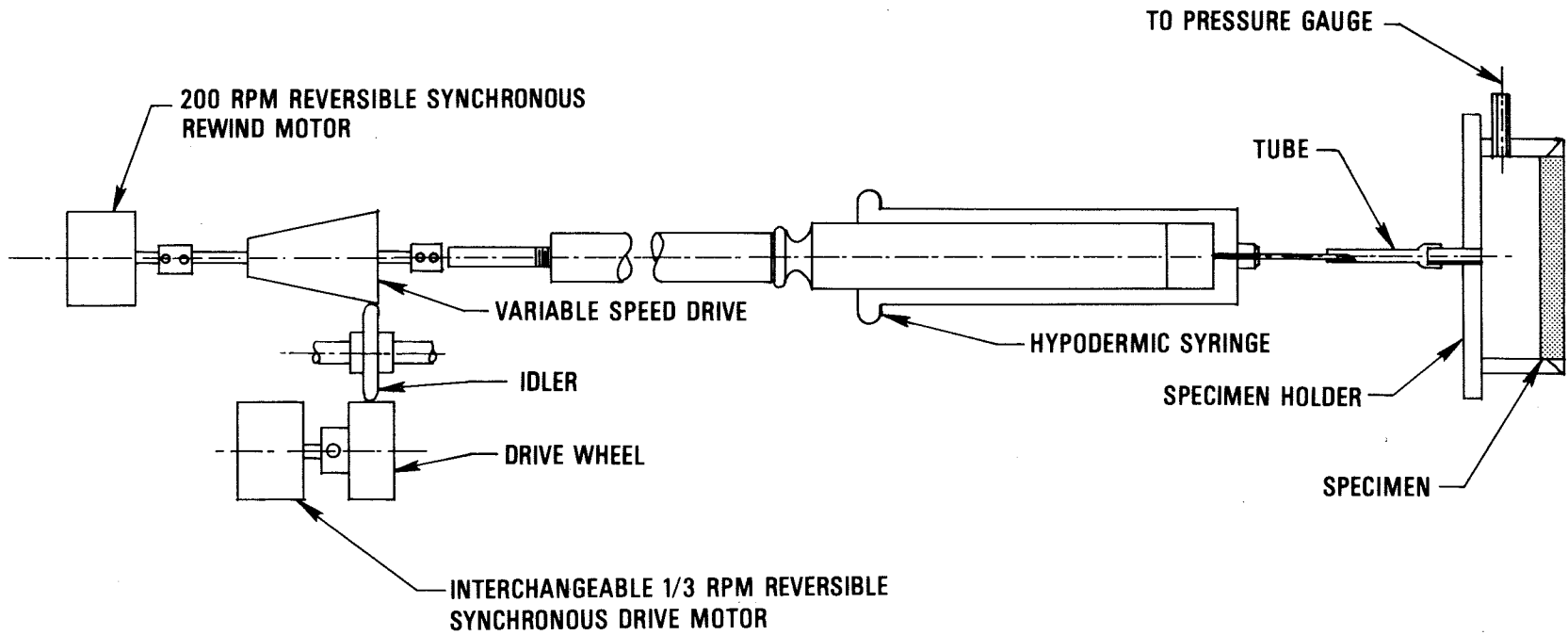
Figure A-1. Apparatus used to measure the air permeability of building materials.
