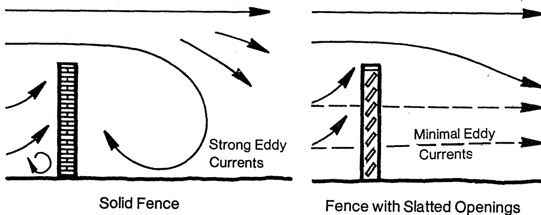
Figure 2. Airflow vs. Fence Design
