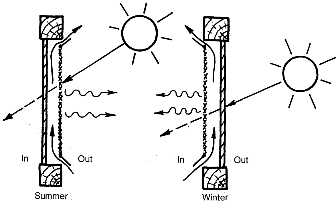
Figure 34. Reversible Sash With Heat-Absorbing Double Glass
