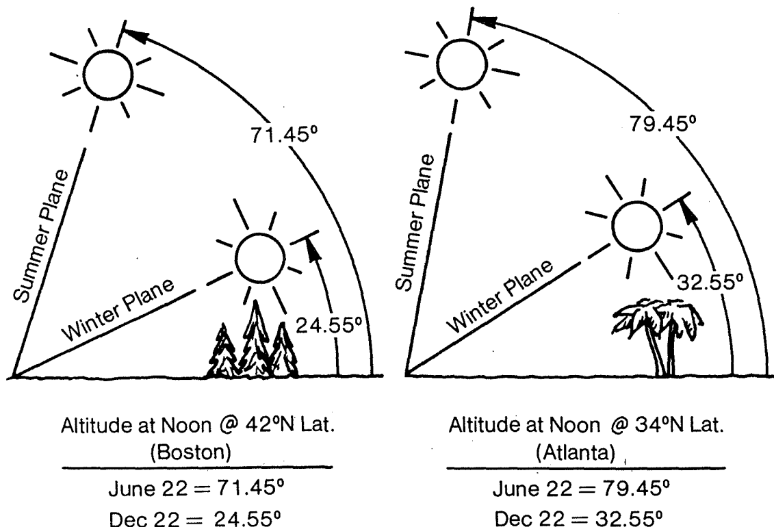
Figure 27. Seasonal Sun Angle Variation For Two Cities
