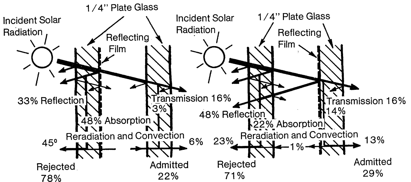
Figure 35. Effect of Film Location on Heat-Gain
