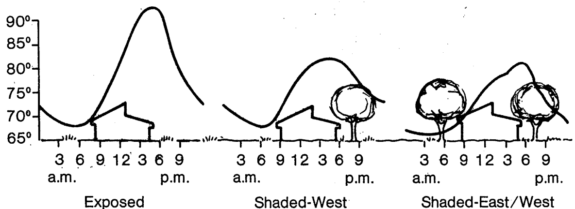
Figure 5. Shade Tree Effectiveness vs. Orientation
