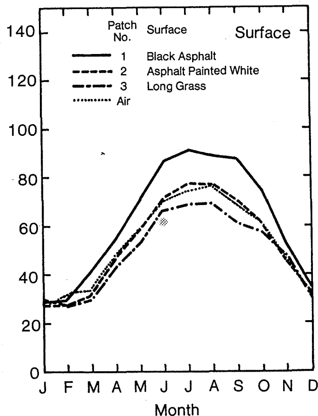
Figure 7. Monthly Ground Surface Temperatures
