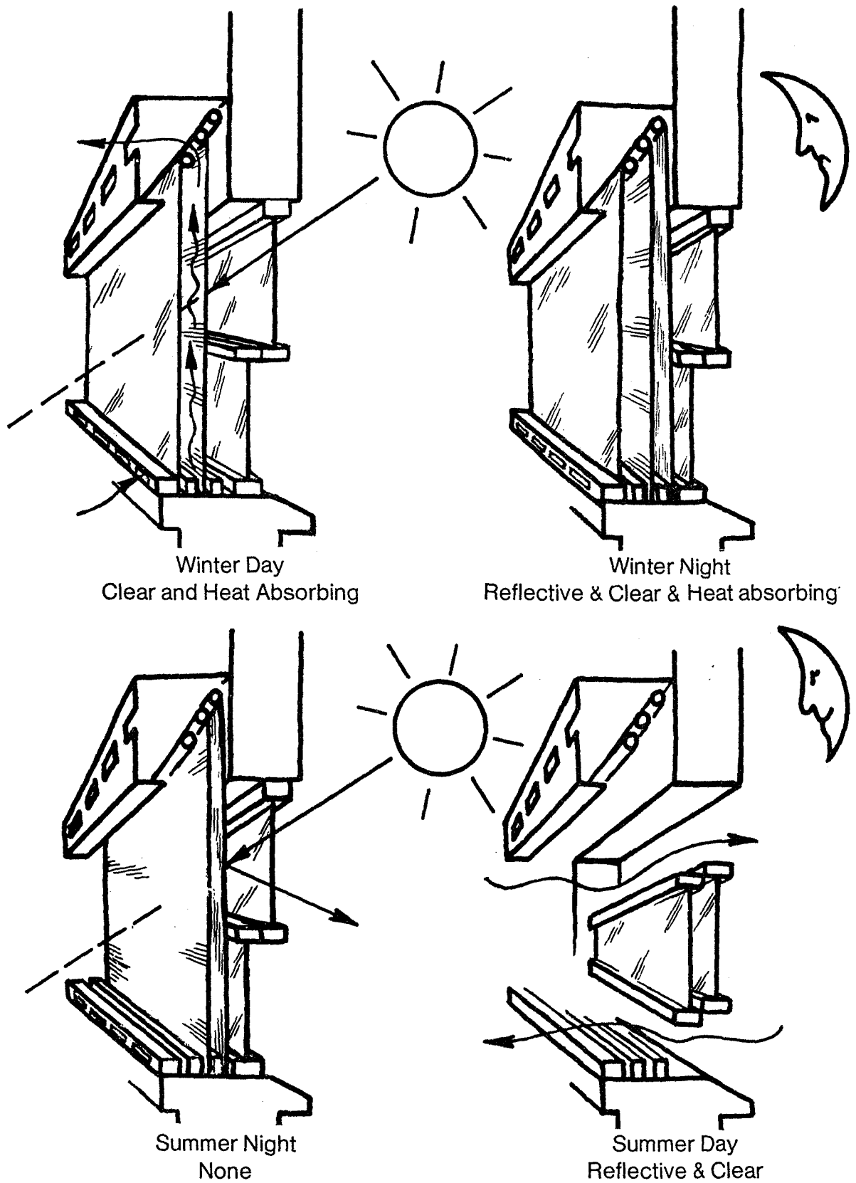
Figure 38. Use Modes of a Multiple Shade System
