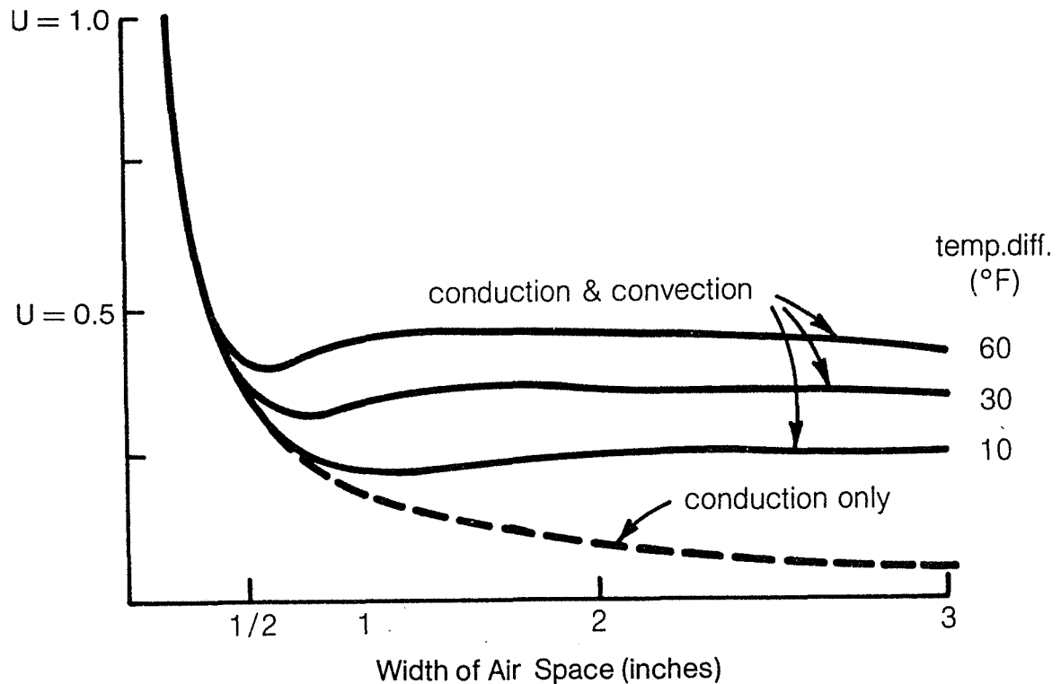
Figure 31. U-Valved Insulation Glass vs. Separation
