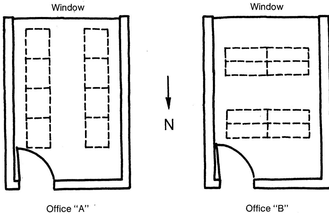
Figure 40. Lighting Fixture Circuiting
