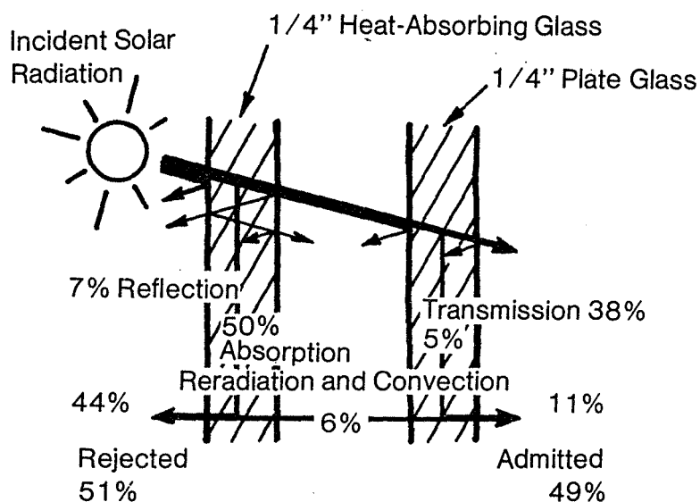
Figure 33. Solar Energy Transmission Heat Absorbing Insulating Glass
