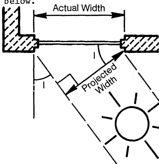
Figure 9. Projected Window Width
