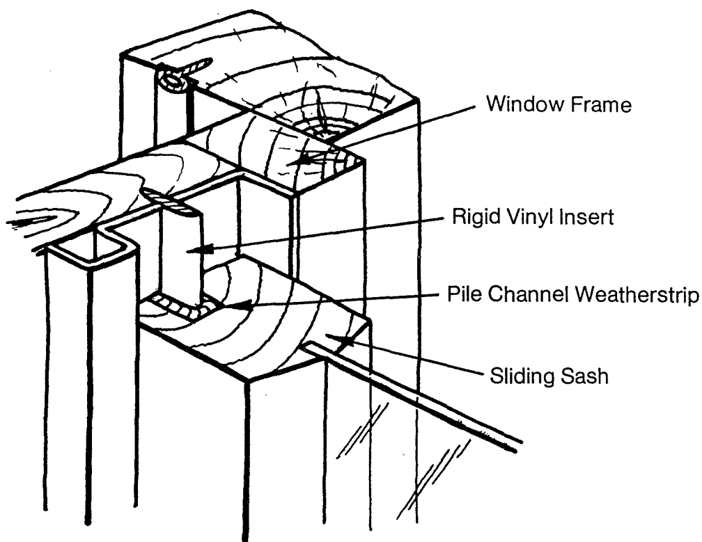
Figure 20. Cut-away Section of a Weatherstripped Window
