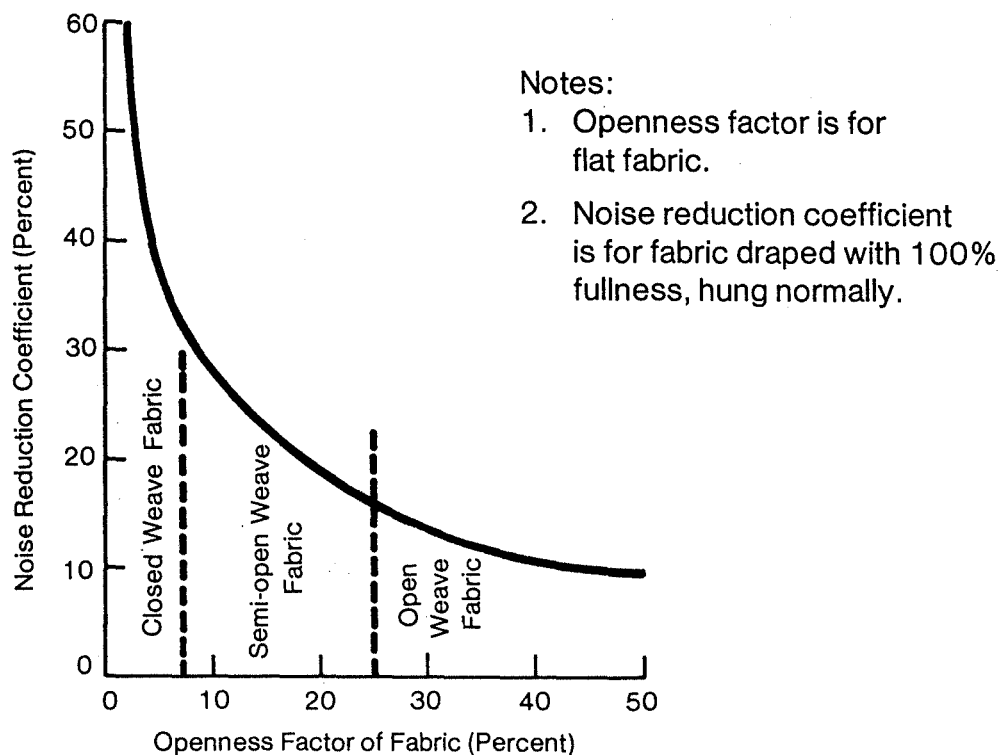
Figure 37 Drapery Type vs. Noise Reduction
