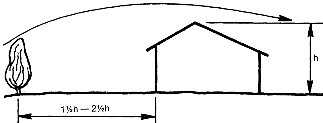
Figure 1. Windbreak Distance
