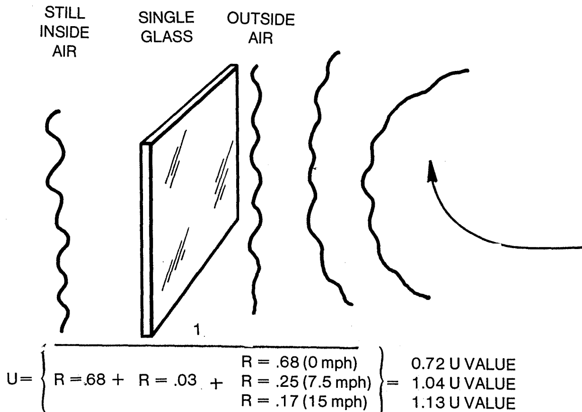
Figure 3. Heat Flow Through Glass vs. Wind Velocity
