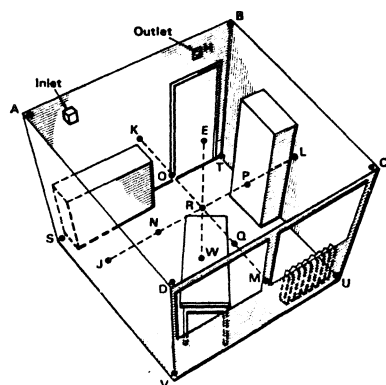
SAMPLING POINTS Each corner and centre of ceiling A, B, C, D, E. Against outlet - - - H. Centre of each wall - - - J, K, L, M. Centre of room - - - N, O, P, Q, R. Each corner and centre of floor - S, T, U, V, W. Each letter indicates the position of one of the 2mm internal diameter tubes used for extracting carbon dioxide samples. The carbon dioxide supply system is shown in fig.10
