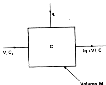
Fig. 7. Gas of concentration c_0 entering a room of volume M at a rate V with fresh air ventilation q .
