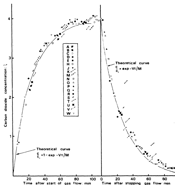
Fig. 11. Variation of carbon dioxide concentration with time at positions shown in Figure 9. Ventilation rate 2½ RV/H.
