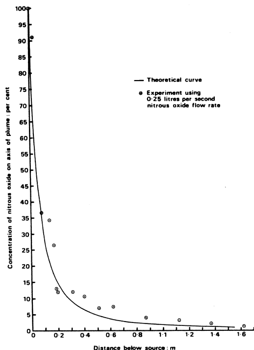
Fig. 23. A comparison of theory and experiment using nitrous oxide for buoyant plumes.
