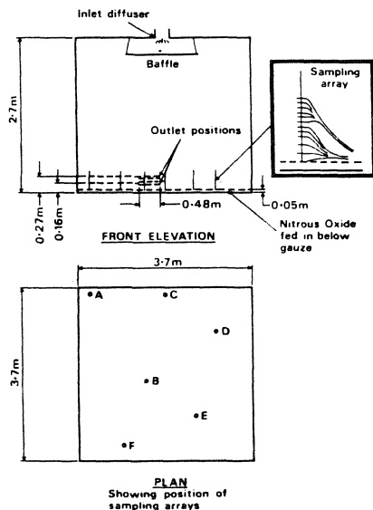
Fig. 15. Room for layering experiments.
