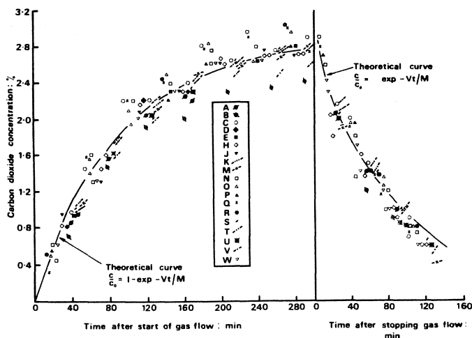
Fig. 12. Variation of carbon dioxide concentration with time at positions shown in Figure 9.
