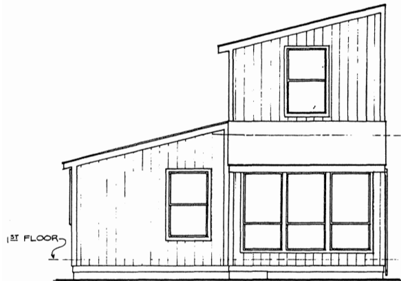
FIGURE 5. Front elevation of test house.
