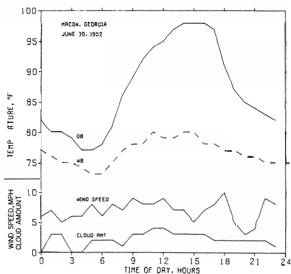
FIGURE 26. Weather data for Macon, Georgia, June 30, 1952.
