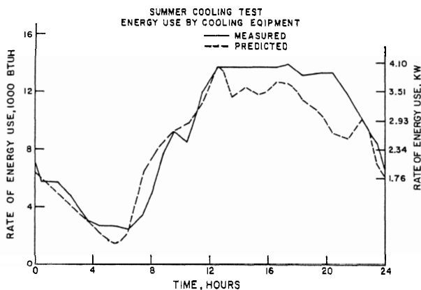
FIGURE 54. Energy consumed by air cooling equipment for test 9.
