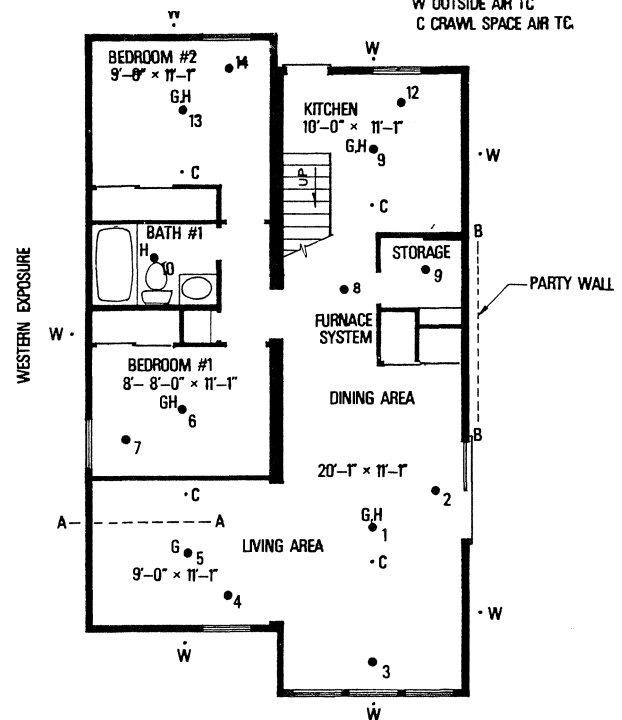
FIGURE 3. First floor plan of test house.
