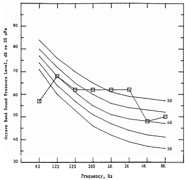
FIGURE B-5. The symbols show the octave band sound pressure levels in the kitchen with the heating system operating.
