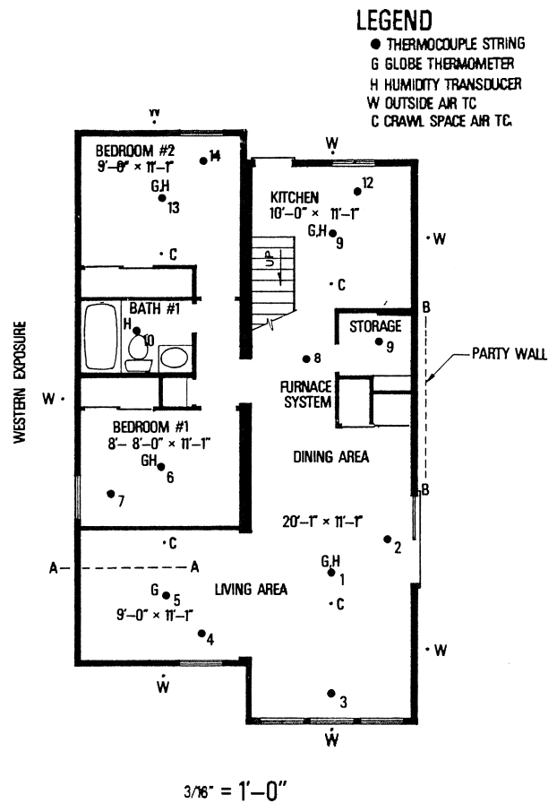
FIGURE 3. First floor plan of test house.
