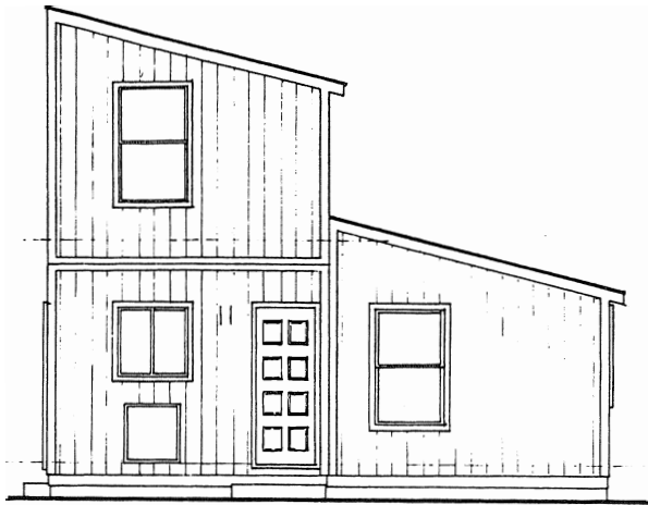
FIGURE 7. Rear elevation of test house.
