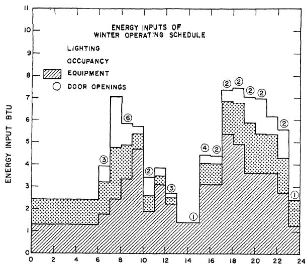
FIGURE 34. Energy inputs for simulated winter operating schedule.
