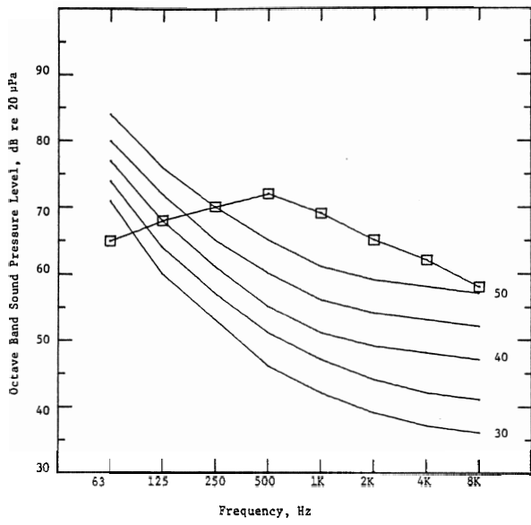
FIGURE B-7. The symbols show the octave band sound pressure levels in the kitchen with the exhaust fan operating. The numbered curves are "noise criteria curves."
