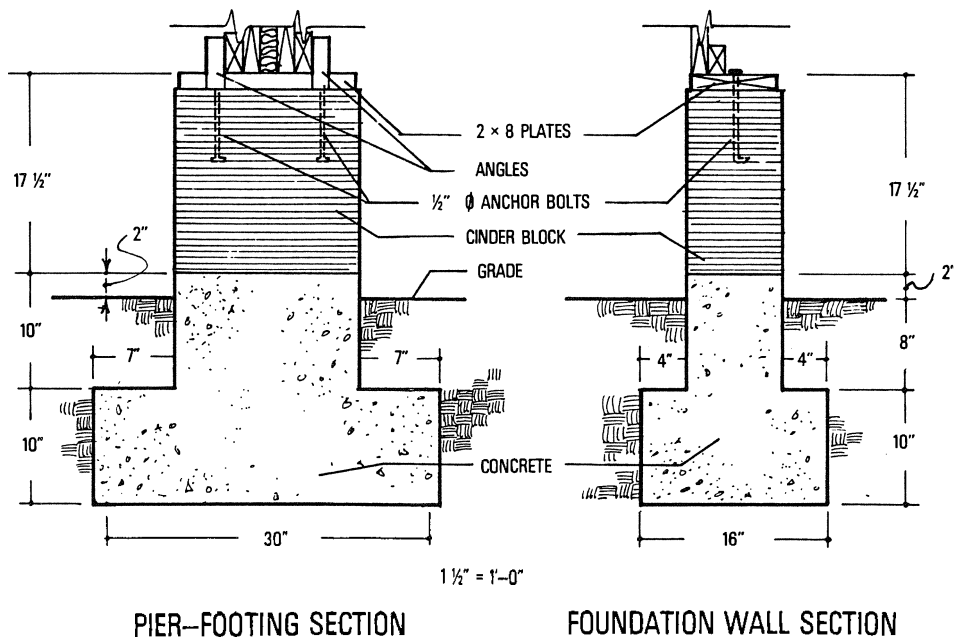
FIGURE 15. Detail sections of foundation pier and footings.
