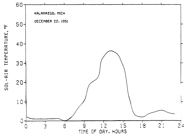
FIGURE 32. Area averaged sol-air temperature for Kalamazoo, Michigan, December 22, 1951.
