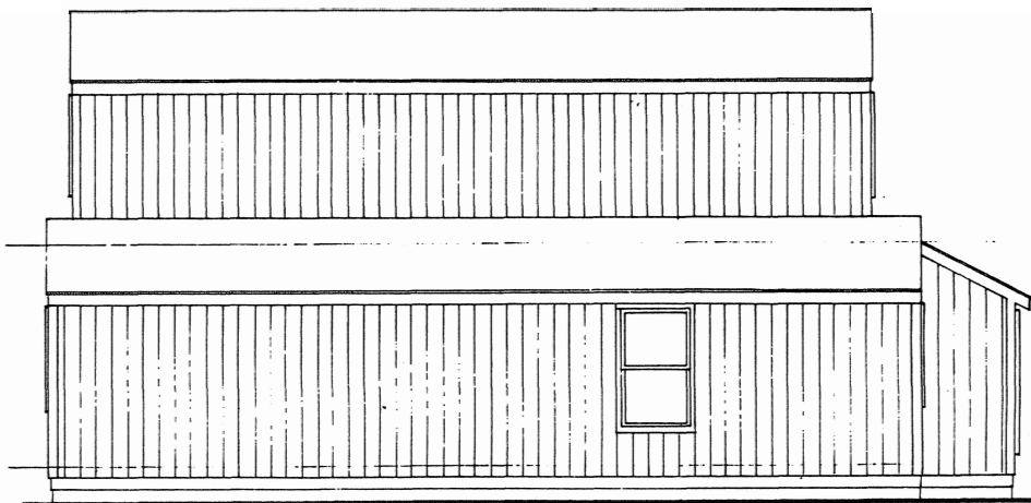
FIGURE 6. Side elevation of test house.
