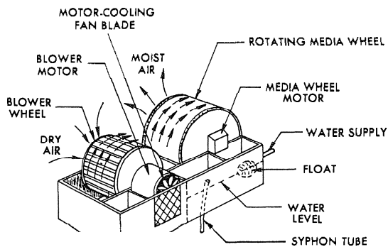
FIGURE 17. Wetted drum type humidifier.
