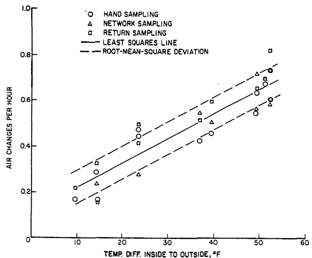
FIGURE A-1. Air exchange rate as a function of difference in temperature between inside and outside of townhouse.
