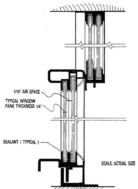
FIGURE 14. Typical window detail showing storm sash installed.
