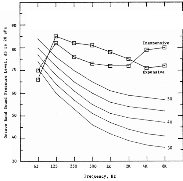
FIGURE B-8. The symbols show the octave band sound pressure levels in the kitchen with two different garbage disposers operating. The numbered curves are "noise criteria curves."
