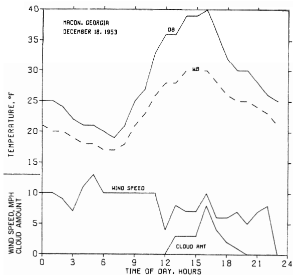
FIGURE 23. Weather data for Macon, Georgia, December 18, 1953.
