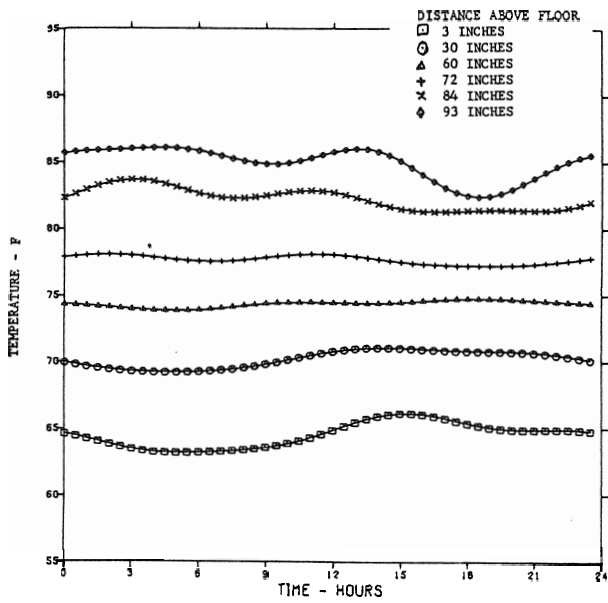
FIGURE 63d. (Bedroom 1).
