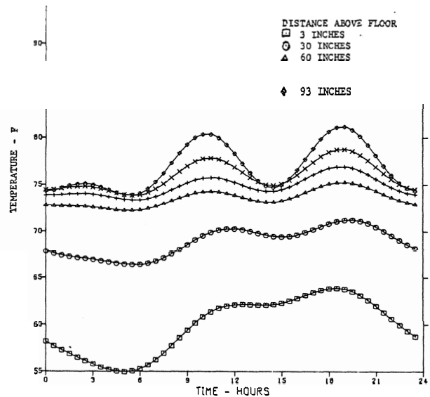
FIGURE 63c. (Kitchen).
