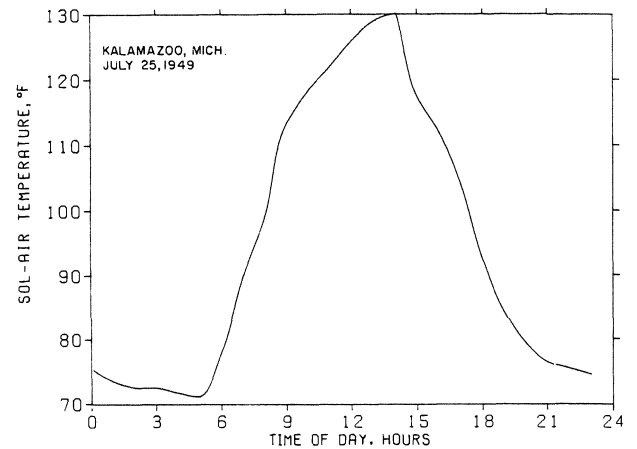
FIGURE 33. Area averaged sol-air temperature, Kalamazoo, Michigan, July 25, 1949.
