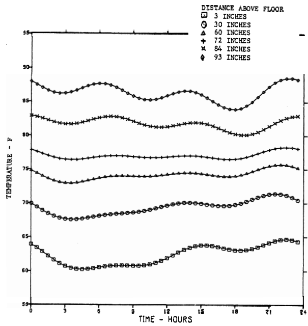
FIGURE 63f. (Bathroom 1).
