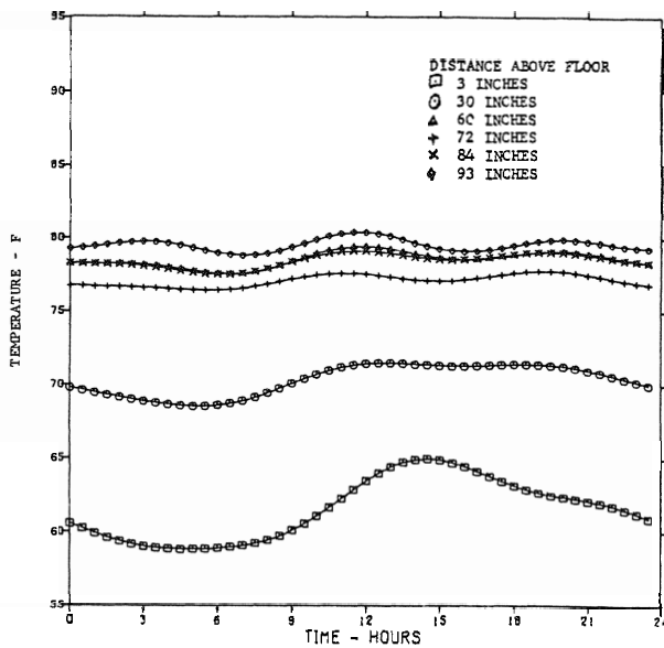
FIGURE 63a. Downstairs temperatures at various levels for test 1 (living room).
