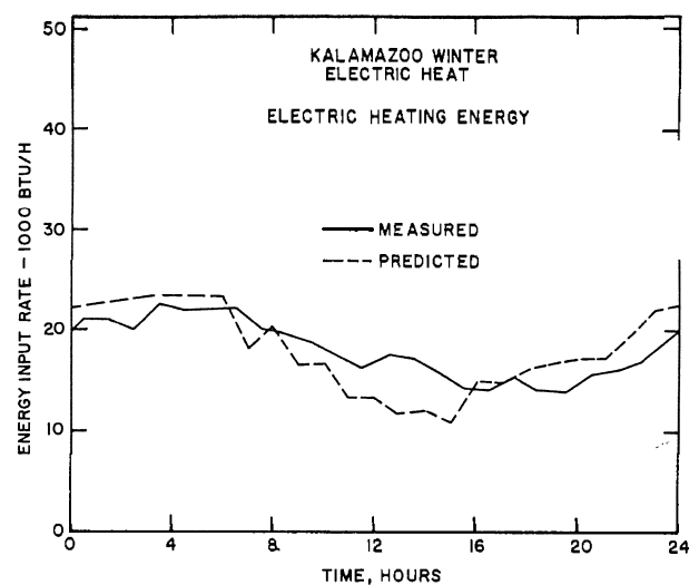
FIGURE 39. A comparison between the measured and calculated rates of energy input to the furnace system for test 1.
