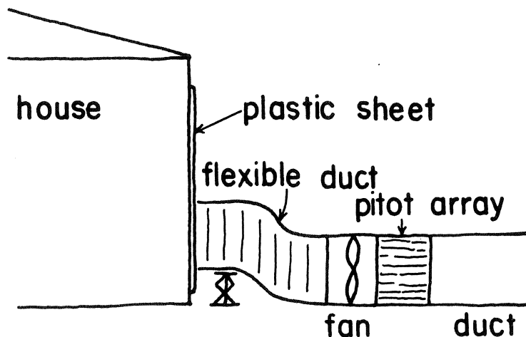
Figure 2. A sketch of the blower door assembly.
